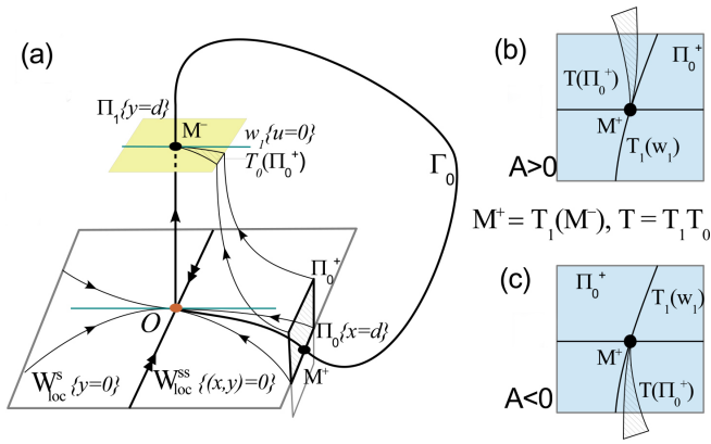
FIG. 3. (a) Example of a homoclinic loop \Gamma_0 to a saddle O with real eigenvalues \lambda_{ss} < \lambda_s < 0 < \lambda_u in 3-dimensional phase space. If the saddle value \sigma = \lambda_u + \lambda_s < 0 , a stable periodic orbit is born from such loop, see Fig. 1. When \sigma is positive, then additional conditions are needed for a single saddle periodic orbit to be born. In some local coordinates (x, y, u) near O the unstable and stable manifolds are the y -axis and the (x, u) -plane; the leading eigen-direction is the x -axis, and the eigen-direction corresponding to the non-leading eigenvalue \lambda^{ss} is the u -axis. We require that the separatrix \Gamma_0 does not lie in the strong-stable manifold W^{ss} . Hence, \Gamma_0 enters O as t \rightarrow +\infty along the x -axis. In order to see that the separatrix value A does not vanish, we build two cross-sections to the homoclinic loop: \Pi_0 across the local stable manifold W_{loc}^s and \Pi_1 across the local unstable manifold. Orbits starting on \Pi_0 pass near O and hit \Pi_1 at the points of a thin wedge tangent to the x -axis; the flow along \Gamma_0 returns this wedge to \Pi_0 . The condition A \neq 0 means that the image wedge on \Pi_0 is not tangent to W_{loc}^s , as shown in panels (b,c) that represent the cases of the orientable (b) and non-orientable (c) homoclinic loop.
