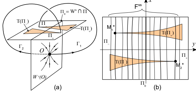
FIG. 15. (a) Return map T generated by trajectories of the Afraimovich-Bykov-Shilnikov geometric model. The map T has a discontinuity line associated with the stable manifold of the saddle equilibrium O . It maps the cross-section \Pi into a pair of triangles. (b) The strong-stable invariant foliation on \Pi due to horizontal expansion and vertical contraction.
