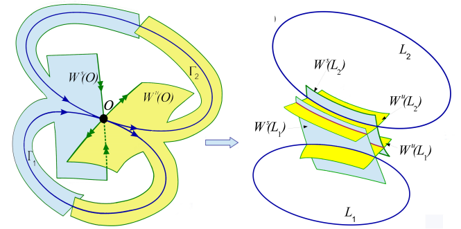
FIG. 5. As a saddle-saddle O with two homoclinic loops \Gamma_1 and \Gamma_2 disappears, the stable and unstable manifolds of the saddle cycles L_1 and L_2 intersect transversely, which causes the onset of a hyperbolic set by virtue of Shilnikov theorem 13 , see Section III.
