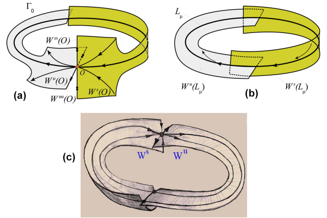
FIG. 4. (a) A saddle-saddle equilibrium O in 3-dimensional phase space with a single homoclinic orbit \Gamma_0 , along which the 2-dimensional stable and unstable invariant manifolds W^s(O) and W^u(O) intersect transversely. (b) Once the saddle-saddle vanishes, the homoclinic transitions to a single saddle periodic orbit L_\mu . (c) A saddle-saddle can have several transverse homoclinic orbits; from Ref. [12].
