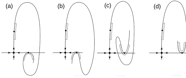
FIG. 9. Various types of homoclinic tangencies in 2D diffeomorphisms.
