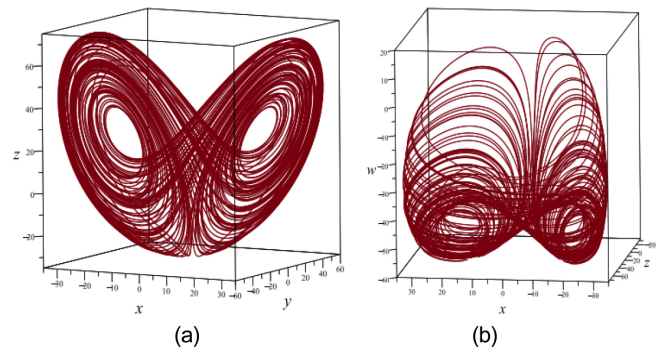
FIG. 17. (a) (x,y,z) -phase space and (b) the (x,z,w) -phase space projections of the strange attractor in the following 4D Lorenz-like system \{\dot{x} = \sigma(y-x), \dot{y} = x(r-z) - y, \dot{z} = xy - bz + \mu y, \dot{w} = -bw - \mu z\} at \sigma = 10, b = 8/3, r = 25 and \mu = 7 ; from Ref. 142
