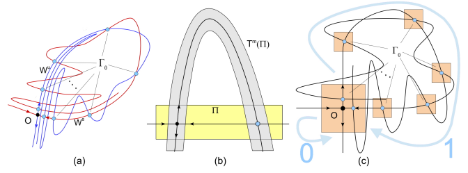
FIG. 8. (a) Poincaré homoclinic tangles. (b) Smale horseshoe due to a transverse homoclinic intersection. (c) The Shilnikov method allows to account for all orbits in a small neighborhood (the orange boxes) of the transverse homoclinic orbit \Gamma_0 . Each of these orbits is uniquely coded by a sequence of 0s and 1s: the symbol “0” corresponds to an iteration in a small neighborhood of the periodic orbit and “1” corresponds to an excursion along the homoclinic.
