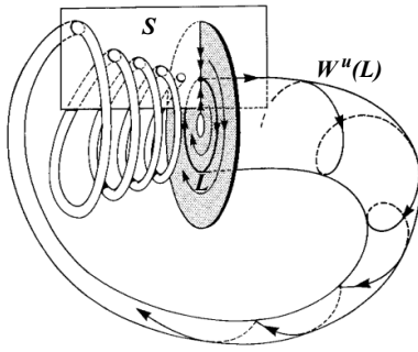
FIG. 13. Illustration to the mechanism of the blue-sky catastrophe, from Ref. 32 . The squeezing unstable manifold W^u(L) returns to the saddle-node periodic orbit L from its node region so that the circles of its intersection with the cross-section S shrink more and more with each subsequent iteration.
