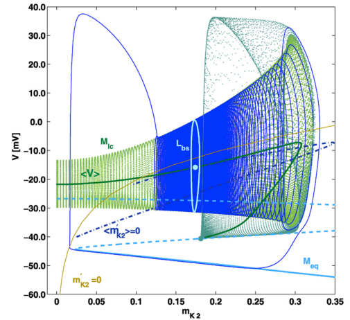
FIG. 14. Shown in the dark blue color is the long bursting orbit transitioning from spiking activity through blue sky catastrophe in the 3D phase space of the neural model as soon as the saddle-node limit cycle (in light blue) vanishes in the slow-motion manifold M_{LC} ; from Refs. 103,104 .
