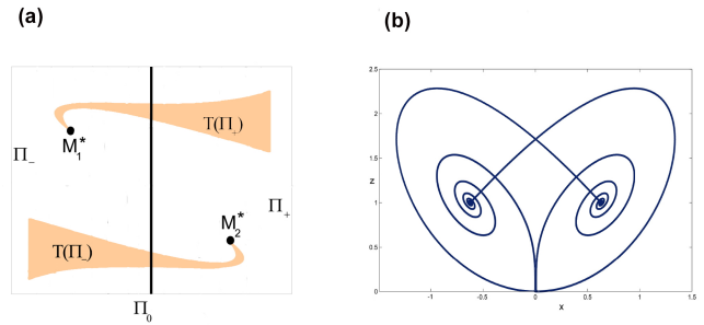
FIG. 16. (a) The “hooks” at the tips of T(\Pi_+) and T(\Pi_-) lead to homoclinic tangencies and, hence, to stable periodic orbits. (b) The heteroclinic cycle connecting a saddle and two symmetric saddle-foci (in the Shimizu-Morioka model 126 ).
