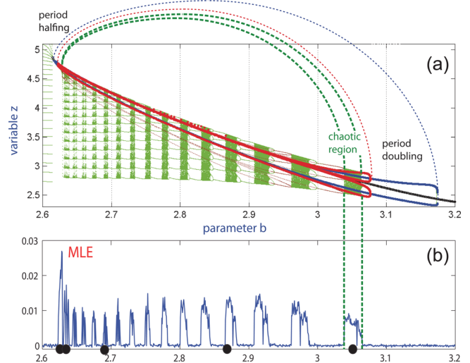
FIG. 7. (a) Sweeping diagram, showing the PSS z -variable plotted against the b -parameter of the HR model along the (brown) straight-line ( I = (1 - 0.265 b)/0.0691 ) transversally passing throughout the chain of the chaotic regions in Fig. 4. Shown in green are chaotic attractors; other colors denote stable/unstable periodic orbits. (b) Ups and downs of the maximum Lyapunov exponent (MLE) of the attractors plotted against the b -parameter reveal alternation of chaotic and stability regions. Black dots locate specific parameter values in the text and in Figures 8 and 9.
