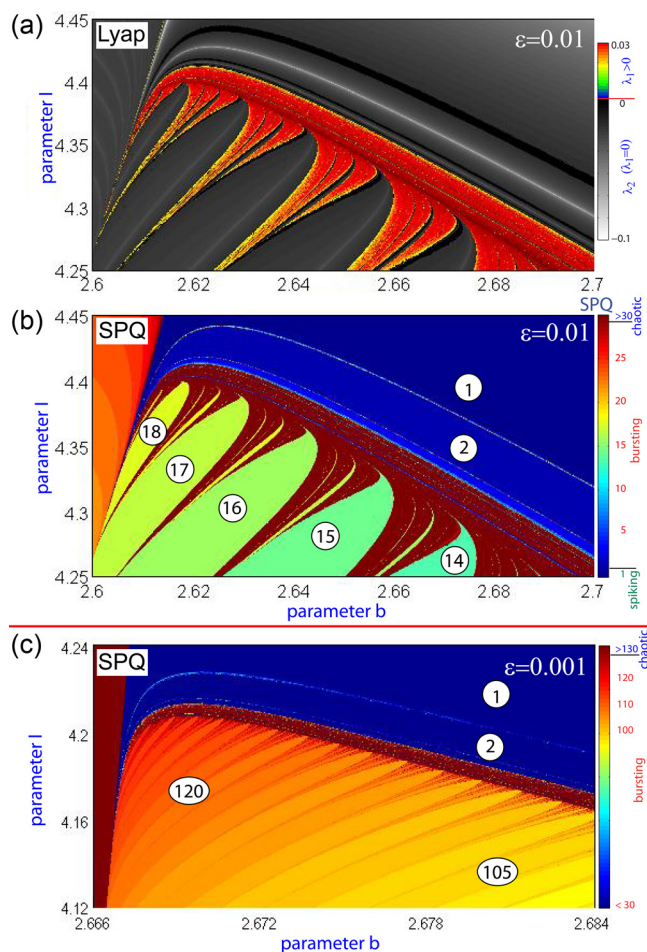
FIG. 3. Magnifications of the upper-left (boxed) fragments of the diagrams in Fig. 2. Panel (a) shows the 1st and 2nd Lyapunov exponents in the color and gray scales, respectively, for \varepsilon = 0.01 . Panel (b) shows the SPQ sweep of the same region. Panel (c) shows the spike-quantification sweep for \varepsilon = 0.001 . Circled numbers depict spike numbers per bursts in the chosen locations.
