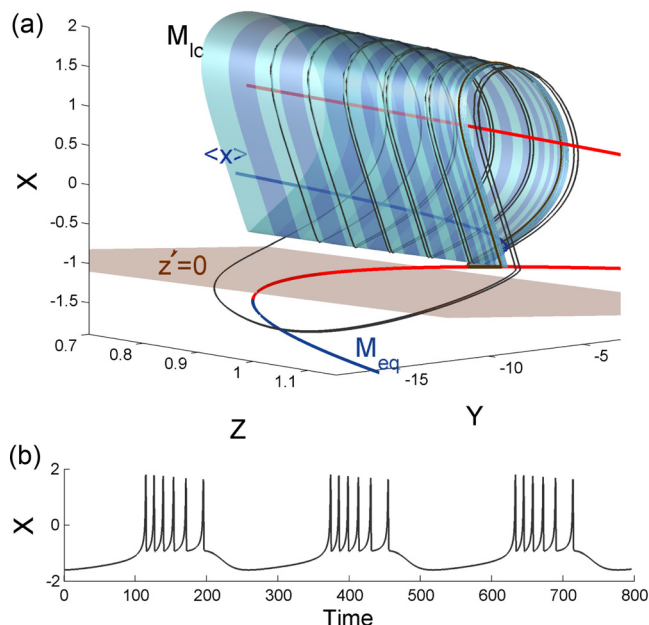
FIG. 1. (a) Bursting orbit in the 3D phase space of the HR model ( x_0 = -1.3 , b = 3 , I = 5 , and \varepsilon = 0.002 ) with two slow motion manifolds: 2D tonic spiking M_{\text{lc}} and 1D quiescent M_{\text{eq}} . Plane, z' = 0 , is a slow nullcline. The number of turns of the bursting orbit around M_{\text{lc}} is that of spikes per bursts in the voltage trace (b).
