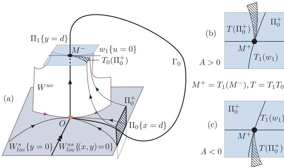
Fig. 4. (a) The local map T_0 takes the upper part \Pi_0^+ of the cross-section \Pi_0 into a curvilinear triangle on the cross-section \Pi_1 . The points in \Pi_0 \cap W^s_{loc} are mapped to a single point M^- . (b) The image of \Pi_0^+ by the Poincaré map T in the case A > 0 . (c) The case A < 0 .
