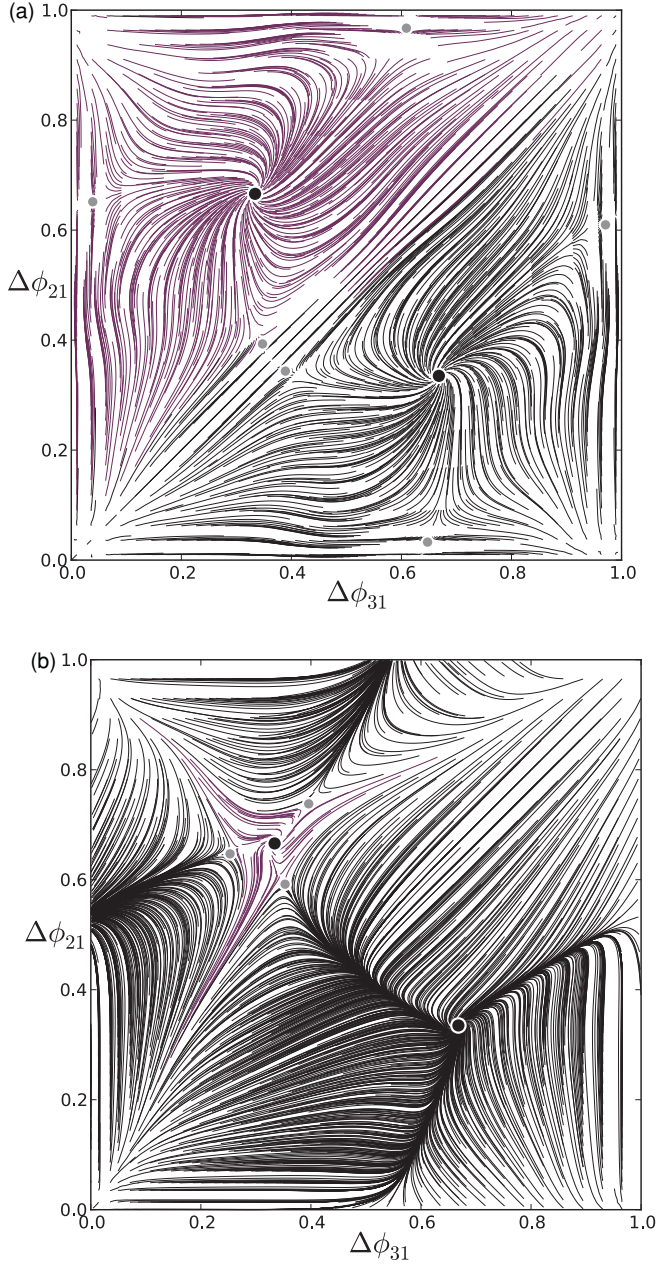
FIG. 5. (Color online) (a) Phase-lag map for the symmetric, long bursting motif revealing two equally dominant attractors: (\frac{2}{3}, \frac{1}{3}) and (\frac{1}{3}, \frac{2}{3}) for (1 < 2 < 3) and (1 < 3 < 2) traveling rhythms. (b) Map for the asymmetric ( g_{\circ} = 0.3 ) medium bursting motif depicting two persistent attractors: the one for the clockwise (1 < 2 < 3) rhythms prevails over the attractor for the counterclockwise (1 < 3 < 2) rhythm. Further increase in g_{\circ} leads to the only observable (1 < 2 < 3) rhythm, after FP at (\frac{1}{3}, \frac{2}{3}) merges with three nearby saddles.
