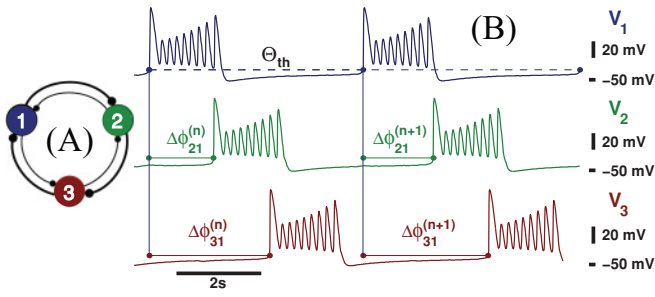
FIG. 1. (Color online) (a) Three-cell motif with asymmetric clockwise vs counterclockwise connection strengths. (b) Voltage traces: the phase (mod 1) of reference cell 1 (blue) is reset when V_1 reaches threshold \Theta_{th} = -40 mV. The time delays between the burst onset in the reference cell 1 and the burst onset in cells 2 (green) and 3 (red), normalized over the recurrent time of cell 1, define a sequence of phase lags \{\Delta\phi_{21}^{(n)}, \Delta\phi_{31}^{(n)}\} .
