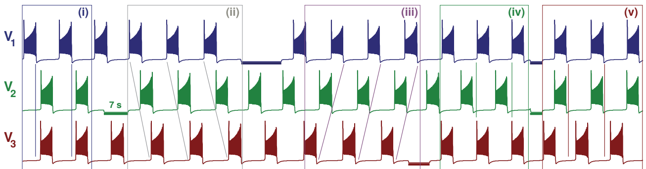
FIG. 2. (Color online) Five polyrhythms in the medium bursting motif at g_{syn} = 5 \times 10^{-3} (increased to secure short transients for the purpose of illustration). Inhibitory pulses (horizontal bars) suppress the targeted cells, thus causing switching between co-existing rhythms: (1 \perp \{2 \parallel 3\}) in episode (i), traveling waves (1 < 2 < 3) in (ii) and (1 < 3 < 2) in (iii), followed by (2 \perp \{1 \parallel 3\}) led by cell 2 in (iv). Having released cells 1 and 2 simultaneously, cell 3 leads the motif in the (3 \perp \{1 \parallel 2\}) rhythm in the last episode.
