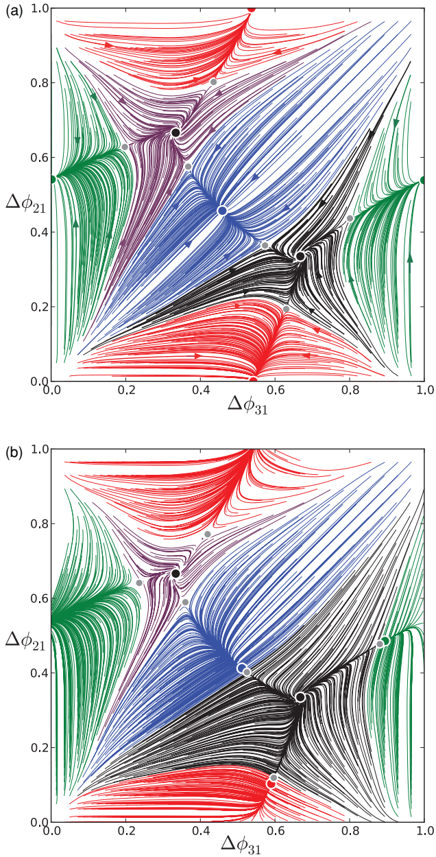
FIG. 3. (Color online) (a) Phase-lag map for the symmetric, medium bursting motif showing five stable FPs: (red) dot at \sim (\frac{1}{2}, 0) , (green) (0, \frac{1}{2}) , (blue) (\frac{1}{2}, \frac{1}{2}) , (black) (\frac{2}{3}, \frac{1}{3}) , and (purple) (\frac{1}{3}, \frac{2}{3}) , corresponding to the antiphase (3 \perp \{1 \parallel 2\}) , (2 \perp \{1 \parallel 3\}) , (1 \perp \{2 \parallel 3\}) bursts, and traveling clockwise (1 < 2 < 3) and counterclockwise (1 < 3 < 2) waves; the attraction basins are divided by “separatrices” (stable sets) of six saddles (small grey dots). Arrows indicate the forward iterate direction in the phase plane. (b) Asymmetric motif at g_{\circ} = 0.154 near the saddle-node bifurcations annihilating three stable FPs for antiphase bursting rhythms.
