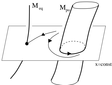
FIGURE 3. An orbit of the fast subsystem may tend to a stable equilibrium, or to a stable limit cycle.
