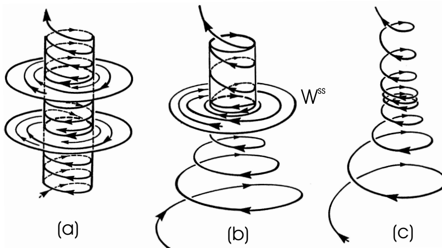
FIGURE 1. Saddle-node bifurcation: (a) \mu < 0 , there are two periodic orbits: stable and saddle; (b) \mu = 0 , the periodic orbits merge into a saddle-node one. Its strong stable manifold W^{ss} divides the neighborhood into the node region (below W^{ss} in the figure) and the saddle region (above W^{ss} ). The unstable manifold is the part of the center manifold which lies in the saddle region. (c) \mu > 0 , the saddle-node disappears; the drifting time throughout its neighborhood is estimated as \sim 1/\sqrt{\mu} .
