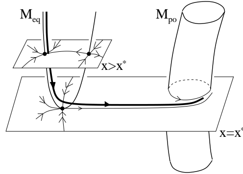
FIGURE 5. Fast jump of the trajectory taking off the fold towards the attracting cylindrical surface.
