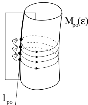
FIGURE 4. The fast circular motion on the cylinder M_{po}(\varepsilon) defines the Poincaré map of the intersection curve l_{po}(\varepsilon) .
