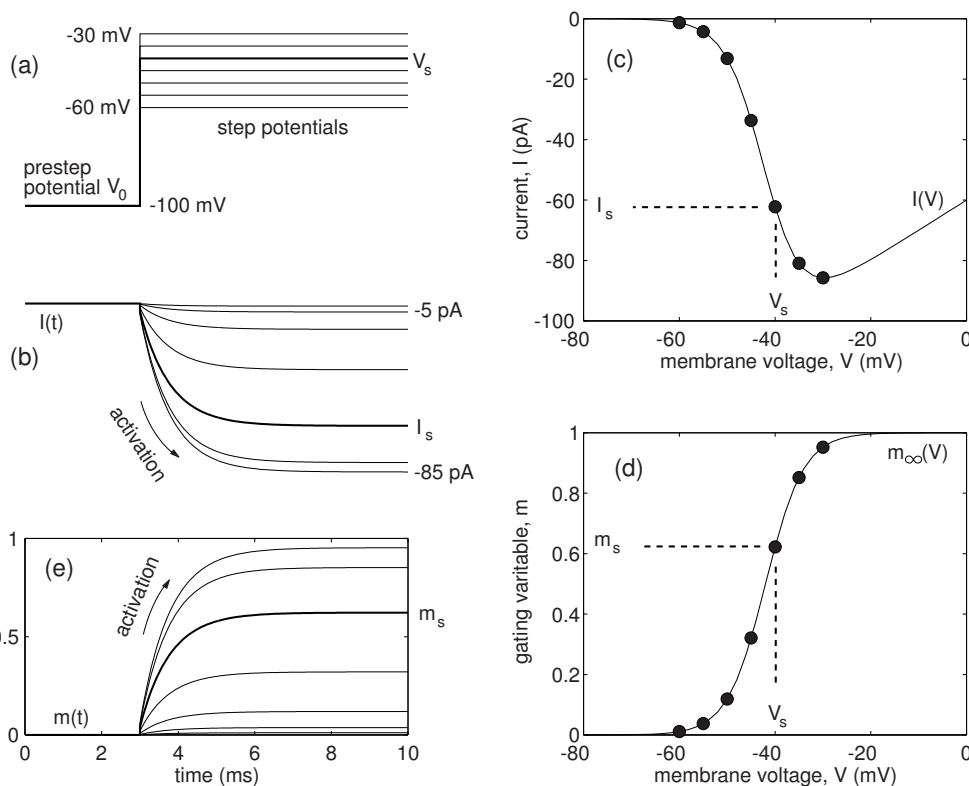
Figure 2.10: An experiment to determine m_\infty(V) . Shown are simulations of the persistent \text{Na}^+ current in Purkinje cells (see Sect. 2.3.5).
