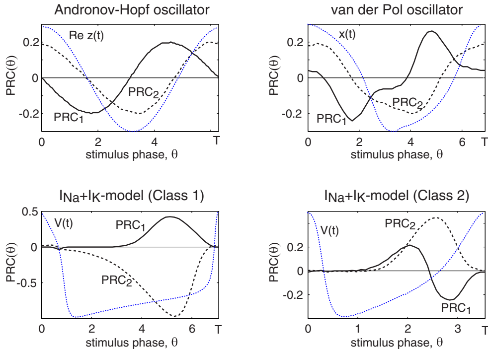
Figure 10.6: Examples of phase response curves (PRC) of the oscillators in Fig. 10.3. \text{PRC}_1(\vartheta) : Horizontal pulses (along the first variable) with amplitudes 0.2, 0.2, 2, 0.2 for Andronov-Hopf, van der Pol, Class 1 and Class 2 oscillators, respectively. \text{PRC}_2(\vartheta) : Vertical pulses (along the second variable) with amplitudes 0.2, 0.2, 0.02, 0.002, respectively. An example of oscillation is plotted as a dotted curve in each subplot (not to scale).
