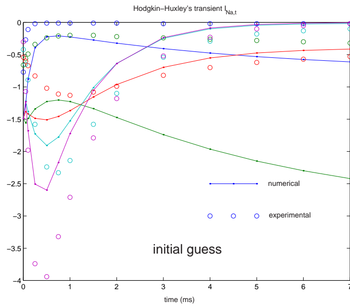
Figure 48: Initial output of the MATLAB numerical optimization procedure; see Ex. 6.
