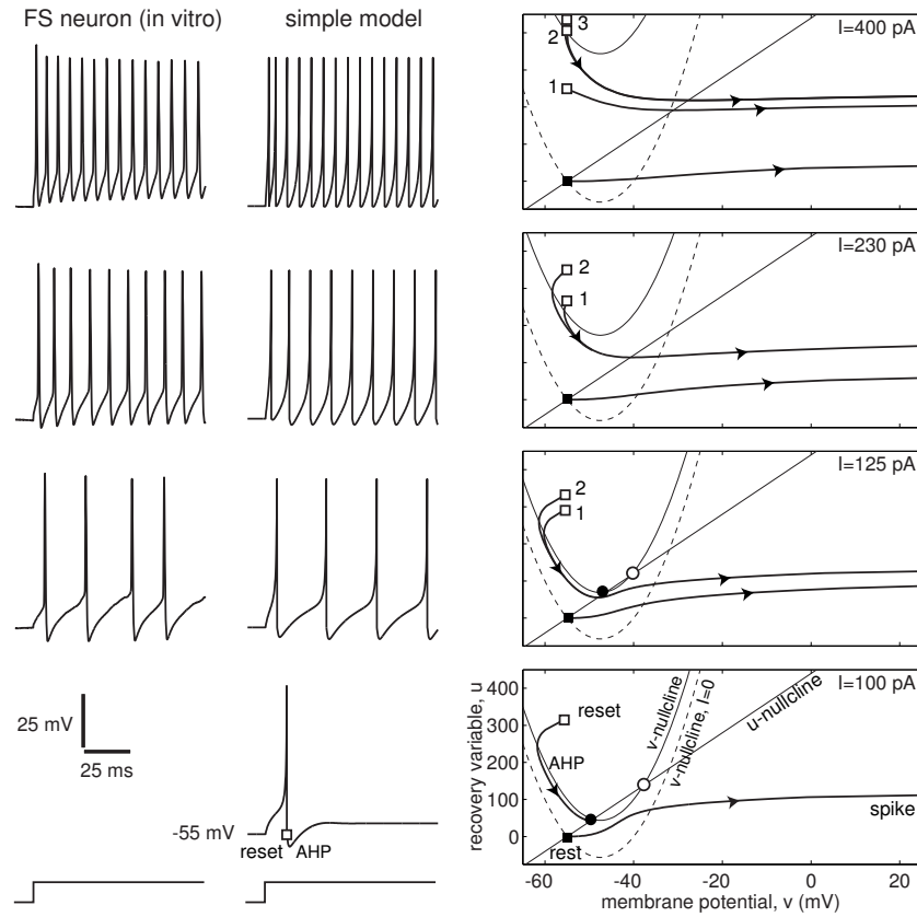
Figure 82: Comparison of in vitro recordings of a fast spiking (FS) interneuron of layer 5 rat's visual cortex with simulations of the simple model with linear slow nullcline 20\dot{v} = (v + 55)(v + 40) - u + I , \dot{u} = 0.15\{8(v + 55) - u\} , if v \geq 25 , then v \leftarrow -55 , u \leftarrow u + 200 .
