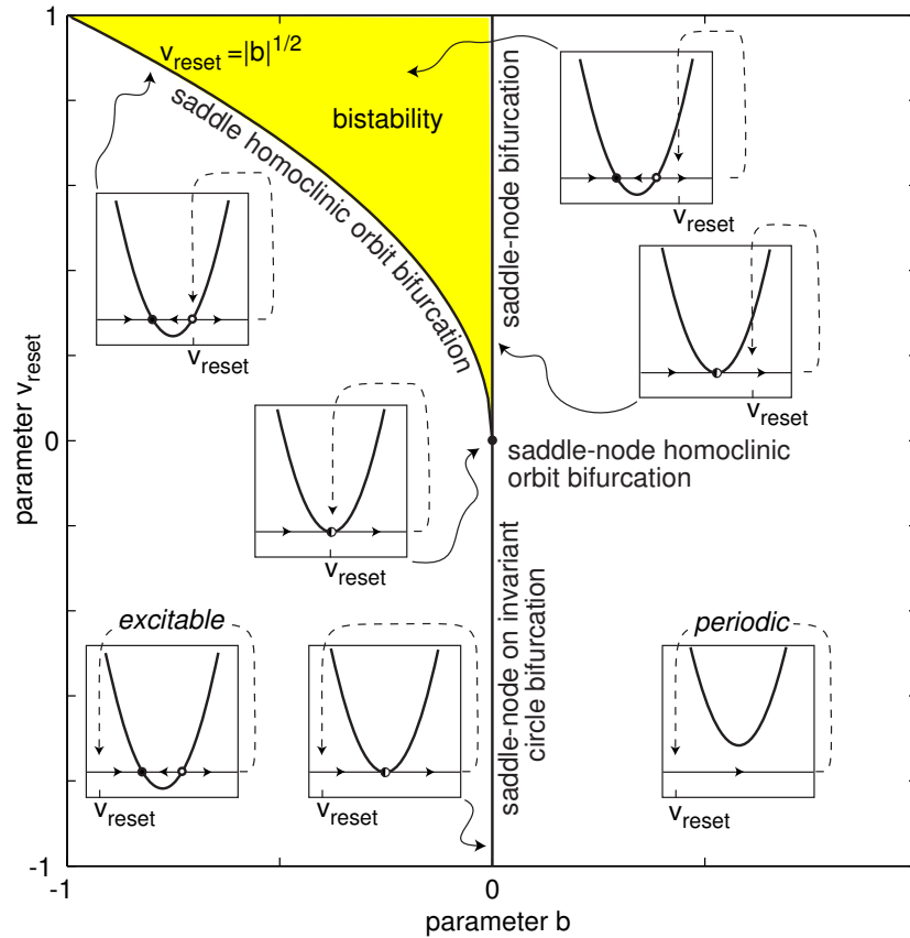
Figure 8.3: Bifurcation diagram of quadratic integrate-and-fire neuron (8.2).
