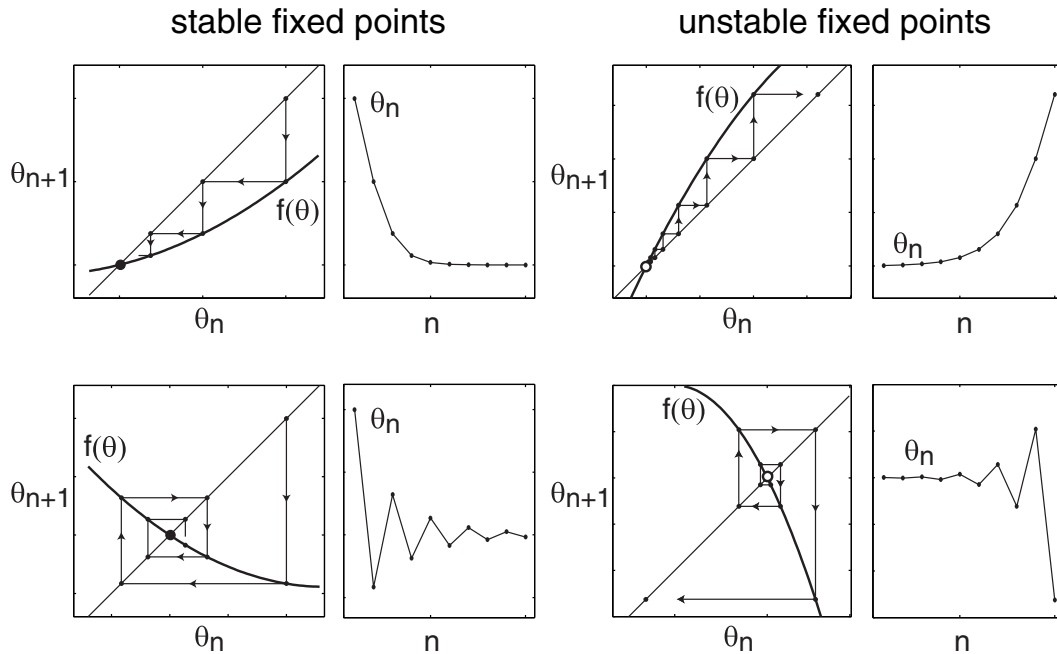
Figure 10.11: Stability of fixed points of the mapping (10.4) depends on the slope of the function f .
