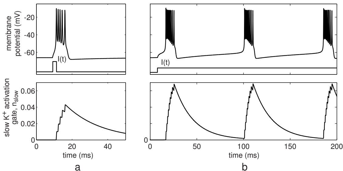
Figure 9.4: Intrinsic bursting in the I_{\text{Na,p}} + I_{\text{K}} + I_{\text{K(M)}} -model (7.1) consisting of the I_{\text{Na,p}} + I_{\text{K}} -model with parameters as in Fig. 4.1a and fast K + current ( g_{\text{K}} = 9 , \tau(V) = 0.152 ) and a slow K + current with g_{\text{slow}} = 5 , V_{1/2} = -20 mV, k = 5 mV and \tau_{\text{slow}}(V) = 20 ms. (a) Burst excitability when I = 0 . (b) Periodic bursting when I = 5 .
