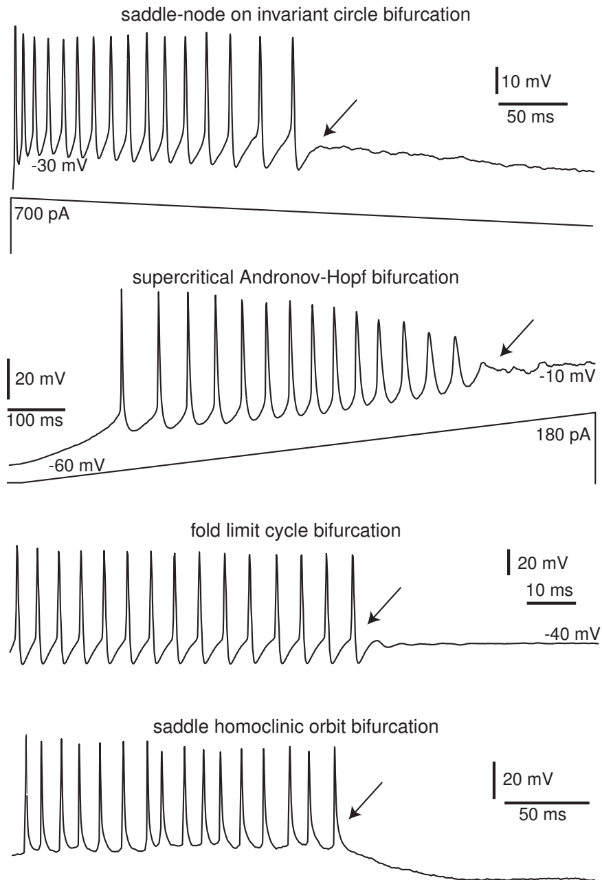
Figure 6.18: Transitions from tonic (periodic) spiking to resting occurs via bifurcations of a limit cycle attractors (marked by arrows). Saddle-node on invariant circle bifurcation: recording of layer 5 pyramidal neuron in rat's visual cortex. Supercritical Andronov-Hopf bifurcation: excitation block in pyramidal neuron of rat's visual cortex. Fold limit cycle bifurcation: brainstem mesencephalic V neuron of rat. Saddle homoclinic orbit bifurcation: neuron in pre-Boltzinger complex of rat brainstem (data provided by C.A. Del Negro and J.L. Feldman).
