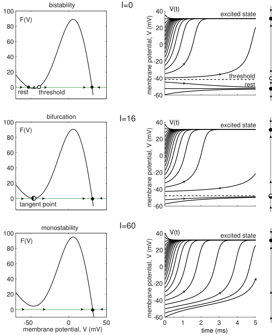
Figure 3.25: Bifurcation in the I_{Na,p} -model (3.5): The rest state and the threshold state coalesce and disappear when the parameter I increases.
