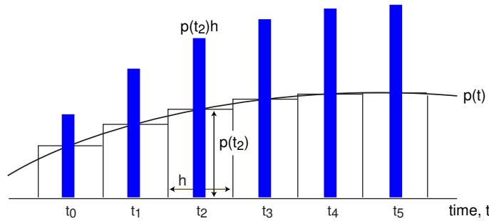
Figure 10.19: Continuous function p(t) is replaced by an equivalent train of pulses of variable amplitudes.
