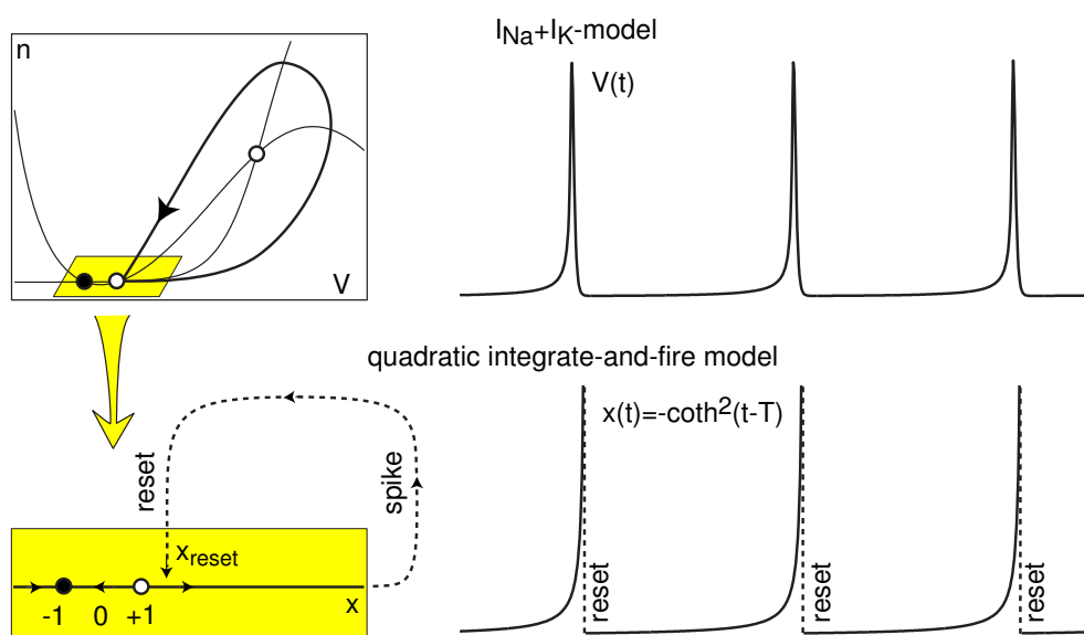
Figure 10.37: Top : Periodic spiking of the I_{Na} + I_K -neuron near saddle-node homoclinic orbit bifurcation (parameters as in Fig. 4.1a with \tau(V) = 0.167 and I = 4.49 ). Bottom : Spiking in the corresponding quadratic integrate-and-fire model.
