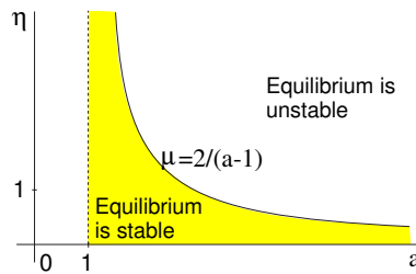
Figure 89: Region of stability of equilibrium of system in Ex. 8.
