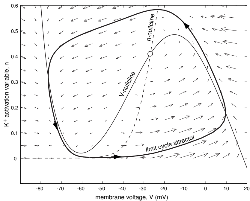
Figure 4.30: Limit cycle attractor (bold) in the I_{Na,p}+I_K -model when I = 10 (compare with Fig. 4.26 and Fig. 4.28).
