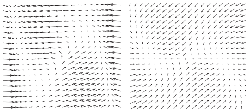
Figure 4.42: Use pencil to draw phase portrait as in Fig. 4.39.
