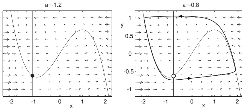
Figure 75: Nullclines and phase portrait of the Bonhoeffer–van der Pol oscillator ( b = 0.05 and c = 0 ).
