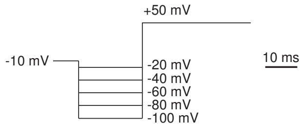
Figure 50: Multiple voltage steps are often needed to determine time constants of inactivation.
