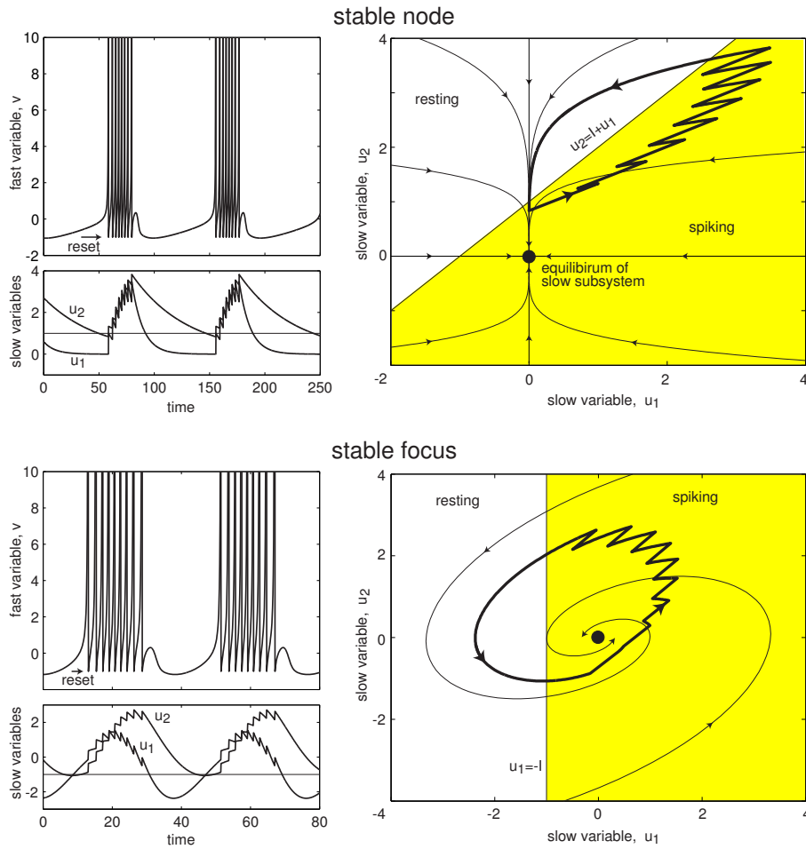
Figure 9.34: “Circle/circle” bursting in the canonical models (9.9) ( top , parameters: I = 1 , \mu_1 = 0.1 , \mu_2 = 0.02 , d_1 = 1 , d_2 = 0.5 ) and (9.10) ( bottom , parameters: I = 1 , \mu_1 = 0.2 , \mu_2 = 0.1 , d_1 = d_2 = 0.5 ).
