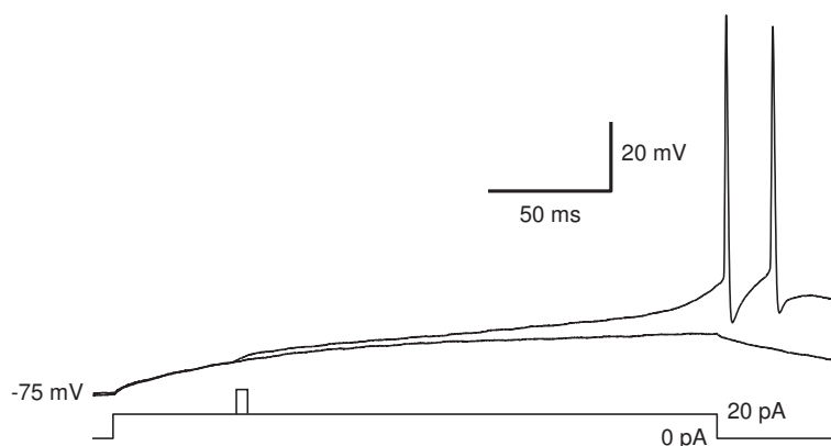
Figure 7.34: Long latencies and threshold crossing of Layer 5 neuron recorded in vitro in rat motor cortex.
