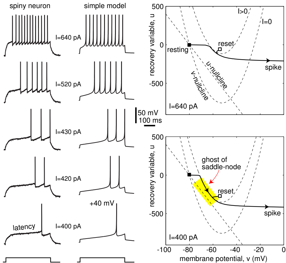
Figure 8.30: Comparison of in vitro recordings of a neostriatal spiny projection neuron of a rat with simulations of the simple model 50\dot{v} = (v + 80)(v + 25) - u + I , \dot{u} = 0.01\{-20(v + 80) - u\} , if v \geq 40 , then v \leftarrow -55 , u \leftarrow u + 150 ( in vitro data were kindly provided by C. Wilson).
