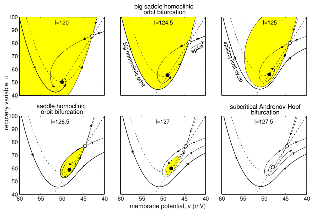
Figure 8.12: The sequence of bifurcations of RS model neuron (8.5, 8.6) in resonator regime. Parameters as in Fig. 8.9 and b = 5 ; see also Fig. 6.40.
