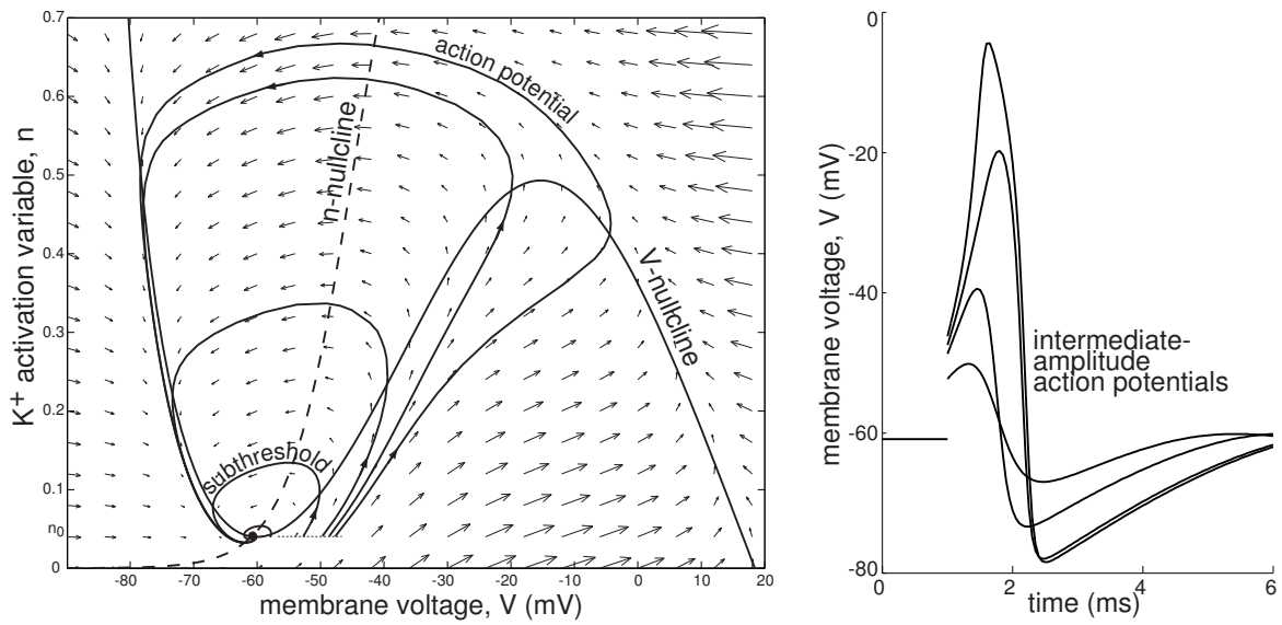
Figure 4.7: Failure to generate all-or-none action potentials in the I_{Na,p} + I_K -model (4.1, 4.2)
