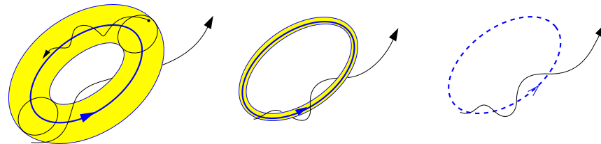
Subcritical Neimark-Sacker Bifurcation
