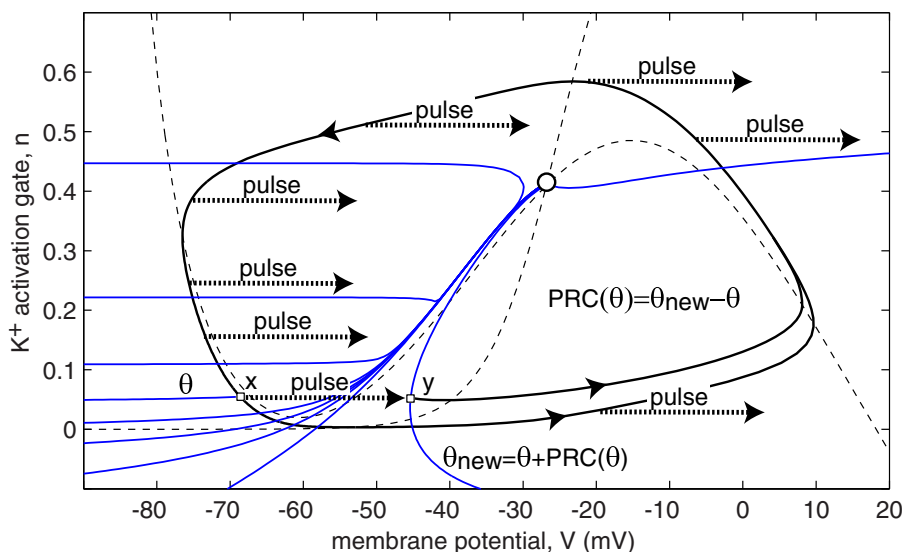
Figure 10.5: The geometrical relationship between isochrons and phase response curve (PRC) of the I_{Na} + I_K -oscillator in Fig. 10.1.
