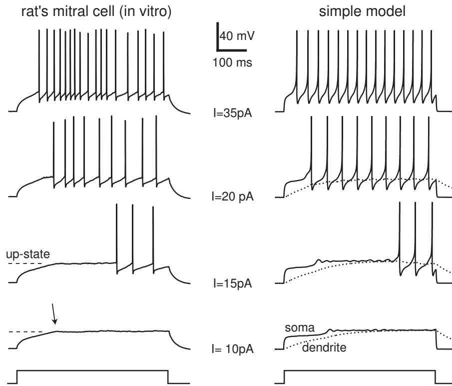
Figure 8.33: Comparison of in vitro recordings of mitral neurons of rat's olfactory bulb with simulations of the simple two-compartment model. Soma: 40\dot{v} = (v+55)(v+50) + 0.5(v_d - v) - u + I , \dot{u} = 0.4\{U(v) - u\} with U(v) = 0 when v < v_b and U(v) = 20(v - v_b) when v \geq v_b = -48 mV. If v \geq 35 , then v \leftarrow -50 . Passive dendrite (dotted curve): \dot{v}_d = 0.0125(v - v_d) . Weak noise was added to simulations to unmask subthreshold oscillations in the up-state. The membrane potential of the neuron is held at -75mV by injecting a strong negative current, and then stimulated with steps of positive current. (Data were kindly provided by Philip Heyward.)
