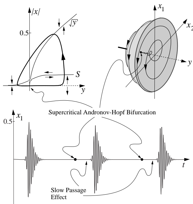
Figure 87: Hopf/Hopf bursting without co-existence of attractors; see Ex. 6 (modified from Hoppensteadt and Izhikevich 1997).
