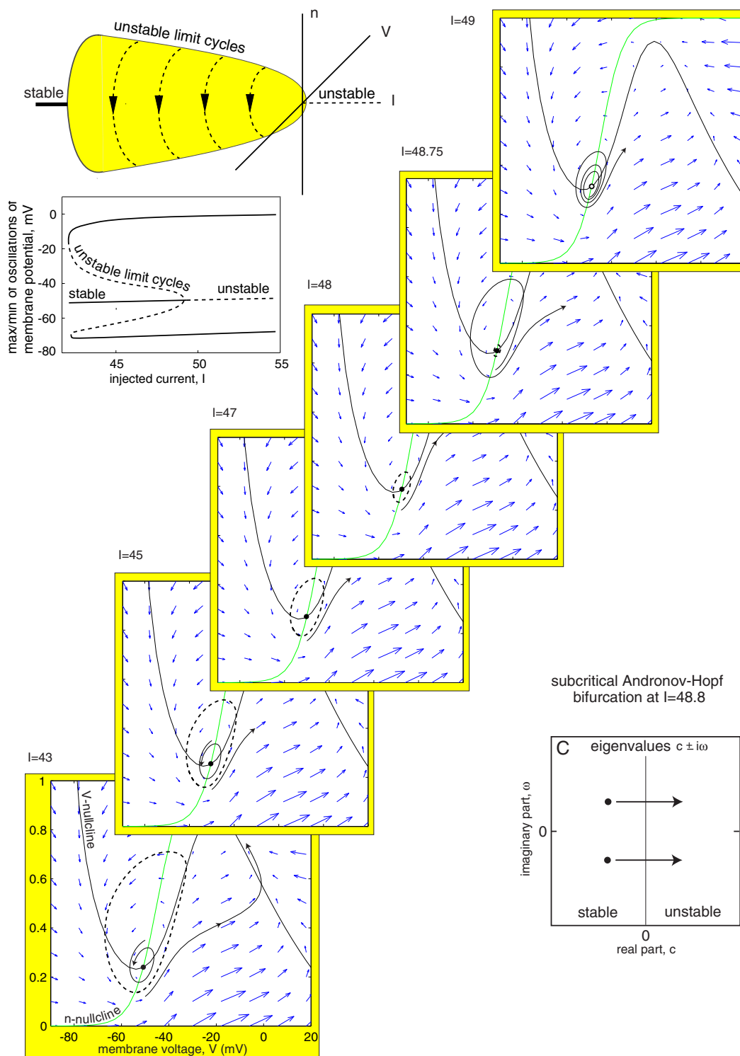
Figure 6.16: Subcritical Andronov-Hopf bifurcation in the I_{Na,p} + I_K -model: As the bifurcation parameter I increases, an unstable limit cycle (dashed circle; see also Fig. 6.14) shrinks to an equilibrium and makes it lose stability. Parameters as in Fig. 4.1b except g_L = 1 , g_{Na} = g_K = 4 , and the Na^+ activation function has V_{1/2} = -30 mV and k = 7 .
