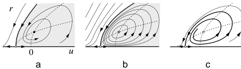
Figure 90: Phase portraits of the system in Ex. 8 for a = 5 and various \mu . a. \mu = 0.4 . b. \mu = 0.5 . c. \mu = 0.6 . Bold curves are separatrices of the saddle (u, r) = (-1, 0) , and dashed curves are nullclines of the system.
