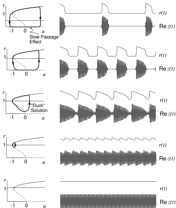
Figure 95: Phase portrait and solution of the canonical model from Ex. 15 with \mu = 0.1 , \omega = 3 and various a . From top to bottom: a = 0.25 , a = 0.8 , a = 0.986 , a = 0.987 , and a = 1.2 .
