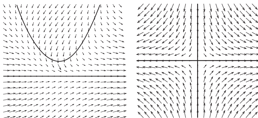
Figure 63: Nullclines of the vector field; see also Fig. 69.
