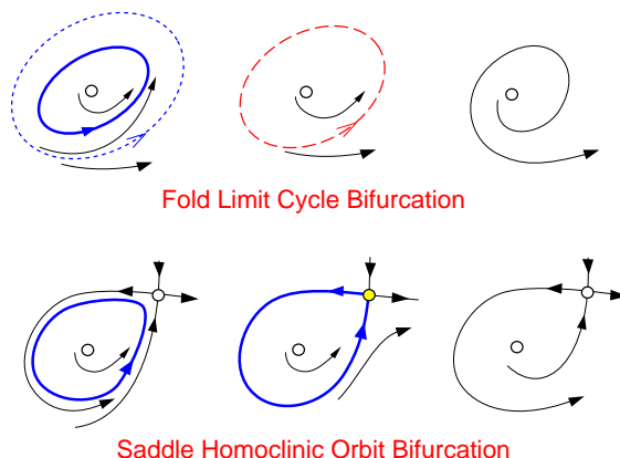
Figure 99: Codimension 1 bifurcations of a stable limit cycle in planar systems that result in sharp loss of stability and transition to a large-amplitude (spiking) limit cycle attractor, not shown in the figure. Fold limit cycle : Stable limit cycle is approached by an unstable one, they coalesce, and then disappear. Saddle homoclinic orbit : A limit cycle grows into a saddle. Unstable manifold of the saddle makes a loop and returns via the stable manifold (separatrix).
