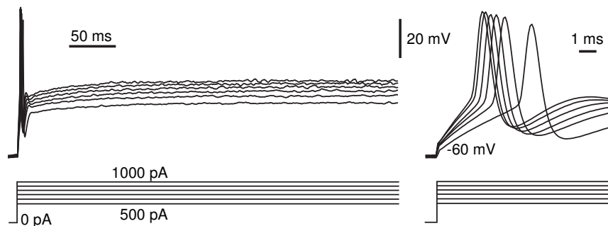
Figure 7.4: Class 3 excitability of a mesV neuron of rat's brainstem (contrast with Fig. 7.3).
