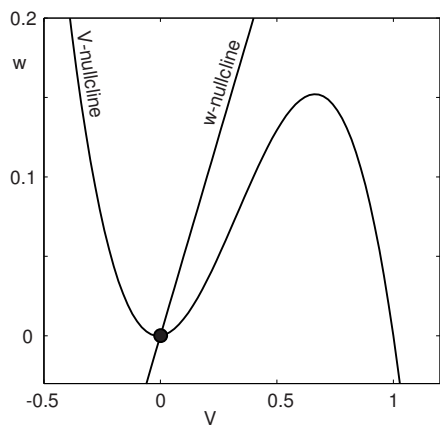
Figure 9.56: Rebound bursting in the FitzHugh-Nagumo oscillator; see Ex. 4.
