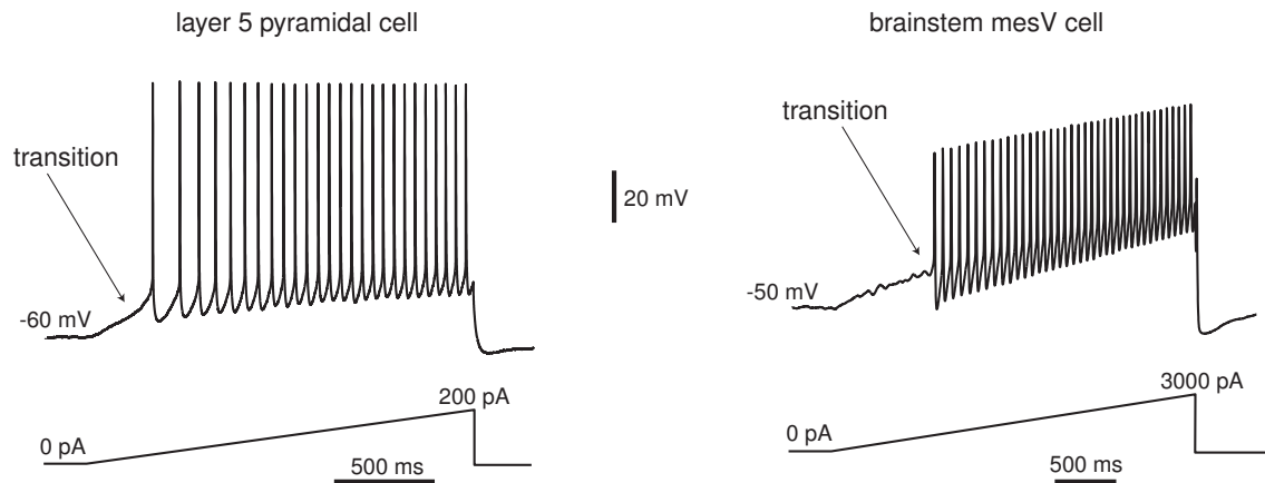
Figure 7.6: As the magnitude of injected dc-current increases, the neurons bifurcates from resting to repetitive spiking behavior. Shown are recordings of the same neurons as in Fig. 7.3. Notice that the ratio of the first and last interspike intervals of the pyramidal cell is much greater than that in mes V neuron.
