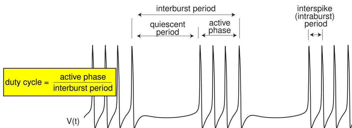
Figure 9.5: Basic characteristics of bursting dynamics.
