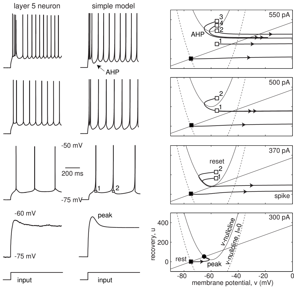
Figure 8.15: Comparison of in vitro recordings of an intrinsically bursting (IB) neuron with the simple model 150\dot{v} = 1.2(v + 75)(v + 45) - u + I , \dot{u} = 0.01\{5(v + 75) - u\} , if v \geq +50 , then v \leftarrow -56 , u \leftarrow u + 130 . White squares denote the reset points numbered according to the spike number.
