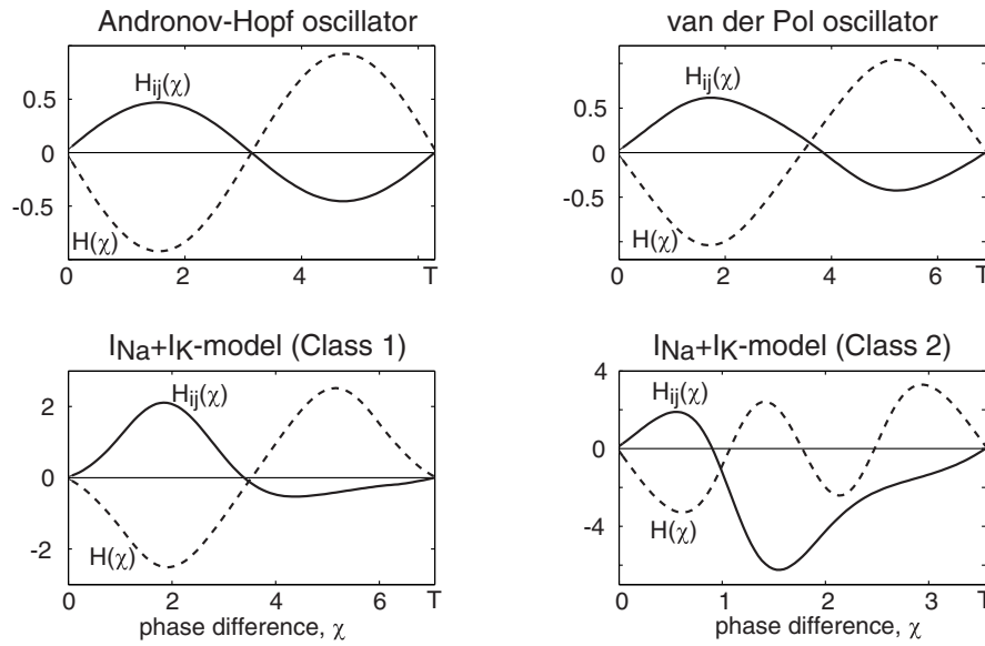
Figure 10.26: Solid curves: Functions H_{ij}(\chi) defined by (10.16) with the input g(x_i, x_j) = (x_{j1} - x_{i1}, 0) corresponding to electrical synapse via gap-junction. Dashed curves: Functions H(\chi) = H_{ji}(-\chi) - H_{ij}(\chi) . Parameters as in Fig. 10.3.
