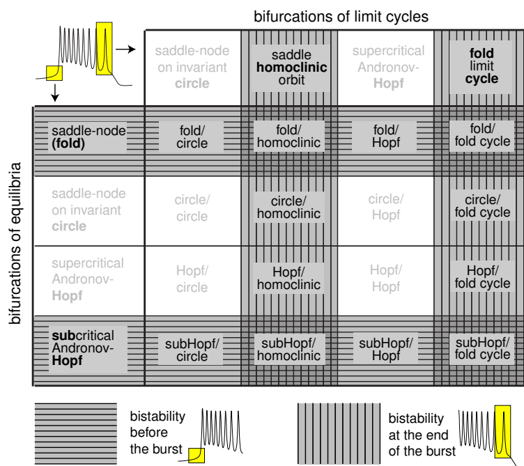
Figure 9.46: Bistability, i.e., co-existence of resting and spiking states, depends on the topological type of bursting.
