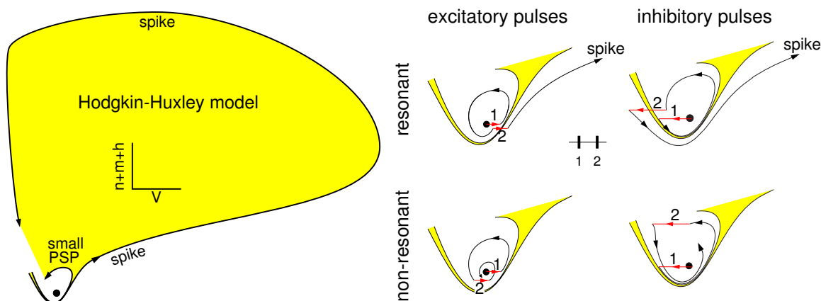
Figure 7.22: (Left) Projection of trajectories of the Hodgkin-Huxley model on a plane. (Right) Phase portrait and typical trajectories during (non-) resonant response of the model to excitatory and inhibitory doublets of spikes. Modified from Izhikevich (2000).
