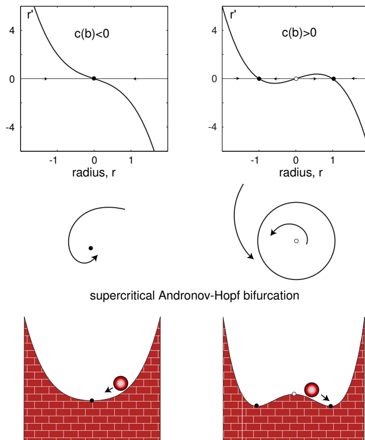
Figure 6.13: Supercritical Andronov-Hopf bifurcation in (6.5, 6.6) with c = \pm 1 and a = -1 .
