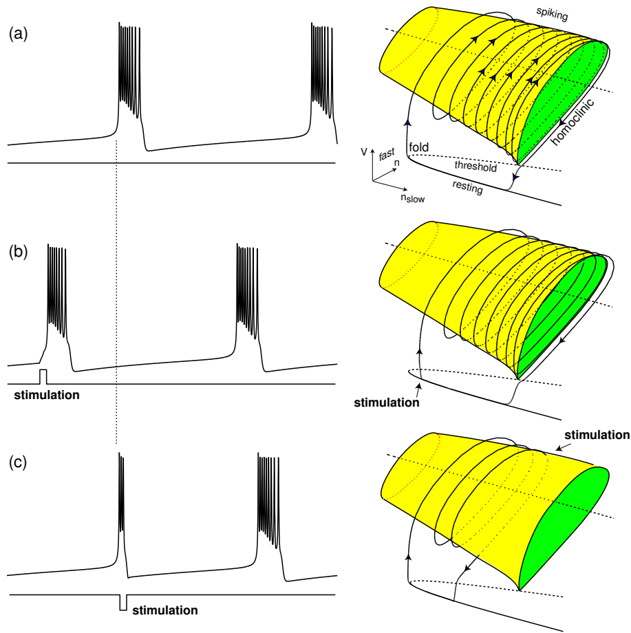
Figure 9.47: Bistability of resting and spiking states in “fold/homoclinic” burster. A brief stimulus can switch between resting and spiking states. Shown are simulations of the I_{Na,p}+I_K+I_{K(M)} -model with parameters as in Fig. 9.4b.
