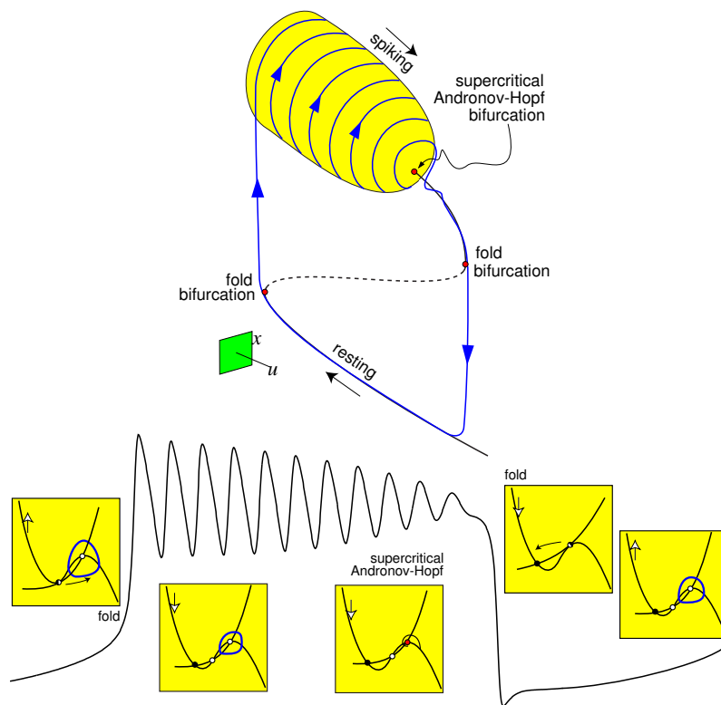
Figure 9.43: “Fold/Hopf” bursting: The resting state disappears via saddle-node (fold) bifurcation and the spiking limit cycle shrinks to a point via supercritical Andronov-Hopf bifurcation (modified from Izhikevich 2000).
