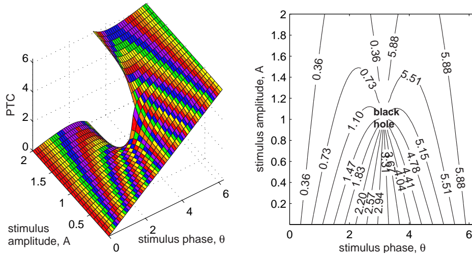
Figure 10.8: Time crystal (left) and its contour plot (right). Shown is the PTC (\vartheta, A) of the Andronov-Hopf oscillator (see Ex. 4).
