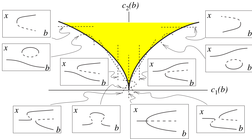
Figure 6.35: Summary of special cases for the supercritical cusp bifurcation. Dotted segments are paths c_1 = c_1(b) , c_2 = c_2(b) , where b is a one-dimensional bifurcation parameter. Corresponding bifurcation diagrams are depicted in boxes. Continuous curves represent stable solutions, dashed curves represent unstable solutions (modified from Hoppensteadt and Izhikevich 1997).
