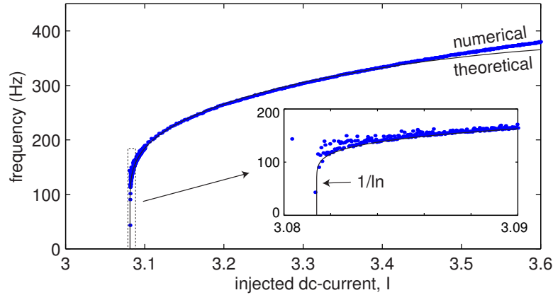
Figure 6.30: Frequency of spiking in the I_{Na,p}+I_K -model with parameters as in Fig. 6.28 near a saddle homoclinic orbit bifurcation. Dots are numerical results; the continuous curve is \omega(I) = 1000\lambda(I)/\{-\ln(0.2(I - 3.0814))\} , where the eigenvalue \lambda(I) = 0.87\sqrt{4.51 - I} was obtained from the normal form (6.3). The inset shows a magnified region near the bifurcation value I = 3.0814 .
