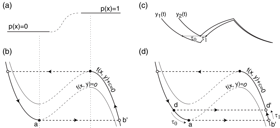
Figure 10.39: Fast threshold modulation of relaxation oscillation. (a) Heaviside or sigmoidal coupling function p(x) is constant while x is on the left or right branch of the x -nullcline. (b) In the relaxation limit \mu = 0 , synchronized limit cycle consists of the left branch of the nullcline f(x, y) = 0 and the right branch of the nullcline f(x, y) + \epsilon = 0 . When oscillator 1 is ahead of oscillator 2 (c), the phase difference between them decreases after the jump (d).
