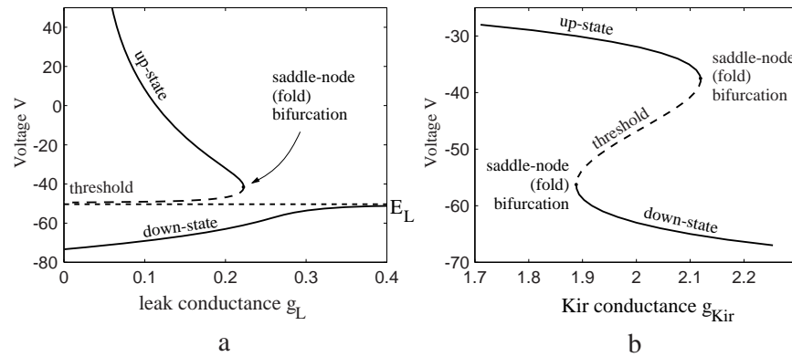
Figure 60: Bifurcation diagrams of the I_{\text{Kir}} -model (3.11), I = 6 , with bifurcation parameters (a) g_L and (b) g_{\text{Kir}} (see Chap. 3, Ex. 12).
