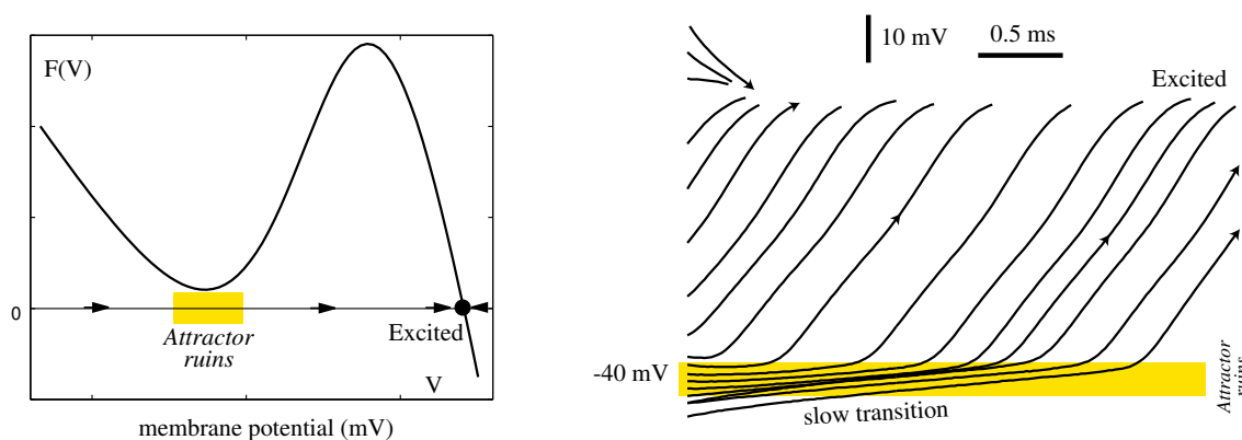
Figure 3.28: Slow transition through the ghost of the resting state attractor in cortical pyramidal neuron with I = 30 pA (the same neuron as in Fig. 3.15). Even though the resting state has already disappeared, the function F(V) , and hence the rate of change, \dot{V} , is still small when V \approx -46 mV.
