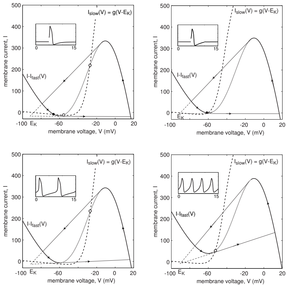
Figure 5.25: Ex. 5: The (V, I) -phase plane of the I_{Na,p} + I_K -model (compare with Fig. 5.4).
