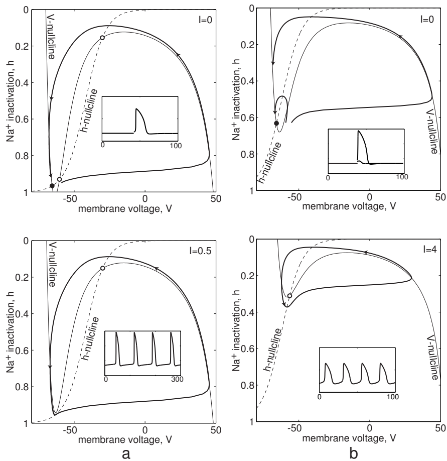
Figure 5.6: Possible forms of nullclines in the I_{Na,t} -model. Notice that the h -axis is inverted. Parameters for I_{Na,t} are as in Hodgkin-Huxley model except \tau_h(V) = 5 ms. E_{Na} = 60 mV, E_L = -70 mV, g_L = 1 , g_{Na} = 15 (in b) and g_{Na} = 10 and V_{1/2} = -42 mV (in a).
