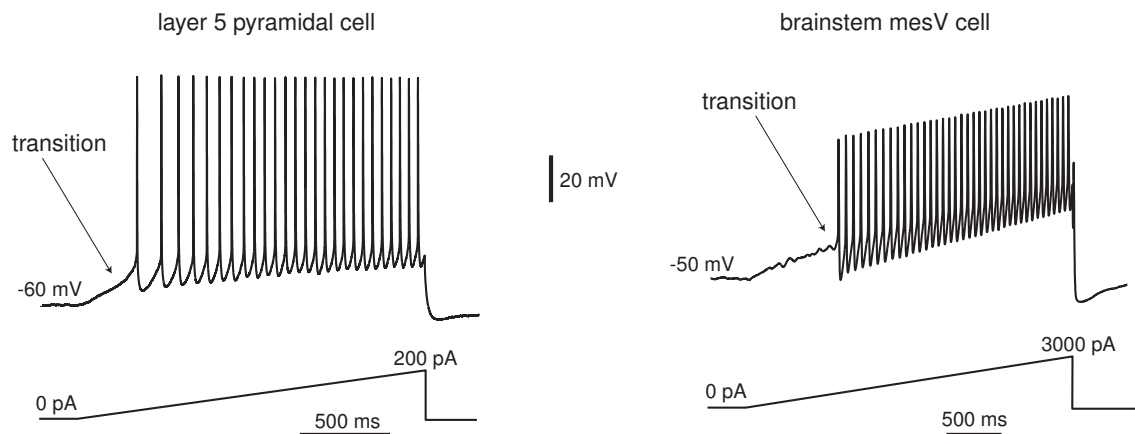
Figure 1.11: As the magnitude of the injected current slowly increases, the neurons bifurcate from resting (equilibrium) to tonic spiking (limit cycle) modes.
