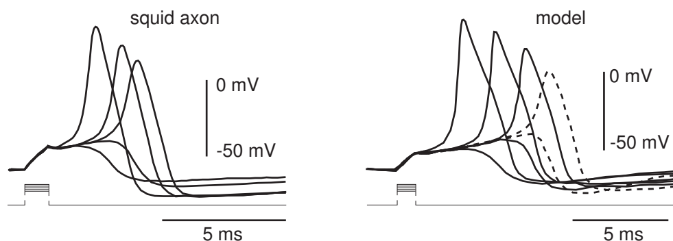
Figure 7.26: Variable-size action potentials in squid giant axon and revised Hodgkin-Huxley model (Clay 1998) in response to brief steps of currents of variable magnitudes (data was kindly provided by John Clay).
