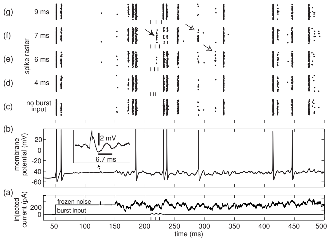
Figure 7.24: Frozen-noise experiments demonstrate frequency preference and resonance to embedded bursts. (a) A random signal (frozen noise) is injected into a neuron in vitro to simulate the in vivo conditions (b). The neuron responds with some spike-timing variability depicted in (c). (d-g) Burst input is added to the frozen noise. Notice that the neuron is most sensitive to the input having the resonant period 7 ms, which is near the period of subthreshold oscillation (6.7 ms). Shown are in vitro responses of mesencephalic V neuron of rats brainstem recorded by the author, Niraj S. Desai, and Betsy C. Walcott. The order of stimulation was first line of c,d,e,f,g, then second line of c,d,e,f,g, then third line, etc., to avoid slow artifacts.
