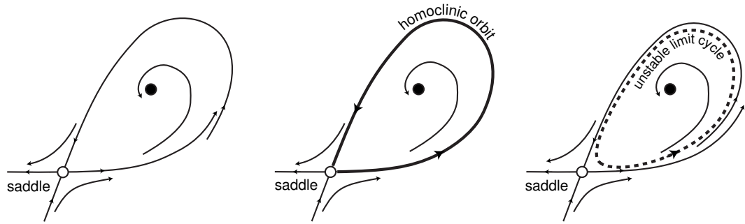
b. subcritical saddle homoclinic orbit bifurcation
