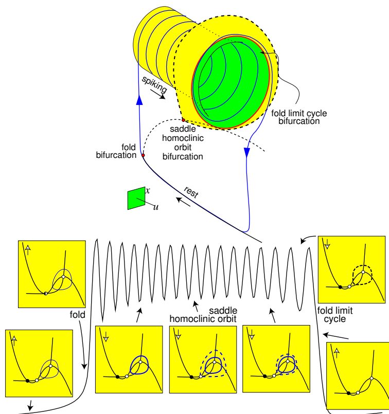
Figure 9.42: “Fold/fold cycle” bursting: The resting state disappears via saddle-node (fold) bifurcation and the spiking limit cycle disappears via fold limit cycle bifurcation (modified from Izhikevich 2000).
