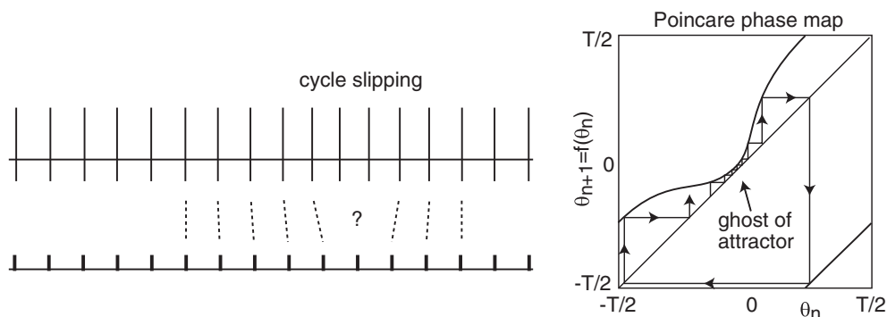
Figure 10.16: Cycle slipping phenomenon at the edge of the Arnold tongue corresponding to a synchronized state.
