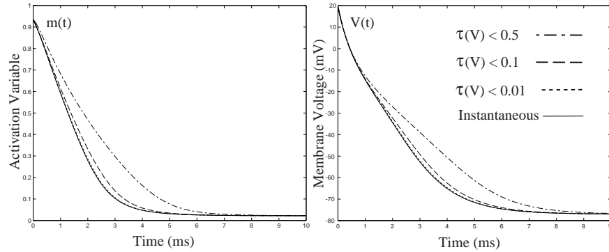
Figure 3.1: Solution of the full system (3.2, 3.3) converges to that of the reduced one-dimensional system (3.4) as \tau(V) \rightarrow 0
