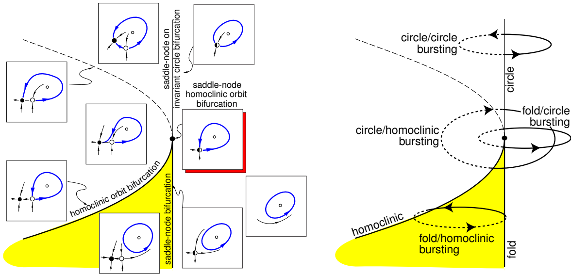
Figure 9.28: A neural system near co-dimension-2 saddle-node homoclinic orbit bifurcation (center dot) can exhibit four different types of fast-slow bursting, depending on the trajectory of the slow variable u \in \mathbb{R}^2 in the two-dimensional parameter space. Solid (dotted) lines correspond to spiking (resting) regimes.
