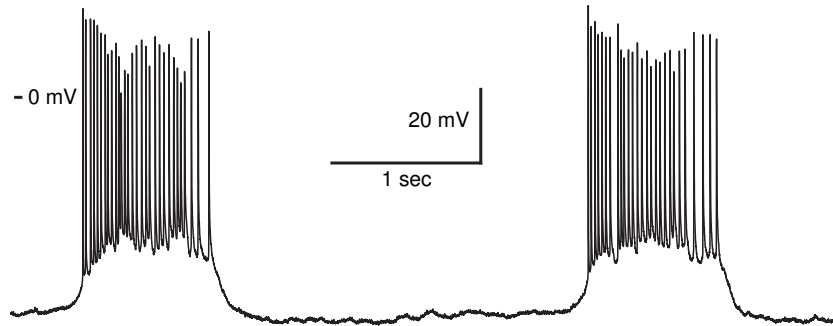
Figure 9.27: Putative “fold/homoclinic” bursting in a cell located in pre-Botzinger complex of rat brain stem (data kindly shared by Christopher A. Del Negro and Jack L. Feldman, Systems Neurobiology Laboratory, Department of Neurobiology, UCLA.)
