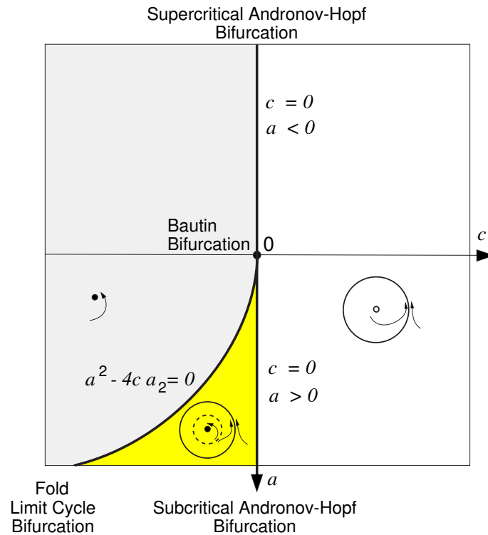
Figure 6.42: Supercritical Bautin bifurcation in (6.8); see also Fig. 9.41, left.
