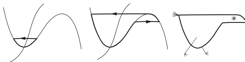
Figure 6.41: French duck (canard) limit cycles in relaxation oscillators.
