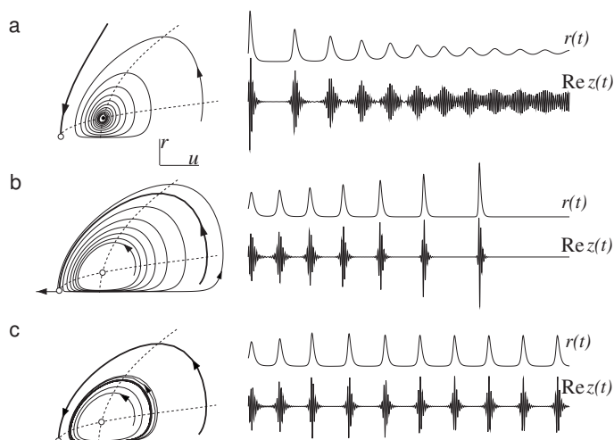
Figure 91: Simulations of the canonical model in Ex. 8. Parameters: \omega = 5 . a. \mu = 1/12 . b. \mu = 1/8 . c. \mu = 1/8 , but additive noise of amplitude 10^{-3} is added to the right-hand side.
