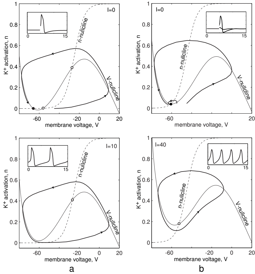
Figure 5.4: Possible forms of nullclines in the I_{Na,p}+I_K -model. Parameters as in the previous chapter (see caption to Fig. 4.1).
