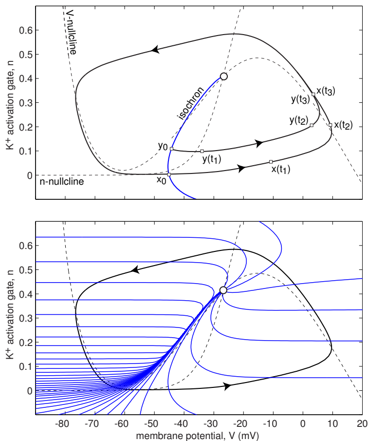
Figure 10.2: Top : An isochron, or a stable manifold, of a point x_0 on the limit cycle attractor is the set of all initial conditions y_0 such that y(t) \rightarrow x(t) as t \rightarrow +\infty . Bottom : Isochrons of the limit cycle attractor in Fig. 10.1 corresponding to 40 evenly distributed phases nT/40 , n = 1, \dots, 40 .
