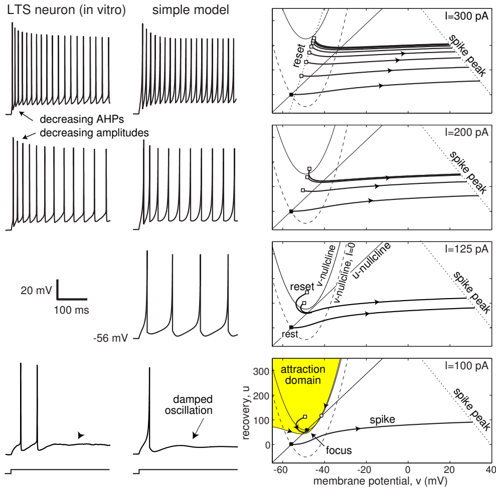
Figure 8.20: Comparison of in vitro recordings of a low threshold spiking (LTS) interneuron (rat's barrel cortex, data provided by B. Connors) with simulations of the simple model 100\dot{v} = (v + 56)(v + 42) - u + I , \dot{u} = 0.03\{8(v + 56) - u\} , if v \geq 40 - 0.1u , then v \leftarrow -53 + 0.4u , u \leftarrow u + 20 .
