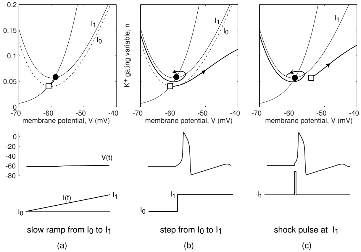
Figure 7.9: The difference between ramp, step, and shock stimulation is in the resetting of initial condition.
