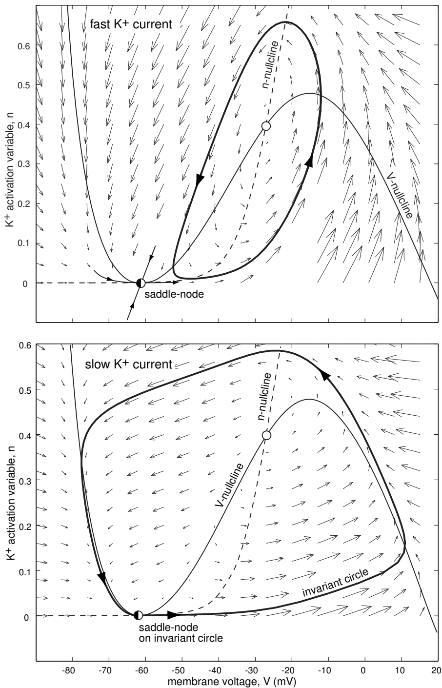
Figure 6.7: Saddle-node bifurcation in the I_{Na,p}+I_K -model with high-threshold K^+ current can be off limit cycle (top) or on invariant circle (bottom). Parameters as in Fig. 4.1a with \tau(V) = 0.152 (top) or \tau(V) = 1 (bottom).
