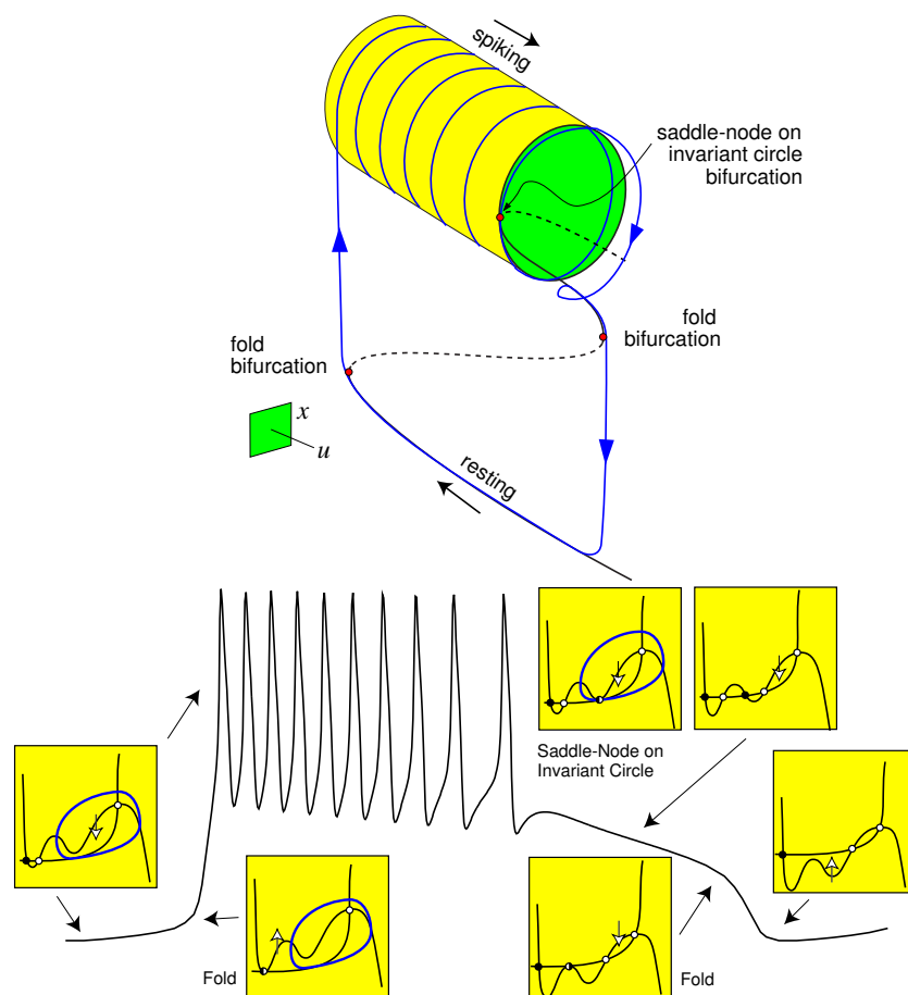
Figure 9.44: “Fold/circle” bursting: The resting state disappears via fold bifurcation and the spiking state disappears via saddle-node on invariant circle bifurcation (modified from Izhikevich 2000).
