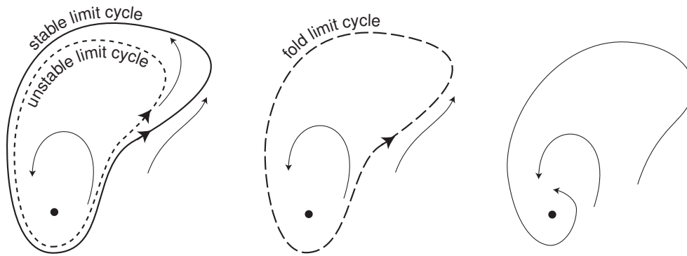
Figure 6.22: Fold limit cycle bifurcation: Stable and unstable limit cycle approach and annihilate each other.
