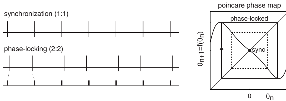
Figure 10.14: The coexistence of synchronized and phase-locked solutions corresponds to the coexistence of stable fixed point and a stable periodic orbit of the Poincare phase map.
