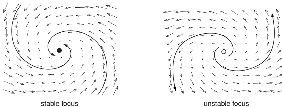
Figure 4.18: Focus equilibrium occurs when eigenvalues are complex-conjugate, e.g., \lambda = -3 \pm i (stable) or \lambda = +3 \pm i (unstable). The imaginary part (here 1) determines the frequency of rotation around the focus.
