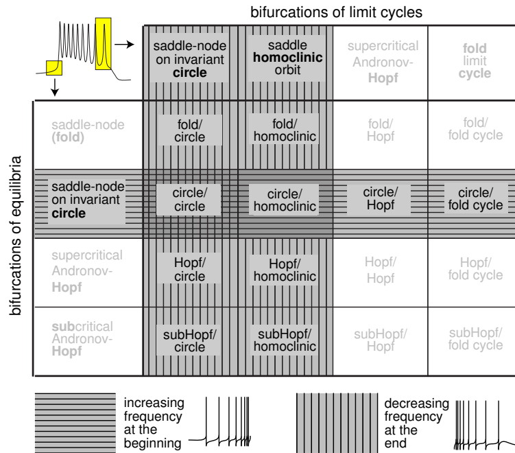
Figure 9.49: Topological types of bursters in the shaded regions can produce chirp-bursters that sweep a frequency range.
