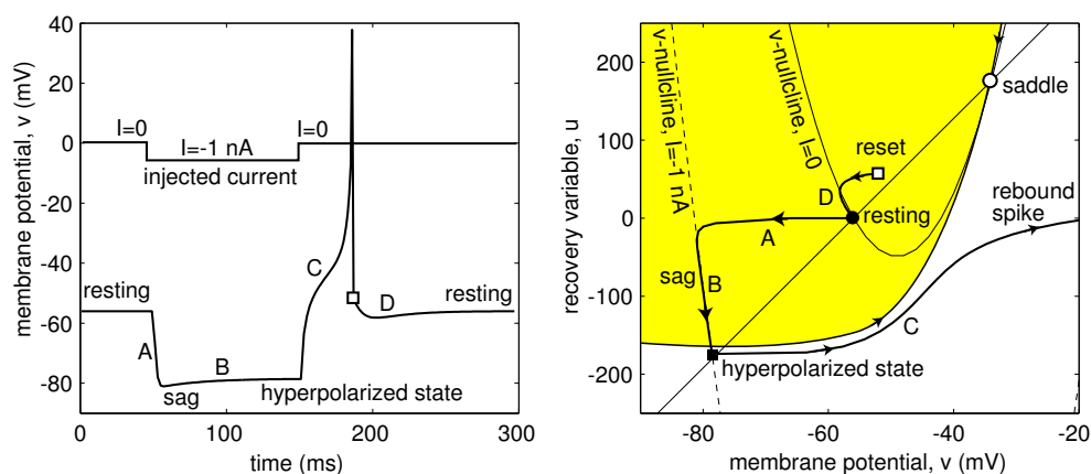
Figure 8.21: The mechanism of sag and rebound spike of the model in Fig. 8.20.
