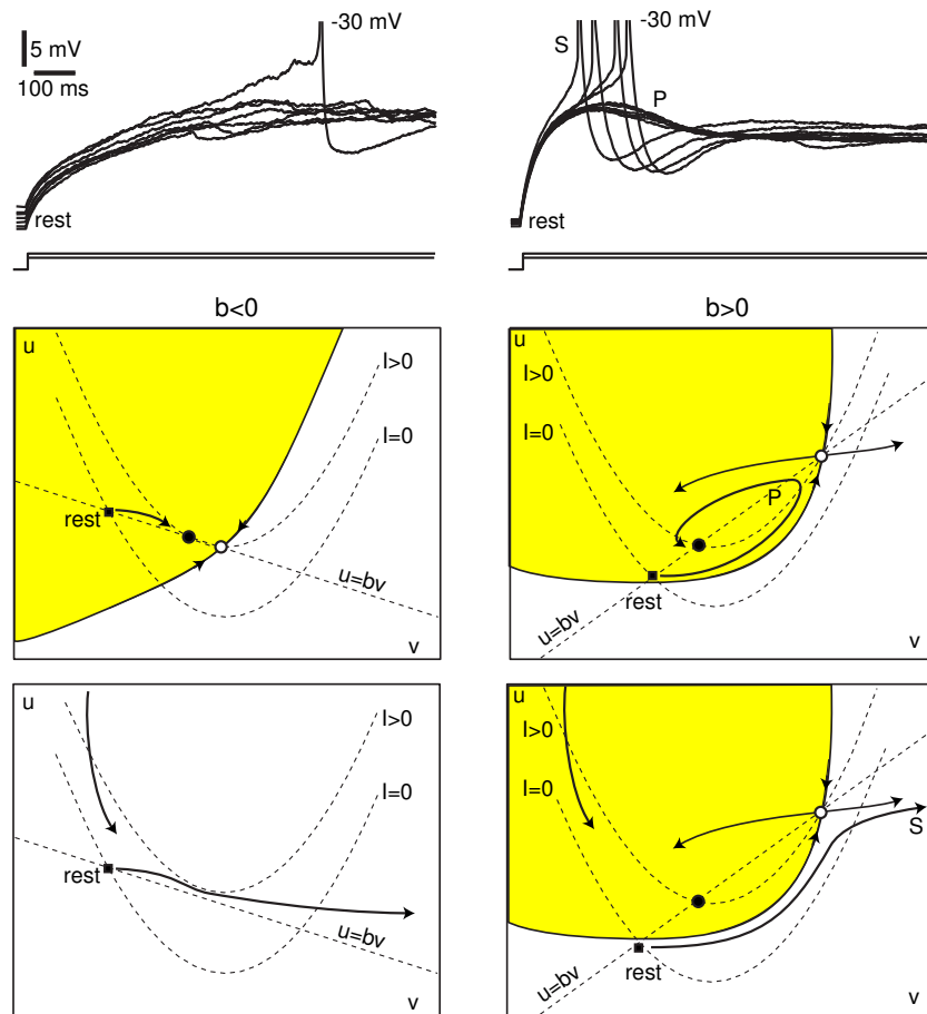
Figure 8.10: Two types of qualitative behavior of RS neurons. Some exhibit monotone responses to weak injected currents (case b < 0 ), others exhibit non-monotone overshooting responses (case b > 0 ). Shown are in vitro recordings of two RS neurons from the same slice of rat's primary visual cortex while an automated procedure was trying to determine the neurons' rheobase. Phase portraits are drawn by hand and they illustrate a possible dynamic mechanism of the phenomenon.
