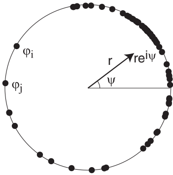
Figure 10.33: Kuramoto synchronization index (10.21) describes the degree of coherence in the network (10.20).
