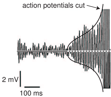
Figure 9.45: The conductance noise destabilizes the focus equilibrium in a mesencephalic V neuron before subcritical Andronov-Hopf bifurcation takes place, thereby giving an impression of a supercritical Andronov-Hopf bifurcation (data modified from Wu et al. 2001).
