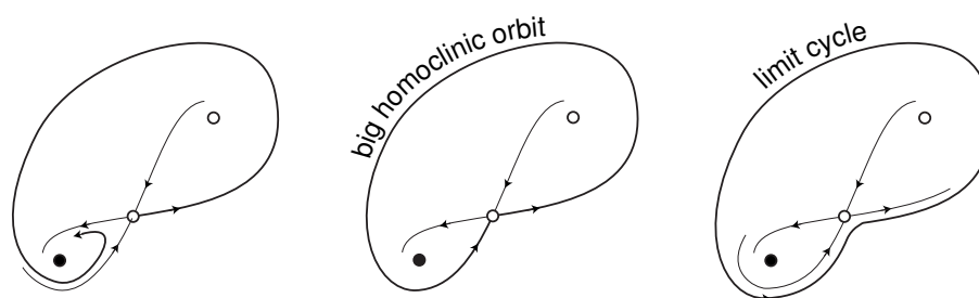
Figure 6.31: Big saddle homoclinic orbit bifurcation.
