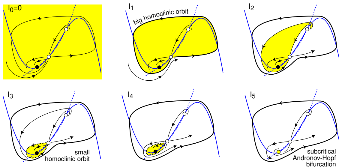
Figure 6.40: Transformations of phase portraits of a neuronal model near subcritical Bogdanov-Takens bifurcation point as the magnitude of the injected current I increases (here I_{k+1} > I_k ). Shaded regions are the attraction domains of the equilibrium corresponding to the resting state.
