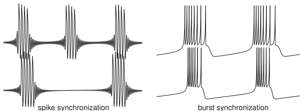
Figure 9.50: Various regimes of synchronization of bursters.
