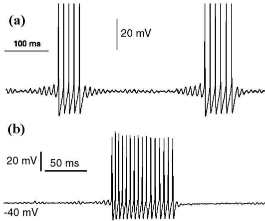
Figure 9.38: Putative “subHopf/fold cycle” bursting in (a) injured dorsal root ganglion (data modified from Jian et al. 2004) and in (b) rat’s mesencephalic V neurons.
