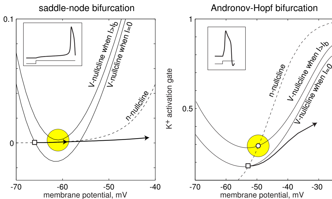
Figure 7.35: Bifurcation mechanism of latency to first spike when injected dc-current steps from I = 0 to I > I_b , where I_b is a bifurcation value. Shaded circle denotes the region where vector-field is small. Shown are phase portraits of the I_{Na,p} + I_K -model.
