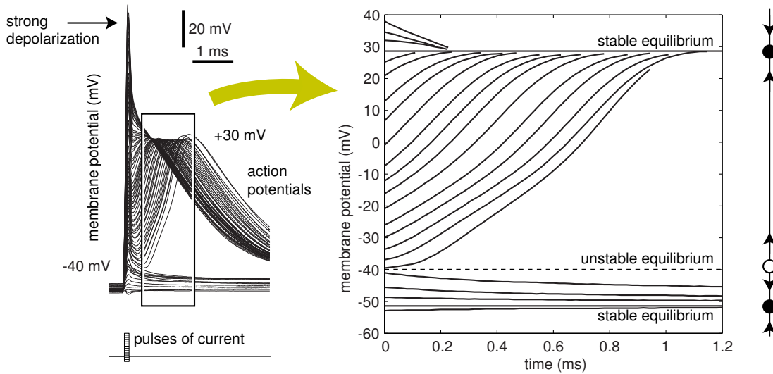
Figure 3.15: Upstroke dynamics of layer 5 pyramidal neuron in vitro (compare with the I_{Na,p} -model (3.5) in Fig. 3.8b).
