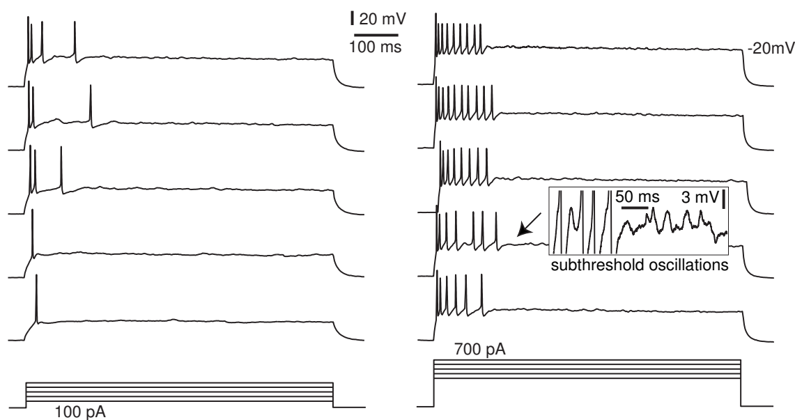
Figure 7.5: Class 3 excitability of a layer 5 pyramidal neuron of rat's visual cortex. The inset shows subthreshold oscillations of membrane potential.
