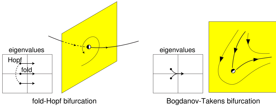
Figure 6.37: Two ways an equilibrium can undergo a saddle-node (fold) and an Andronov-Hopf bifurcations simultaneously.
