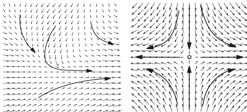
Figure 69: Left: No equilibria. Right: Saddle equilibrium.
