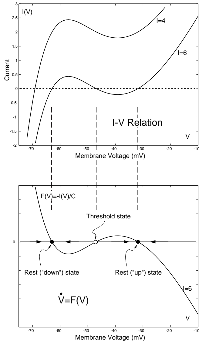
Figure 57: Top: The I-V relations of the non-linear membrane in Fig. 3.38 with I = 4 and I = 6 . Bottom: The right-hand side function F(V) of the I_{K_{ir}} -model (3.11) when I = 6 .
