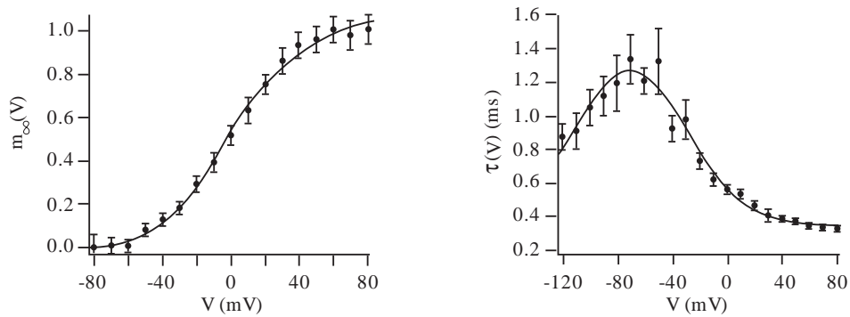
Figure 2.9: The activation function m_\infty(V) and the time constant \tau(V) of the fast transient \text{K}^+ current in the layer 5 neocortical pyramidal neurons (modified from König and Sakmann 2000).
