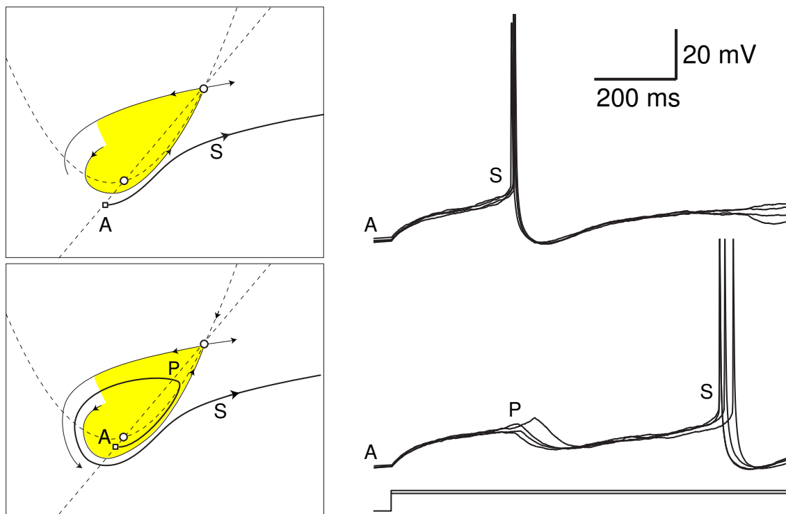
Figure 7.42: Proximity to Bogdanov-Takens bifurcation in layer 5 pyramidal neuron of rat primary visual cortex results in slow subthreshold oscillation before a spike. Shown are hand-drawn phase portrait and in vitro recordings obtained while an automated procedure was testing the neuronal rheobase.
