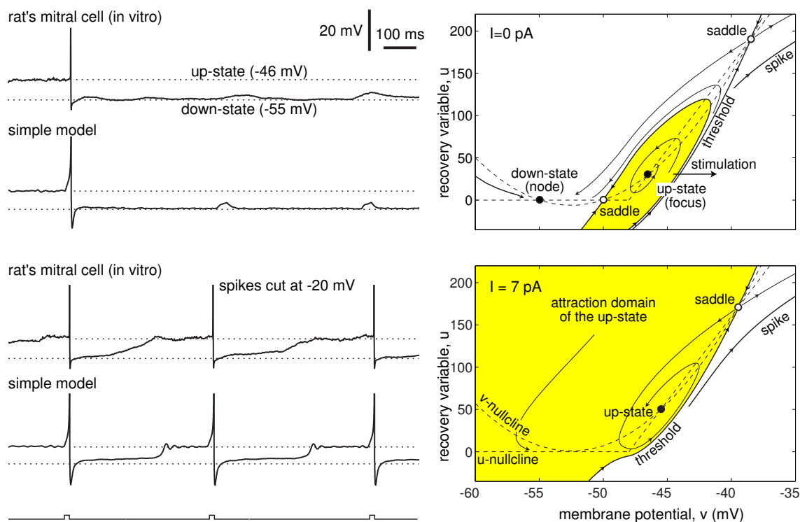
Figure 8.34: Voltage responses of a rat's mitral cell and a simple model from Fig. 8.33 at two different values of the holding current. Right: Phase portraits of somatic compartments show coexistence of stable node (down-state) and stable focus (up-state) equilibria. Spikes are emitted only from the up-state.
