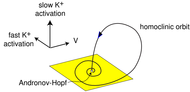
Figure 81: Co-dimension-2 Shilnikov-Hopf bifurcation.
