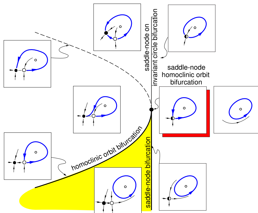
Figure 6.45: Unfolding of saddle-node homoclinic orbit bifurcation.
