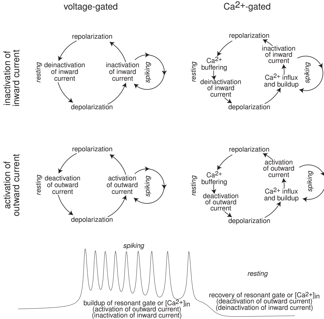
Figure 9.6: Four major classes of bursting models are defined by the slow resonant gating variable that modulates spiking activity.
