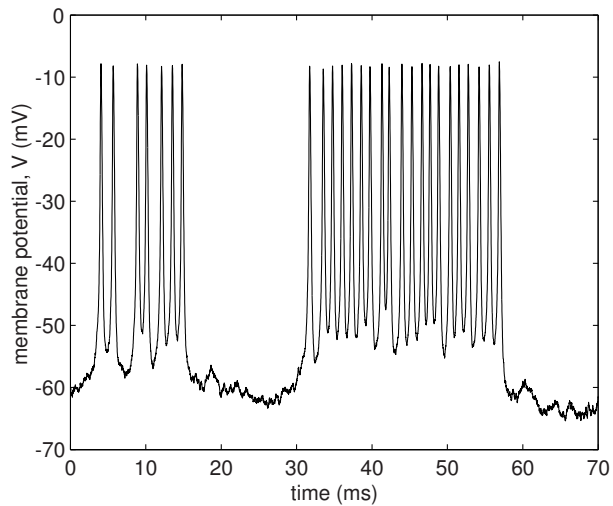
Figure 9.55: Bursting in a two-dimensional I_{Na,p} + I_K -model; see Ex. 3.
