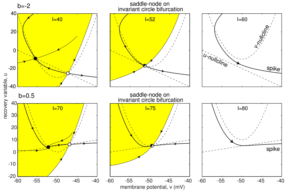
Figure 8.11: Saddle-node on invariant circle bifurcations in the RS neuron model as the magnitude of the injected current I increases.
