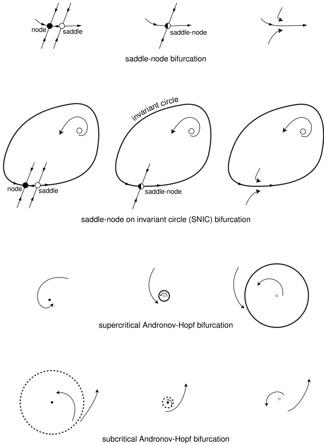
Figure 6.48: Summary of all co-dimension-1 bifurcations of a stable equilibrium (resting state).
