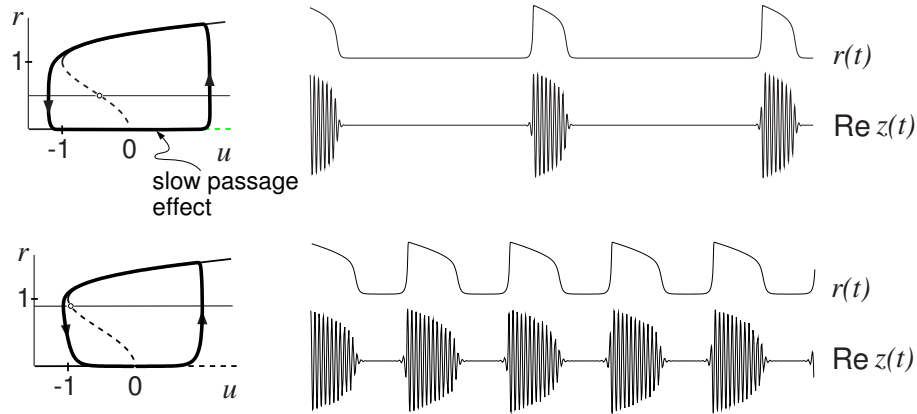
Figure 9.36: Phase portrait and solution of the canonical model (9.11) for \mu = 0.1 , \omega = 3 , and a = 0.25 (top) and a = 0.8 (bottom), where r = |z| is the amplitude of oscillation (modified from Izhikevich 2000).
