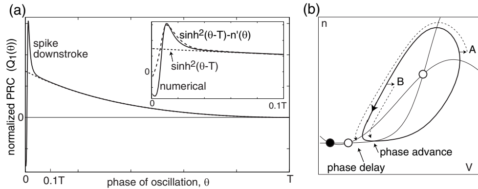
Figure 10.38: (a) Numerically found PRCs of the I_{Na} + I_K -oscillator near saddle-node homoclinic orbit bifurcation (as in Fig. 10.37) using the MATLAB program in Ex. 12. Magnification shows the divergence from the theoretical curve \sinh^2(\vartheta - T) during the spike. (b) A pulsed input during the downstroke of the spike can produce a significant phase delay (pulse A) or advance (pulse B) not captured by the quadratic integrate-and-fire model.
