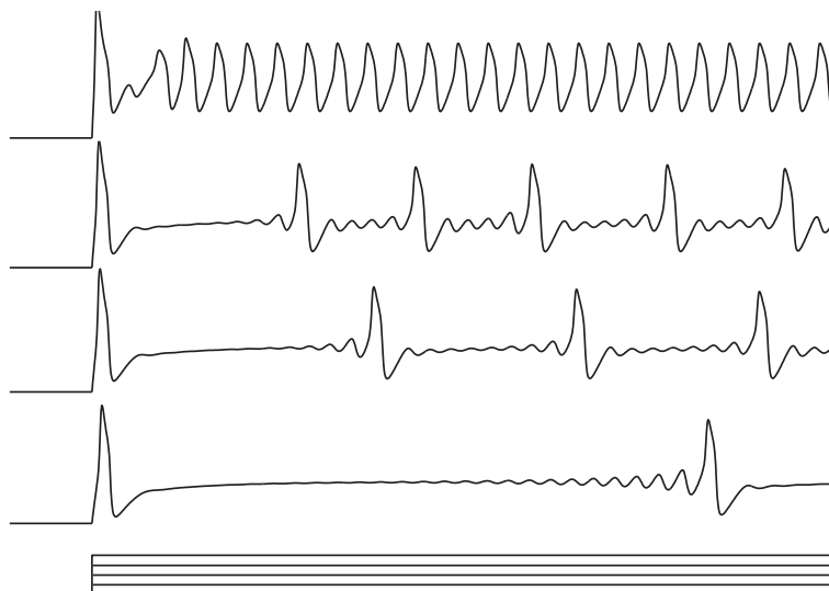
Figure 7.54: Ex. 6: Zero frequency firing near subcritical Andronov-Hopf bifurcation in the I_{Na,p}+I_K -model with parameters as in Fig. 6.16 and a high-threshold slow K^+ current ( g_{K,slow} = 25 , \tau_{K,slow} = 10 ms, n_{\infty,slow}(V) has V_{1/2} = -10 mV and k = 5 mV.)
