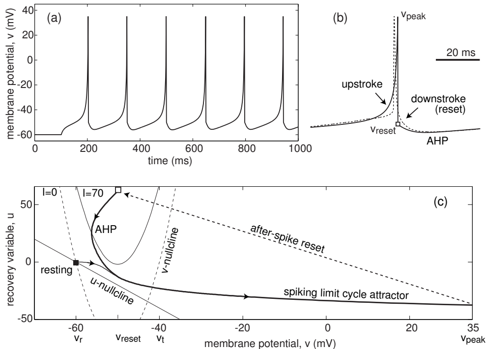
Figure 8.6: (a) Output of the MATLAB code simulating the simple model (8.5, 8.6). (b) Comparison of the simulated (continuous curve) and experimental (dashed curve) voltage traces shows two major discrepancies marked by arrows. (c) Phase portrait of the model.
