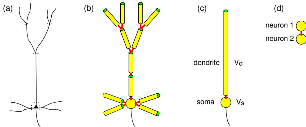
Figure 2.19: Dendritic tree of a neuron (a) is replaced by a network of compartments (b), each modeled by a Hodgkin-Huxley-type model. Two-compartment neuronal model (c) may be equivalent to two neurons coupled via gap junctions (electrical synapse).
