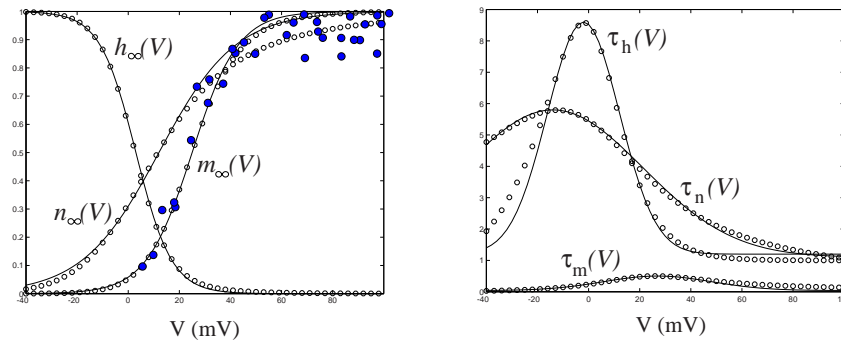
Figure 47: Open dots : The steady-state (in)activation functions and voltage-sensitive time constants in the Hodgkin-Huxley model. Filled dots : steady-state \text{Na}^+ activation function m_\infty(V) in the squid giant axon (experimental results by Hodgkin and Huxley, 1952, Fig. 8). Continuous curves : Approximations by Boltzmann and Gaussian functions. See Ex. 4.
