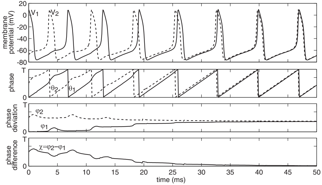
Figure 10.25: The relationship between membrane potential oscillation of two neurons, V_1 (solid) and V_2 (dashed), their phases, phase deviations, and phase difference. Shown simulation of two I_{Na} + I_K -models with parameters as in Fig. 10.3 and coupled symmetrically via gap junctions 0.1(V_j - V_i) (see Sect. 2.3.4).
