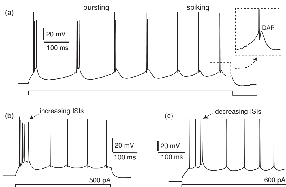
Figure 8.14: (a) bursting and spiking in an IB neuron (layer 5 of somatosensory cortex of a 4 week old rat at 35C; data was kindly provided by Greg Stuart and Maarten Kole). Notice the depolarized after-potential (DAP). (b) IB neuron of a cat (modified from Fig. 2 of Timofeev et al. (2000)). (c) pyramidal neuron of rat's visual cortex. Notice that IB neurons may exhibit bursts with increasing or decreasing inter-spike intervals (ISIs).
