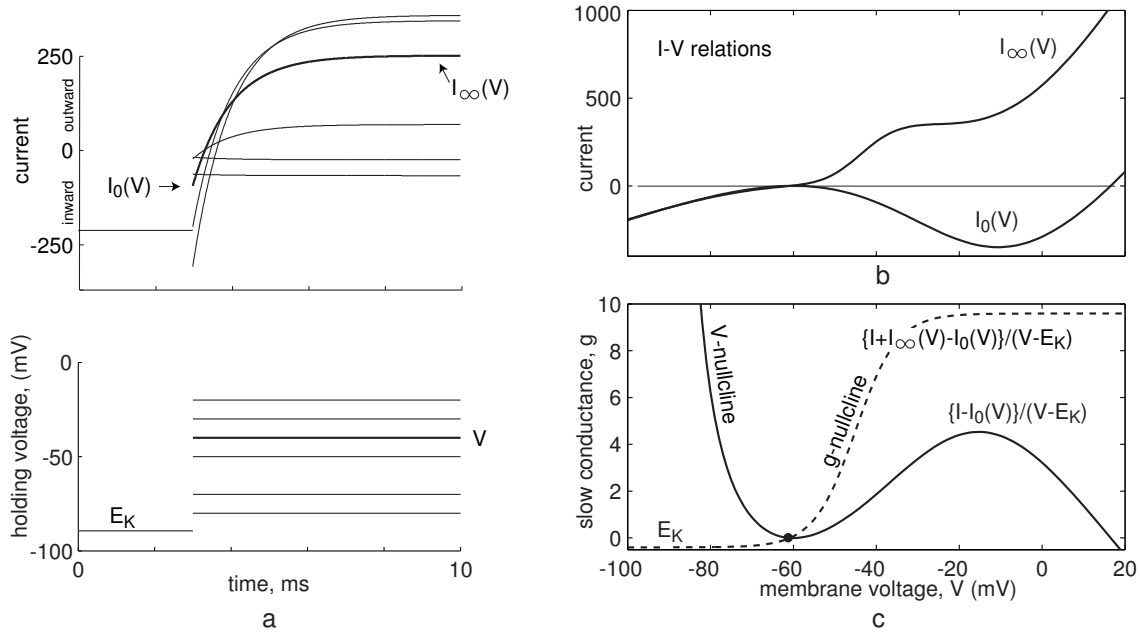
Figure 5.22: Voltage-clamp protocol to measure instantaneous (peak) and steady state current-voltage (I-V) relations. (Shown simulations of the I_{Na,p}+I_K -model from Fig. 5.4b.)
