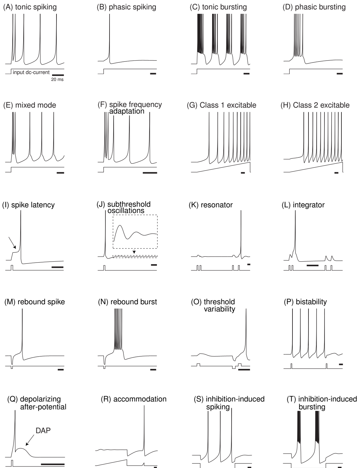
Figure 8.7: Summary of neuro-computational properties exhibited by the simple model; see Ex. 11. The figure is reproduced with permission from www.izhikevich.com . (electronic version of the figure and reproduction permissions are freely available at www.izhikevich.com )
