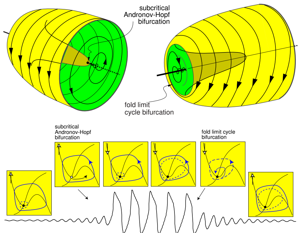
Figure 9.35: “SubHopf/fold cycle” burster: The middle equilibrium corresponding to the resting state loses stability via subcritical Andronov-Hopf bifurcation, and the outer limit cycle attractor corresponding to repetitive spiking disappears via fold limit cycle bifurcation. Top two images are different views of the same 3-D structure.
