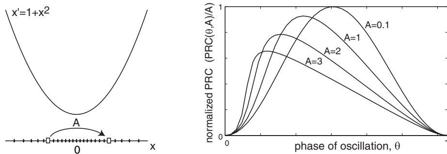
Figure 10.35: The dependence of PRC of the quadratic integrate-and-fire model on the strength of the pulse A .
