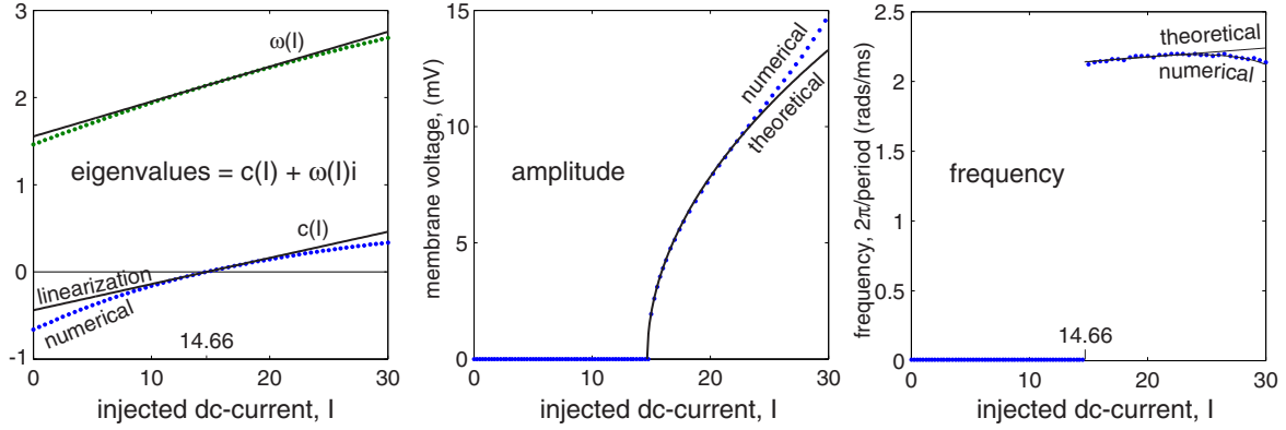
Figure 6.12: Supercritical Andronov-Hopf bifurcation in the I_{Na,p} + I_K -model with low-threshold K^+ current (see Fig. 6.11). Dots — numerical simulation of the full model, continuous curves - analytical results using the topological normal form (6.5, 6.6).
