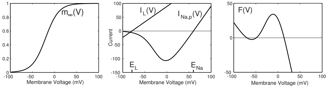
Figure 3.39: The I_{Na,p} -model having leak current ( I_L ) and persistent Na^+ current ( I_{Na,p} ) and described by (3.5) with the right-hand side function F(V) . Parameters: C = 1 , I = 0 , g_L = 1 , E_L = -80 , g_{Na} = 2.25 , E_{Na} = 60 , V_{1/2} = -20 , k = 15 (see Fig. 2.20).
