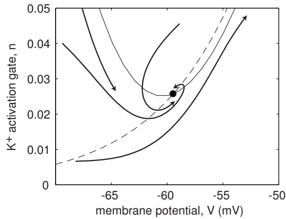
Figure 7.39: Bogdanov-Takens bifurcation in the I_{Na} + I_K -model (4.1, 4.2). Parameters as in Fig. 4.1a, except n_\infty(V) has k = 7 mV and V_{1/2} = -31.64 mV, E_{leak} = -79.42 and I = 5 . Integrator: V_{1/2} = -31 mV and I = 4.3 . Resonator: V_{1/2} = -34 mV and I = 7 .
