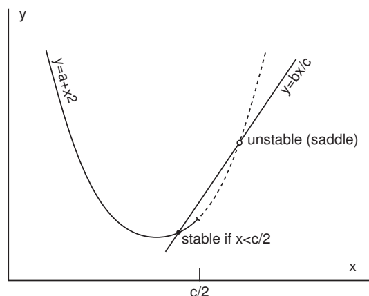
Figure 77: The left equilibrium is stable when x < c/2 ; see Ex. 11.
