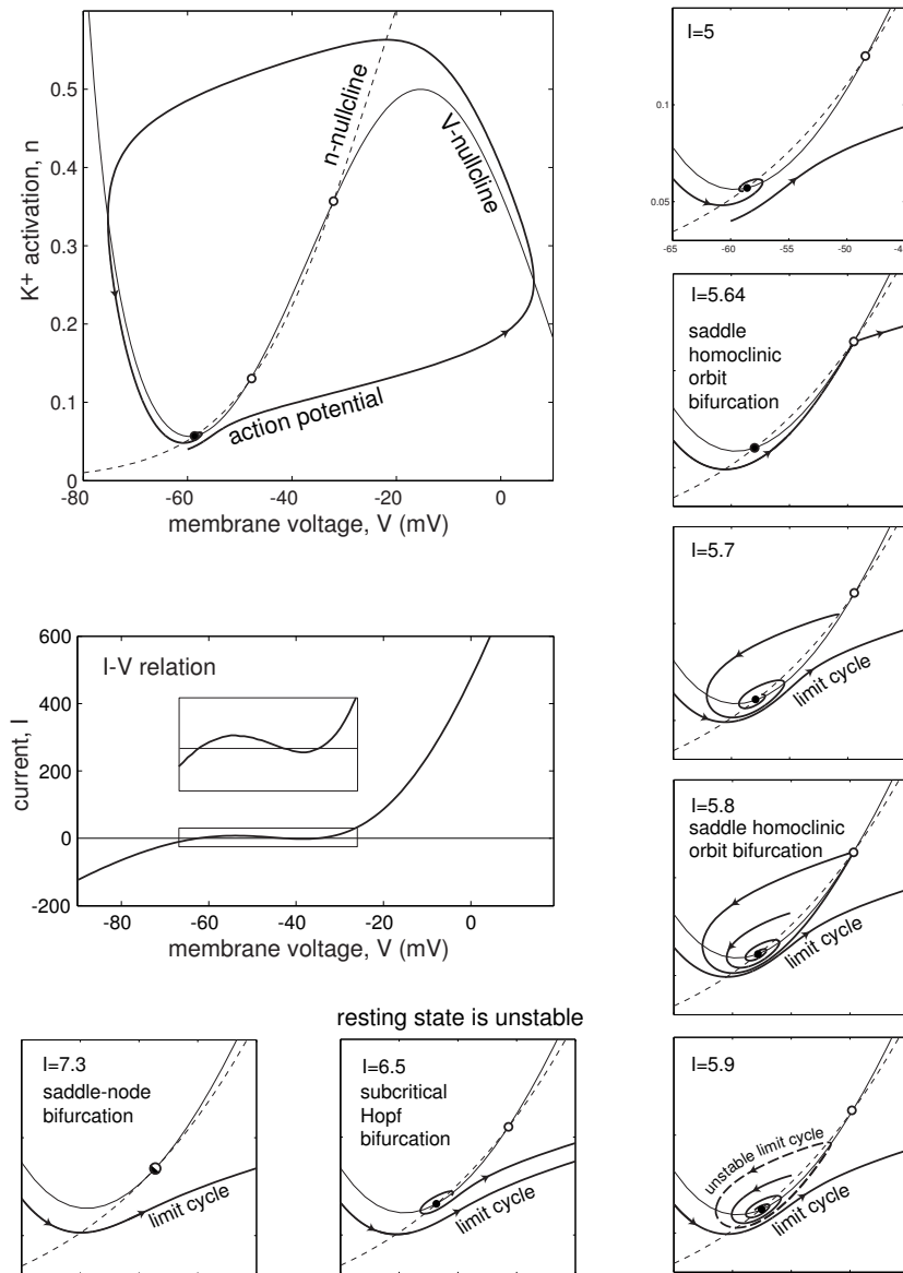
Figure 80: Answer to Ex. 8.
