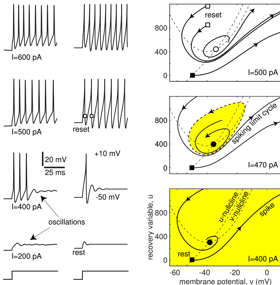
Figure 8.31: Comparison of in vitro recordings of rat's brainstem mes V neuron (from Fig. 7.3) with simulations of the simple model 25\dot{v} = (v + 50)(v + 30) - u + I , \dot{u} = 0.5\{U(v + 50) - u\} , with cubic slow nullcline U(x) = 25x + 0.009x^3 . If v \geq 10 , then v \leftarrow -40 .
