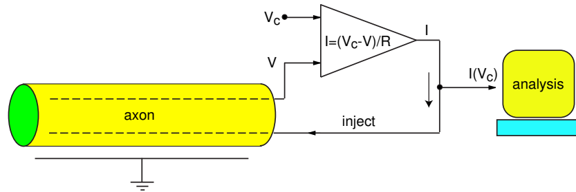
Figure 2.5: Two-wire voltage-clamp experiment on the axon: Top wire is used to monitor the membrane potential V . Bottom wire is used to inject the current I proportional to the difference V_c - V to keep the membrane potential at V_c .
