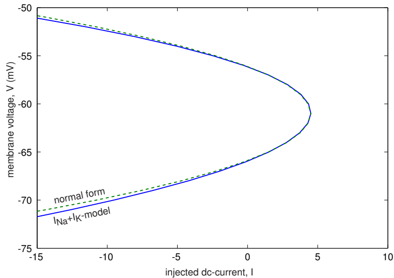
Figure 6.5: Bifurcation diagrams of the topological normal form (6.3) and the I_{Na,p}+I_K -model (4.1, 4.2).
