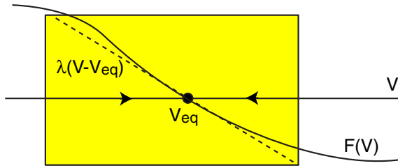
Figure 3.21: Hartman-Grobman theorem: Non-linear system \dot{V} = F(V) is topologically equivalent to the linear one \dot{V} = \lambda(V - V_{\text{eq}}) in the local (shaded) neighborhood of the hyperbolic equilibrium V_{\text{eq}} .
