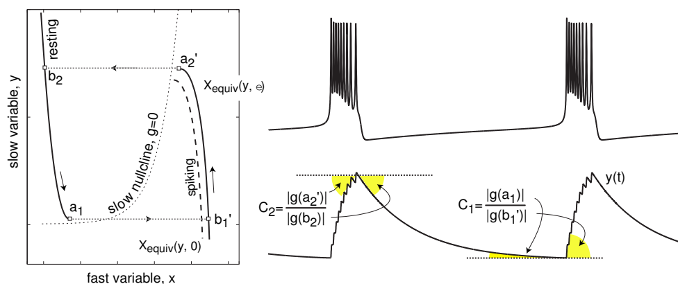
Figure 10.40: Reduction of the I_{Na,p} + I_K + I_{K(M)} -burster to a relaxation oscillator. The slow variable exhibits “scalped” oscillations needed for stability of in-phase burst synchronization. C_1 and C_2 are compression functions at the two jumps.
