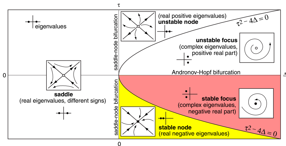
Figure 4.15: Classification of equilibria according to the trace ( \tau ) and the determinant ( \Delta ) of the Jacobian matrix L . Shaded region corresponds to stable equilibria.
