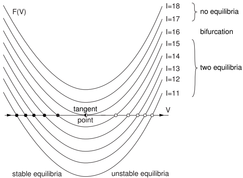
Figure 3.26: Saddle-node bifurcation: While the graph of the function F(V) is lifted up, the stable and unstable equilibria approach each other, coalesce at the tangent point, and then disappear.
