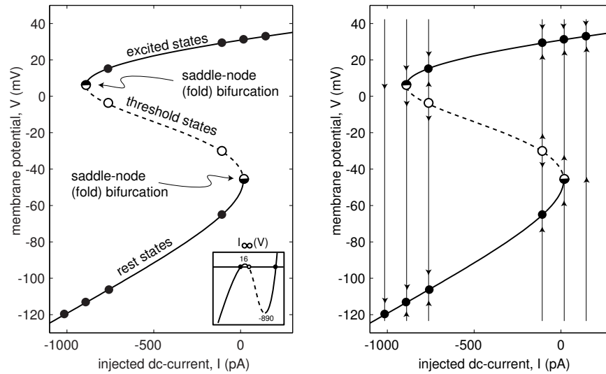
Figure 3.32: Bifurcation diagram of the I_{Na,p} -model (3.5).
