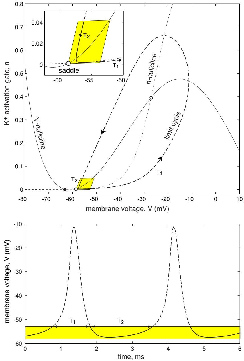
Figure 6.29: The period of limit cycle is T = T_1 + T_2 with T_2 \rightarrow \infty as the cycle approaches the saddle equilibrium. Shown is the I_{Na,p} + I_K -model with I = 3.5 .
