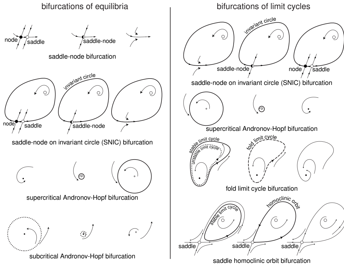
Figure 9.22: Summary of co-dimension-1 bifurcations of equilibria and limit cycles in two-dimensional systems.
