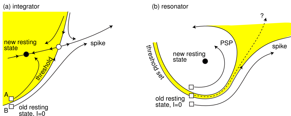
Figure 7.28: Integrators have well-defined rheobase current while resonators may not.
