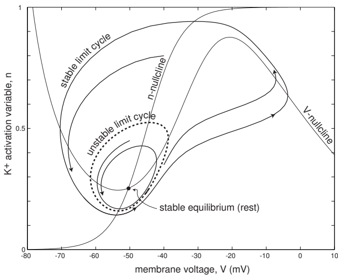
Figure 9.39: Phase portrait of the I_{Na,p}+I_K -model with parameters corresponding to subcritical Andronov-Hopf bifurcation and fold limit cycle bifurcation.
