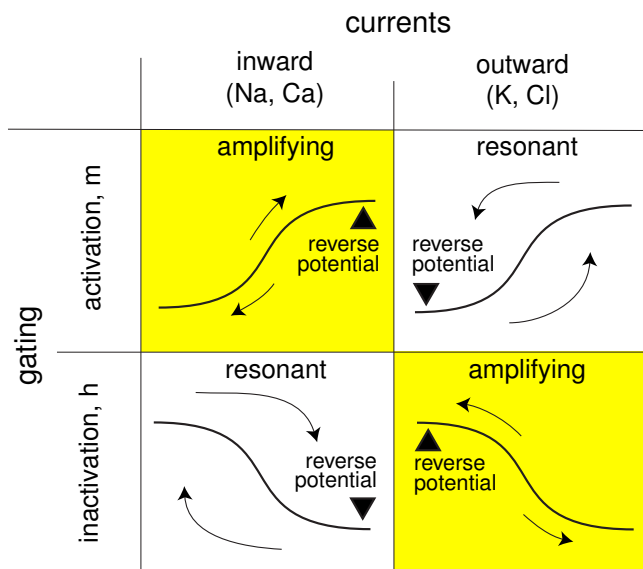
Figure 5.2: Gating variables may be amplifying or resonant depending on whether they represent activation/inactivation of inward/outward currents (compare with Fig. 3.3).
