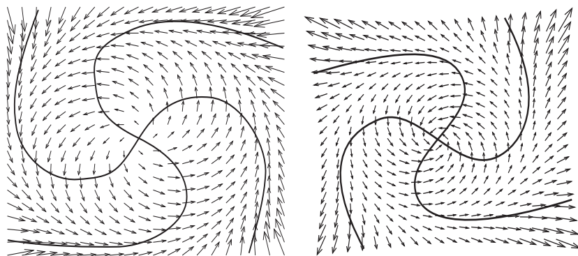
Figure 66: Nullclines of the vector field; see also Fig. 72.
