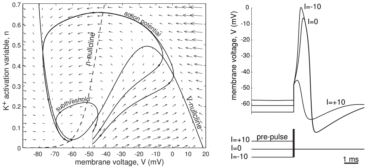
Figure 4.8: Failure to have a fixed value of threshold voltage in the I_{Na,p} + I_K -model (4.1, 4.2).
