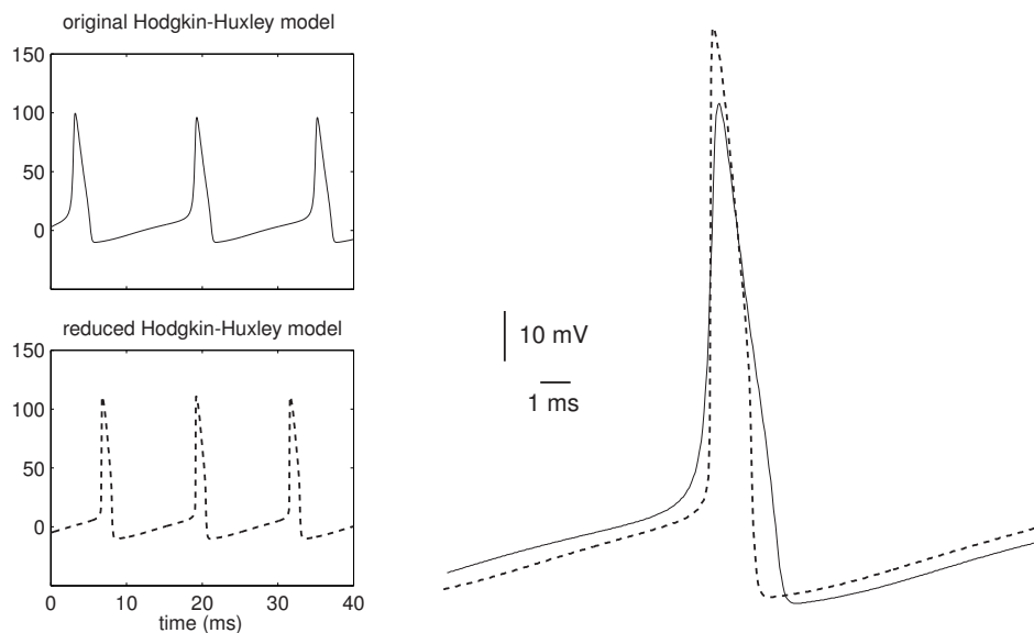
Figure 5.20: Action potentials in the original (top) and reduced (bottom) Hodgkin-Huxley model ( I = 8 ).
