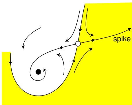
Figure 1.16: Phase portrait of a system near Bogdanov-Takens bifurcation that corresponds to the transition from integrator to resonator mode.
