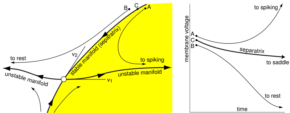
Figure 4.24: Stable and unstable manifolds to a saddle. Eigenvectors v_1 and v_2 correspond to positive and negative eigenvalues, respectively.
