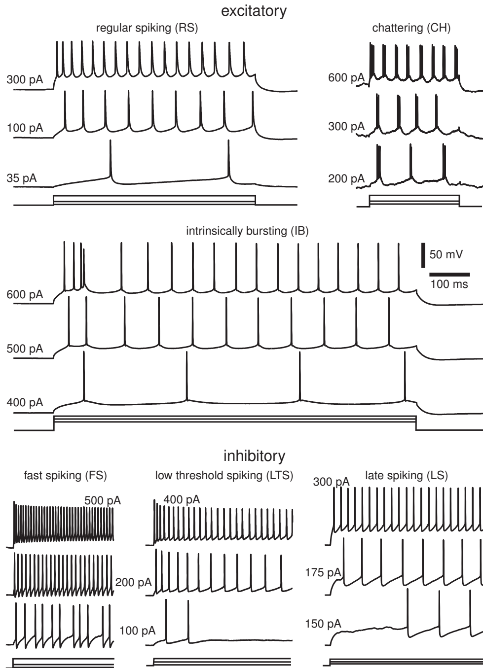
Figure 8.8: Six most fundamental classes of firing patterns of neocortical neurons in response to pulses of depolarizing dc-current. RS and IB are in vitro recordings of pyramidal neurons of layer 5 of primary visual cortex of a rat, CH was recorded in vivo in cat's visual cortex (area 17, data provided by D. McCormick). FS was recorded in vitro in rat's primary visual cortex, LTS was recorded in vitro in layer 4 or 6 of rat's barrel cortex (data provided by B. Connors). LS was recorded in layer 1 of rat's visual cortex (data provided by S. Hestrin). All recordings are plotted on the same voltage and time scale, and the data are available on the author's webpage ( www.izhikevich.com ).
