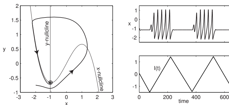
Figure 9.59: Phase portrait of the system in Ex. 12 shows that there is only one stable equilibrium for any value of I . Yet, the system bursts when I is periodically modulated.
