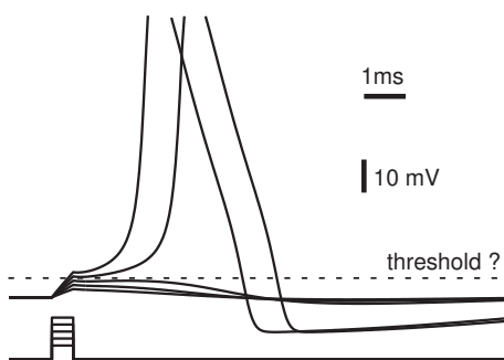
Figure 7.25: Finding threshold in Hodgkin-Huxley model.
