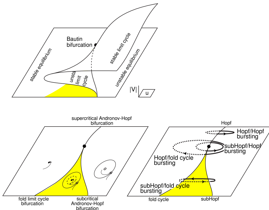
Figure 9.41: A neural system near co-dimension-2 Bautin bifurcation (central dot) can exhibit 4 different types of fast-slow bursting, depending on the trajectory of the slow variable u \in \mathbb{R}^2 in the parameter space. The “subHopf/fold cycle” bursting occurs via a hysteresis loop and requires only one slow variable. Solid (dotted) lines correspond to spiking (resting) regimes (modified from Izhikevich 2000).
