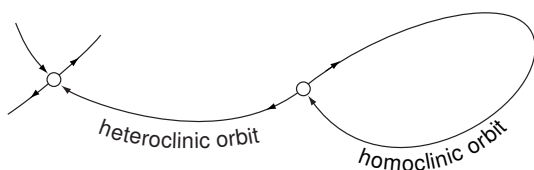
Figure 4.25: Heteroclinic orbit starts and ends at different equilibria. Homoclinic orbit starts and ends at the same equilibrium.
