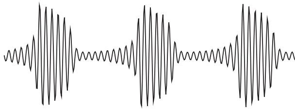
Figure 9.60: A cycle-cycle bursting: The resting state is not an equilibrium, but a small-amplitude limit cycle attractor.
