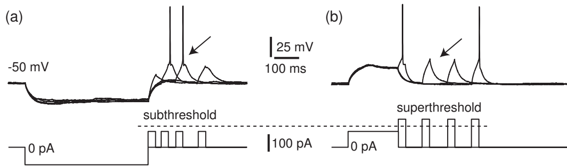
Figure 7.49: Post-inhibitory facilitation (a) and post-excitatory depression (b) in a layer 5 pyramidal neuron (IB type) of rat's visual cortex having slow conductances ( in vitro recording).
