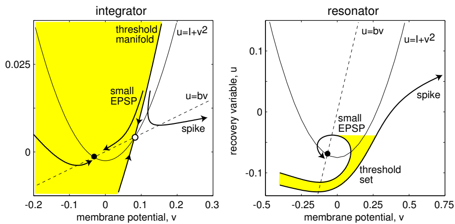
Figure 8.5: Simple model (8.3, 8.4) can be an integrator or a resonator. Compare with Fig. 7.27.
