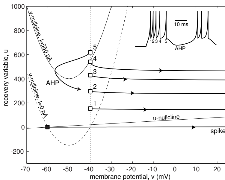
Figure 8.19: Phase portrait of the simple model in Fig. 8.18 exhibiting CH firing pattern.
