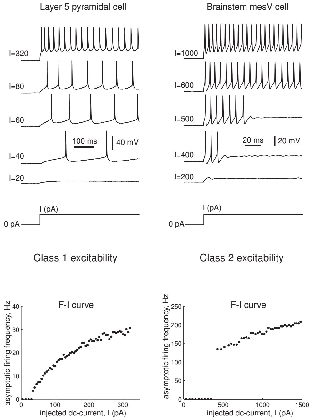
Figure 7.3: Top : Typical responses of membrane potentials of two neurons to steps of dc-current of various magnitudes I . Bottom : Corresponding frequency-current (F-I) relations are qualitatively different. Shown are recordings of layer 5 pyramidal neurons from rat's primary visual cortex (left) and mesV neuron from rat's brainstem (right). Asymptotic frequency is 1000/T_\infty , where T_\infty is taken to be interval between the last two spikes in a long spike train.
