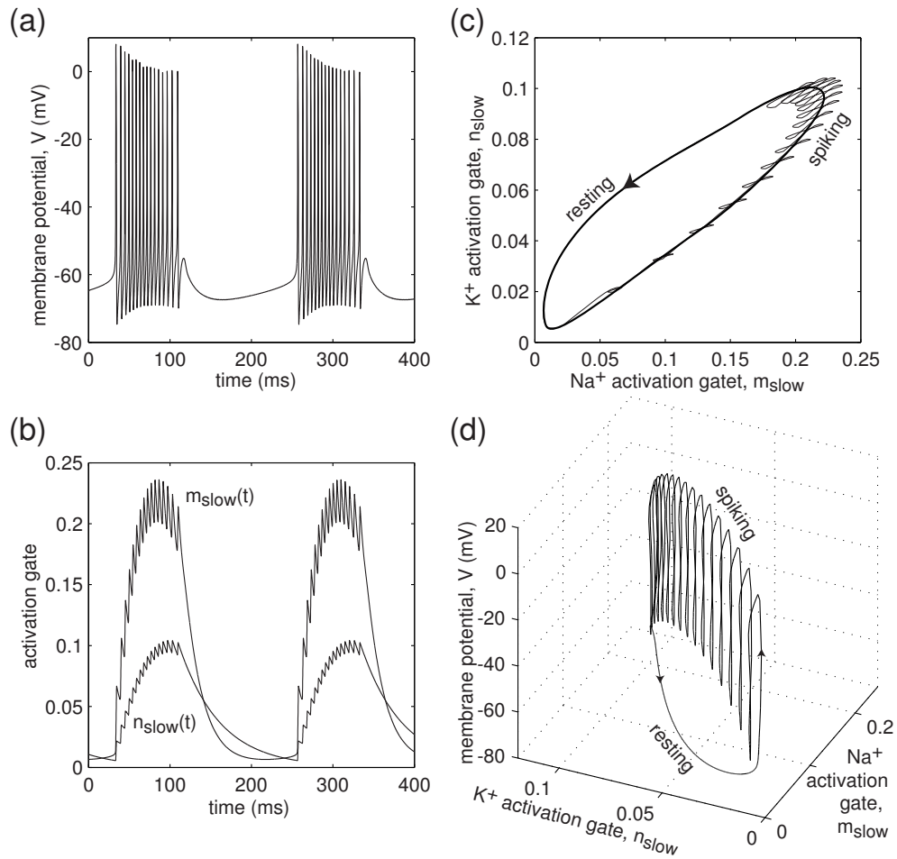
Figure 9.33: “Circle/circle” bursting in the I_{Na,p} + I_K + I_{Na,slow} + I_{K(M)} -model. Parameters of the fast I_{Na,p} + I_K -subsystem are the same as in Fig. 4.1a with I = 5 . Slow Na^+ current has V_{1/2} = -40 mV, k = 5 mV, g_{Na,slow} = 3 , \tau_{Na,slow}(V) = 20 ms. Slow K^+ current has V_{1/2} = -20 mV, k = 5 mV, g_{K(M)} = 20 , \tau_{K(M)}(V) = 50 ms.
