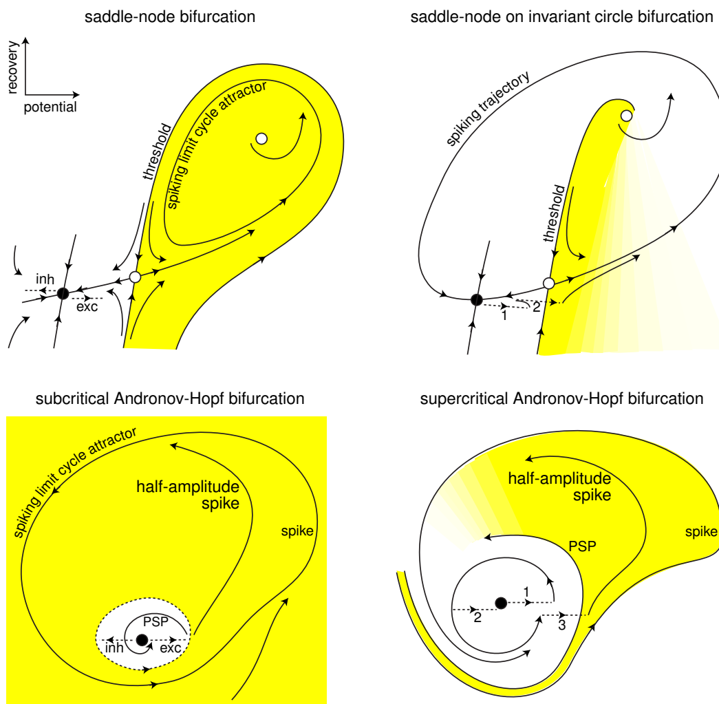
Figure 1.15: The geometry of phase portraits of excitable systems near 4 bifurcations can explain many neuro-computational properties (see Sect. 1.2.4 for detail).
