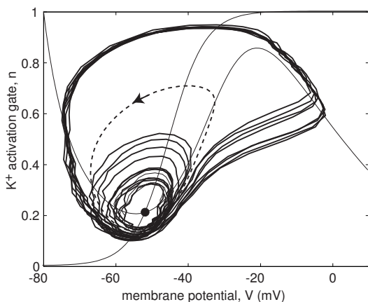
Figure 84: Noise-induced bursting in two-dimensional system; See Ex. 2.
