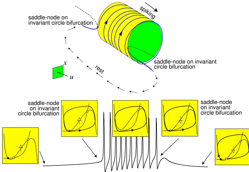
Figure 9.30: “Circle/circle” bursting: The resting state disappears via saddle-node on invariant circle bifurcation and the spiking limit cycle disappears via saddle-node on invariant circle bifurcation.
