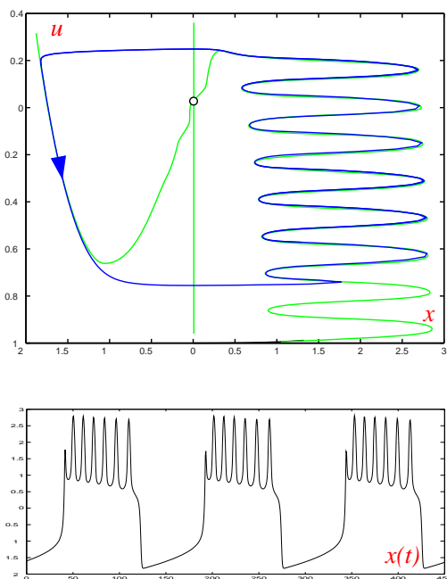
Figure 83: Solution to Ex. 1. Nullclines, hedgehog limit cycle and a bursting solution of a planar system (modified from Izhikevich 2000).
