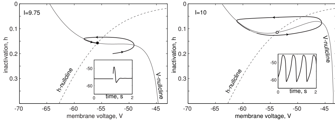
Figure 5.10: Rest and sustained subthreshold oscillations in the I_h + I_{K_{ir}} -model. Parameters: E_K = -80 mV, E_h = -43 mV, E_L = -50 mV, g_{K_{ir}} = 4 , g_h = 0.5 , g_L = 0.44 . h -current is the same as in the previous section, except V_{1/2} = -65 mV. Instantaneous I_{K_{ir}} has V_{1/2} = -76 mV and k = -11 .
