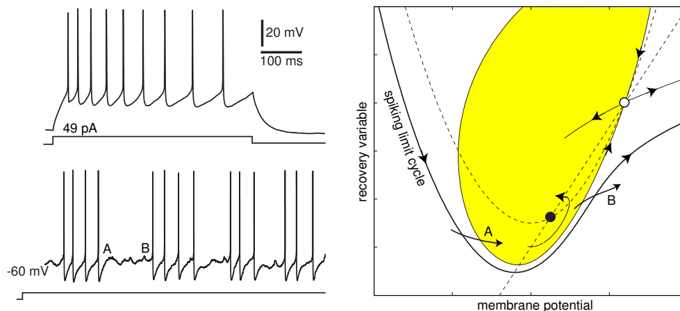
Figure 8.13: Stuttering behavior of an RS neuron (data were provided by Dr. Klaus M. Stiefel, P28-36 adult mouse, coronal slices, 300\mu\text{m} , layer II/III pyramid, visual cortex).
