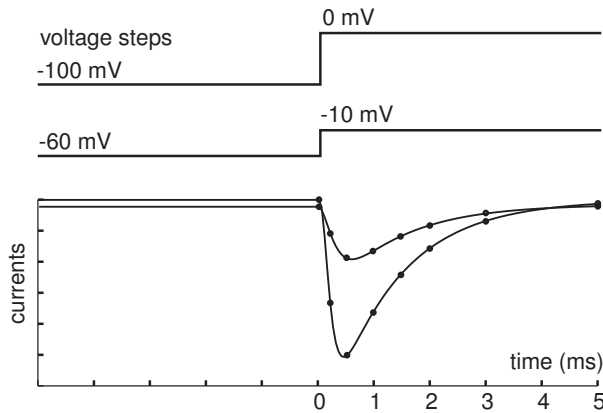
Figure 2.23: Current traces corresponding to voltage steps of various amplitudes; see Ex. 6.
