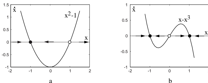
Figure 52: Phase portraits of the systems (a) \dot{x} = -1 + x^2 , (b) \dot{x} = x - x^3 .
