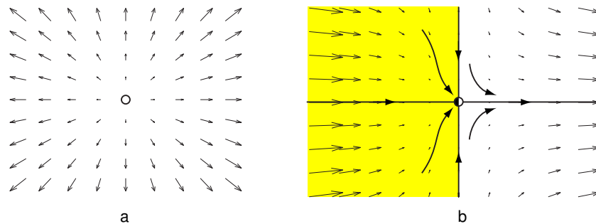
Figure 4.14: Unstable equilibria.
