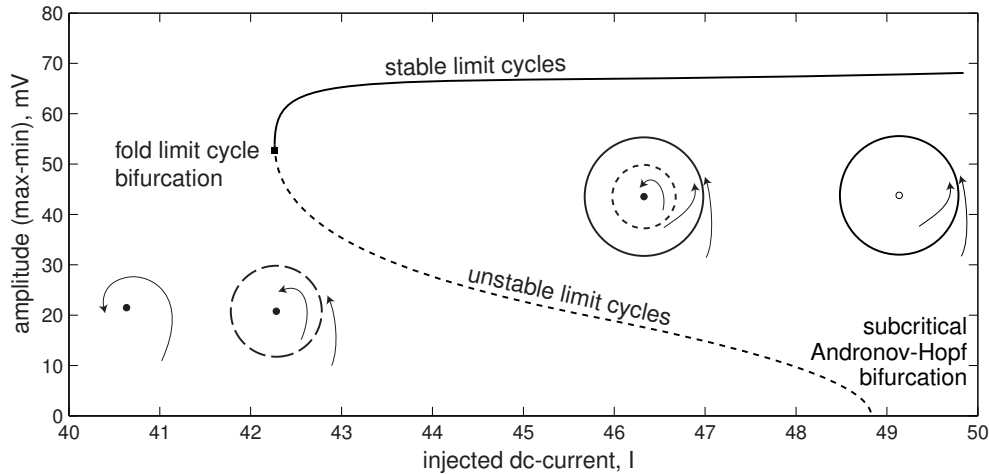
Figure 6.24: Bifurcation diagram of the I_{Na,p}+I_K -model. Parameters as in Fig. 6.16.
