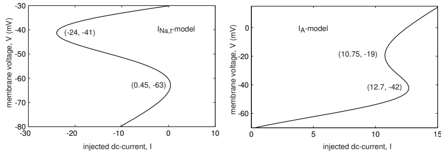
Figure 79: The saddle-node bifurcation diagrams of the I_{Na,t} - and I_A -minimal models.
