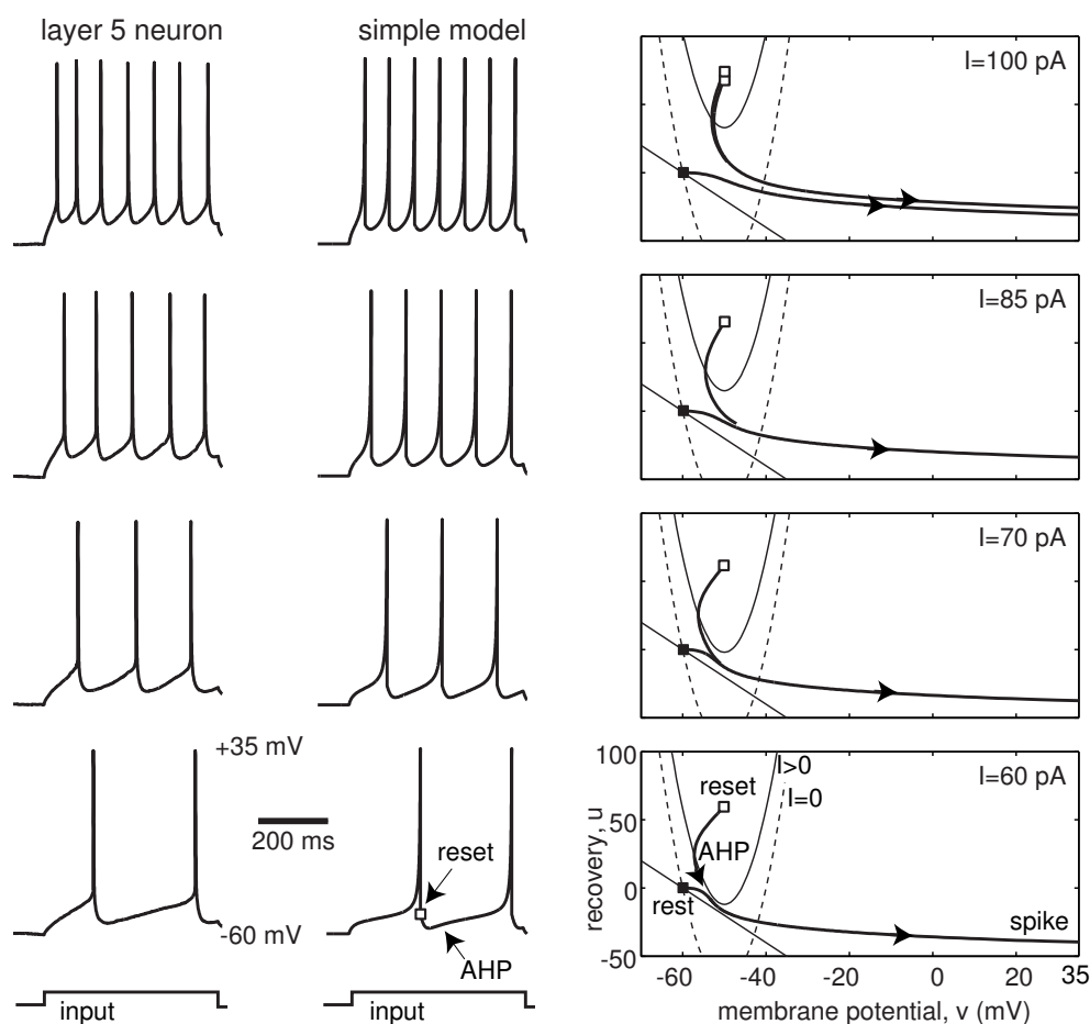
Figure 8.9: Comparison of in vitro recordings of a regular spiking (RS) pyramidal neurons with simulations of the simple model 100\dot{v} = 0.7(v + 60)(v + 40) - u + I , \dot{u} = 0.03\{-2(v + 60) - u\} , if v \geq +35 , then v \leftarrow -50 , u \leftarrow u + 100 .
