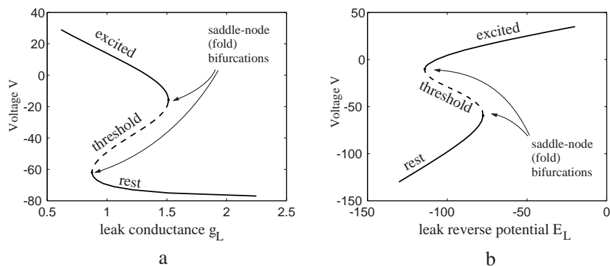
Figure 56: Bifurcation diagrams of the I_{Na,p} -model (3.5) with bifurcation parameters (a) g_L and (b) E_L (see Chap. 3, Ex. 11).
