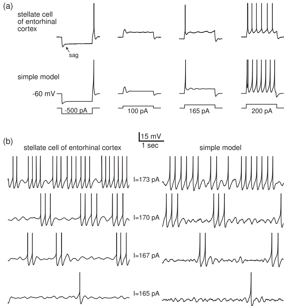
Figure 8.32: Comparison of in vitro recordings of stellate neurons of rat's entorhinal cortex with simulations of the simple model 200\dot{v} = 0.75(v + 60)(v + 45) - u + I , \dot{u} = 0.01\{15(v + 60) - u\} , if v \geq 30 , then v \leftarrow -50 . (a) Responses to steps of dc-current. (b) Subthreshold oscillations and occasional spikes at various levels of injected dc-current. Weak noise was added to simulations to unmask subthreshold oscillations. (Data were kindly provided by Brian Burton and John A. White. All recordings are from the same neuron except steps of -500 pA and 200 pA were recorded from a different neuron. Spikes are cut at 0 mV.)
