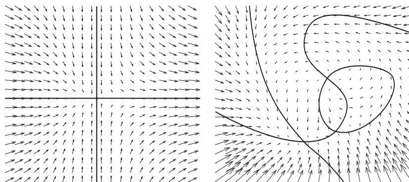
Figure 67: Nullclines of the vector field; see also Fig. 73.
