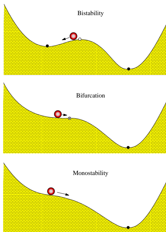
Figure 3.22: Mechanistic illustration of a bifurcation as a change of the landscape.
