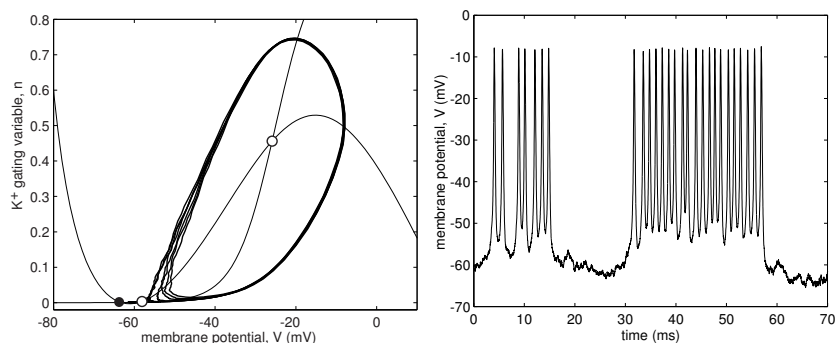
Figure 85: Noise-induced bursting a two-dimensional system with co-existence of an equilibrium and a limit cycle attractor; See Ex. 3.
