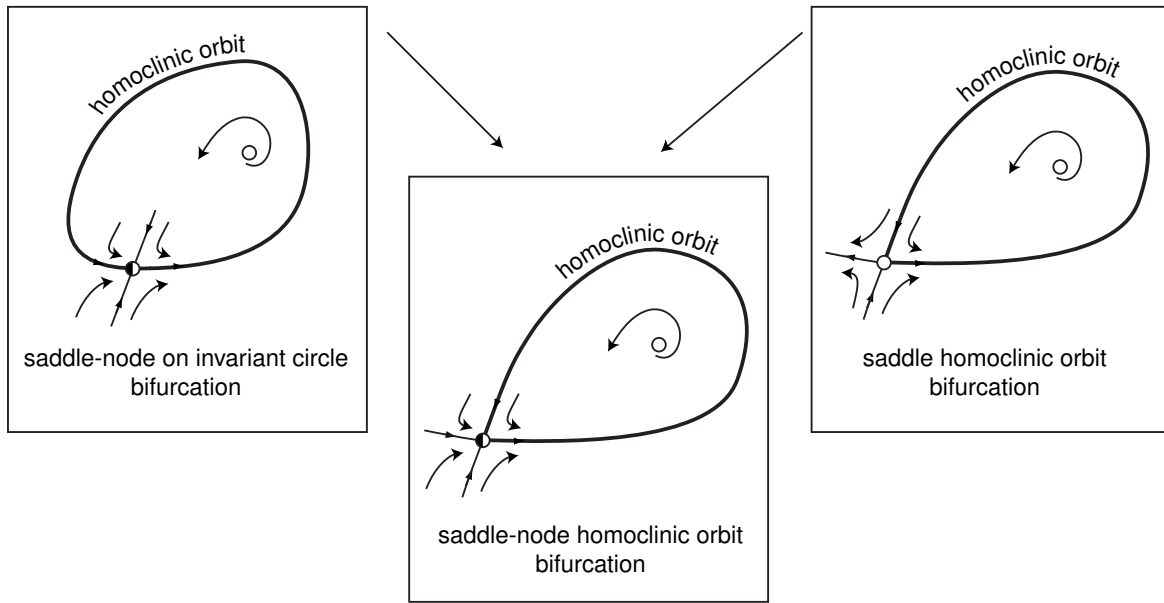
Figure 6.43: Saddle-node homoclinic orbit bifurcation occurs when a systems undergoes a saddle-node on invariant circle and saddle homoclinic orbit bifurcations simultaneously.
