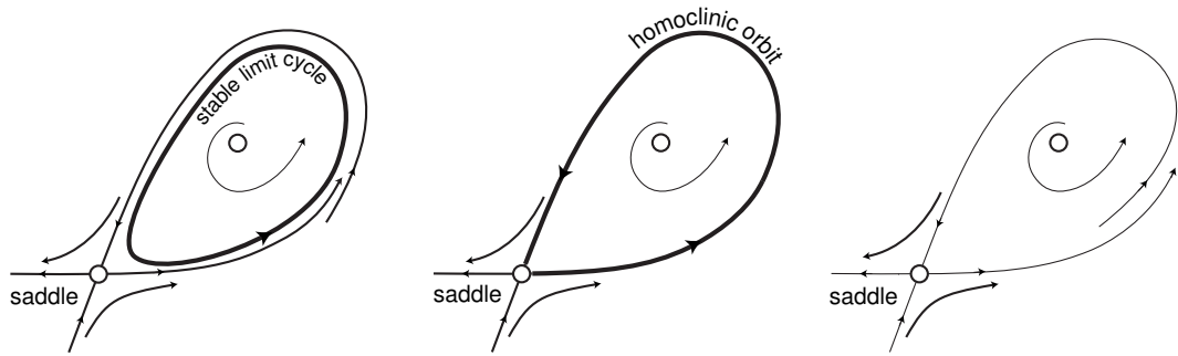
a. supercritical saddle homoclinic orbit bifurcation
