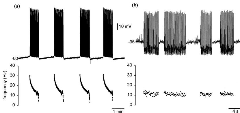
Figure 9.48: The instantaneous spike frequency of a trigeminal motor neuron (a) and trigeminal interneuron (b) of a rodent (modified from Del Negro et al. 1998).
