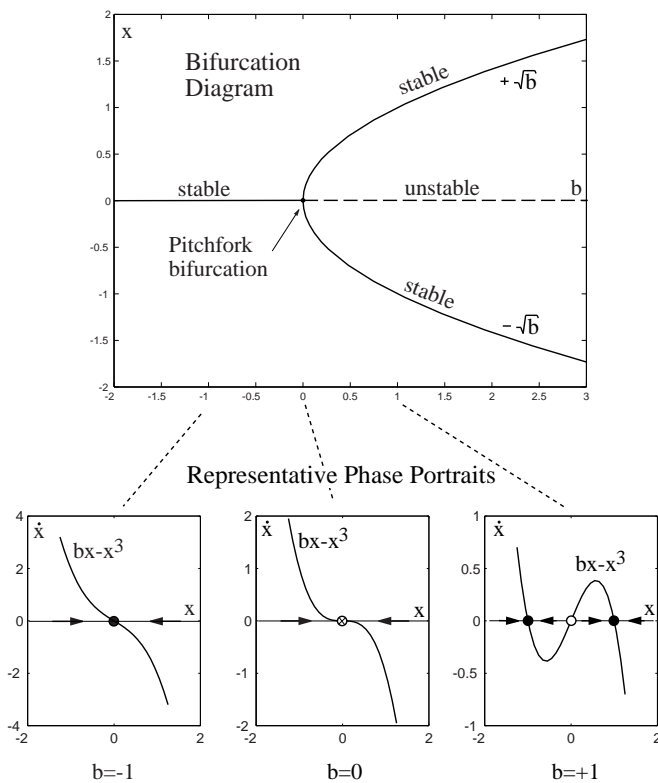
Figure 55: Pitchfork bifurcation diagram and representative phase portraits of the system \dot{x} = bx - x^3 (see Chap. 3, Ex. 8).
