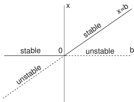
Figure 6.52: Transcritical bifurcation in \dot{x} = x(b - x) .
