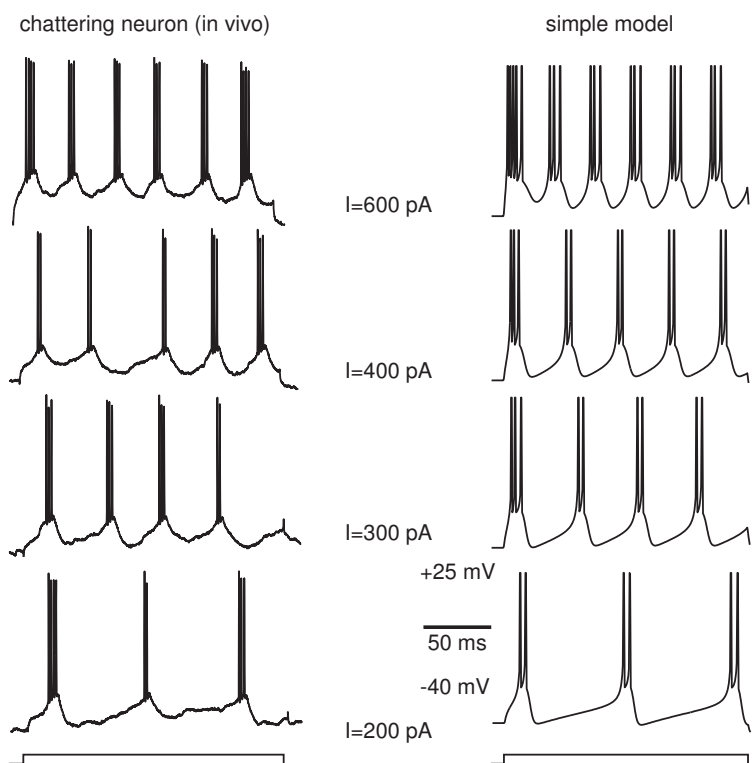
Figure 8.18: Comparison of in vivo recordings from cat's primary visual cortex with simulations of the simple model 50\dot{v} = 1.5(v+60)(v+40) - u + I , \dot{u} = 0.03\{(v+60) - u\} , if v \geq +25 , then v \leftarrow -40 , u \leftarrow u + 150 . Data were kindly provided by D. McCormick, and it is available on the author's webpage.
