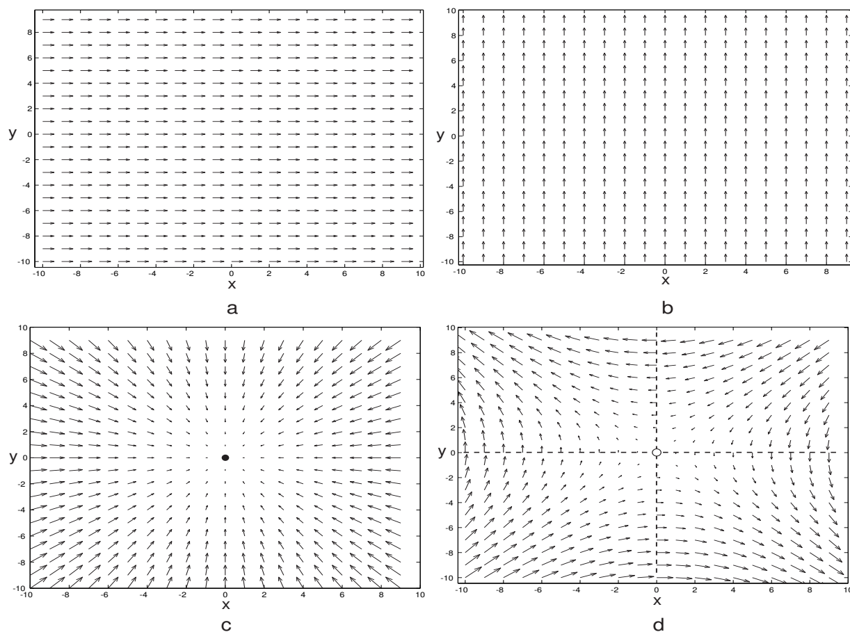
Figure 4.3: Examples of vector fields.
