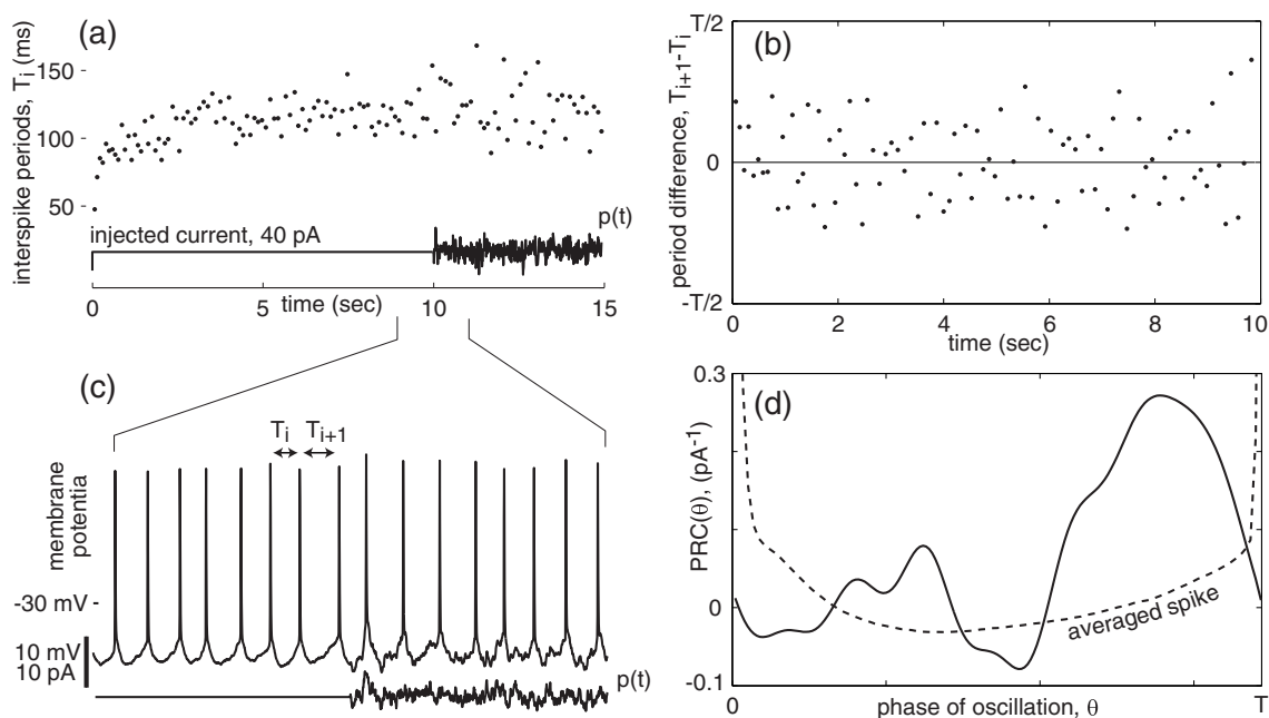
Figure 10.24: Measuring the infinitesimal PRC experimentally in layer 5 pyramidal neuron of mouse visual cortex. (a) Interspike periods in response to the injection of dc-current. (b) Differences between successive periods. (c) Spiking 1 second before and after the noisy current p(t) is injected. (d) Infinitesimal PRC of the neuron (continuous curve) obtained from 40 cycles and the MATLAB program in Ex. 13 (first 8 Fourier terms). Averaged voltage trace during the spike (dotted curve) is plotted for reference.
