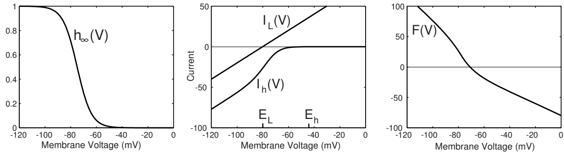
Figure 3.41: The I_h -model having leak current ( I_L ) and “hyperpolarization-activated” inward current I_h and described by (3.13). Parameters: C = 1 , g_L = 1 , E_L = -80 , g_h = 1 , E_h = -43 , V_{1/2} = -75 , k = -5.5 (Huguenard and McCormick 1992).
