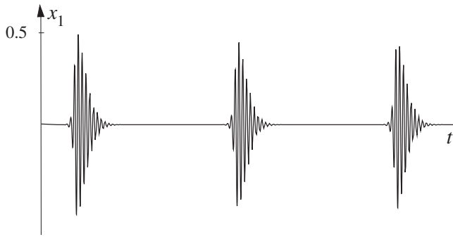
Figure 9.57: Hopf/Hopf bursting without co-existence of attractors; see Ex. 6 (modified from Hoppensteadt and Izhikevich 1997).
