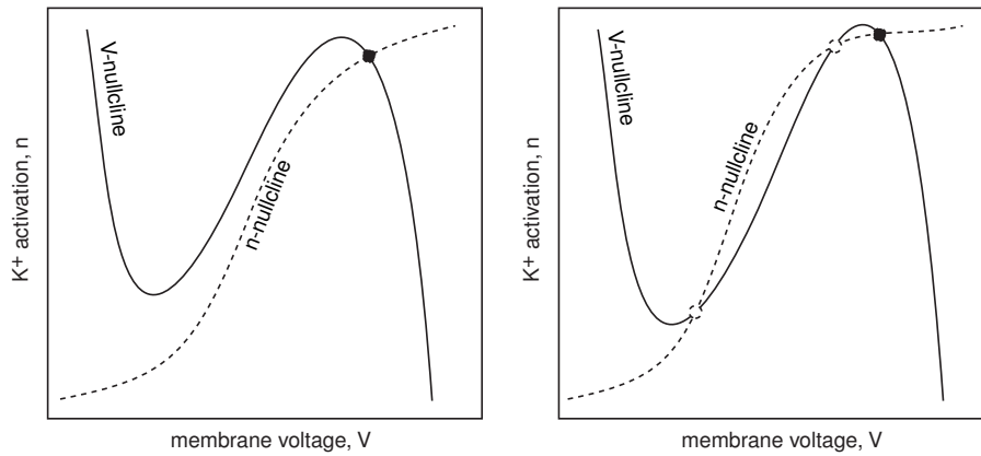
Figure 78: Answer to Ex. 2.
