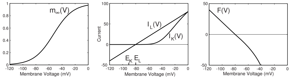
Figure 3.40: The I_K -model having leak current ( I_L ) and persistent K^+ current ( I_K ) and described by (3.12). Parameters: C = 1 , g_L = 1 , E_L = -80 , g_K = 1 , E_K = -90 , V_{1/2} = -53 , k = 15 (see Fig. 2.20).
