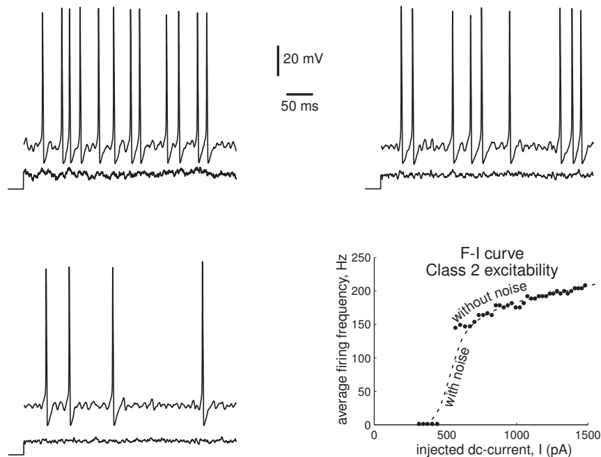
Figure 7.12: Examples of noise-induced low-frequency firings of Class 2 excitable system. The F-I curve may look like the one for Class 1 excitability. Shown are recordings of brainstem mesV neuron.
