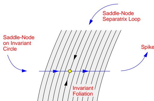
Figure 96: A small neighborhood of the saddle-node point can be invariantly foliated by stable submanifolds.
