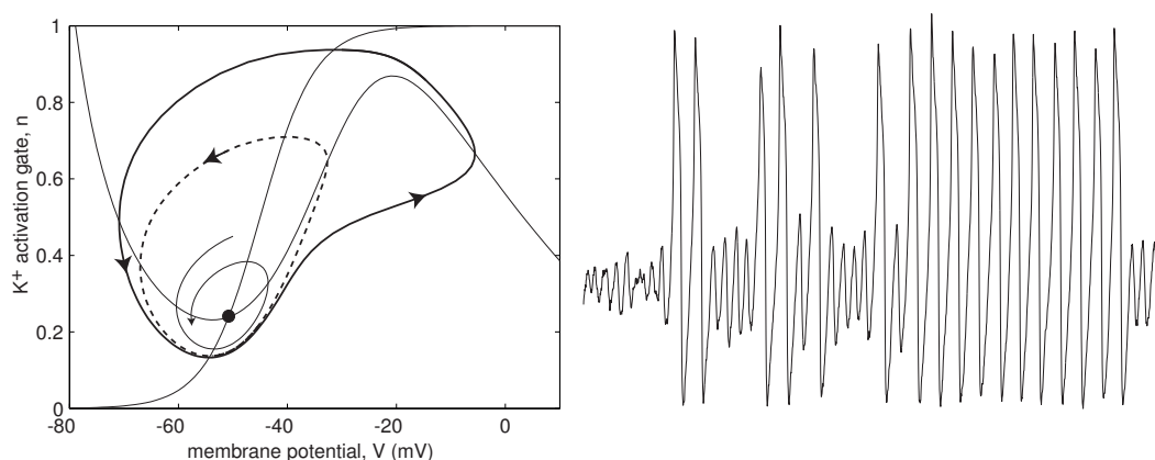
Figure 9.54: Bursting in two-dimensional I_{Na,p}+I_K -model with parameters as in Fig. 6.16 and I = 43 .
