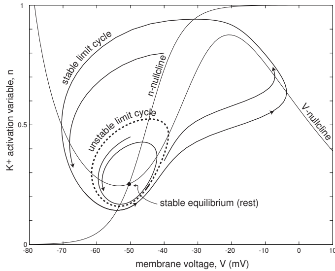
Figure 6.14: Phase portrait of the I_{Na,p} + I_K -model: Unstable limit cycle (dashed circle) is often surrounded by a stable one (solid circle) in two-dimensional neuronal models.
