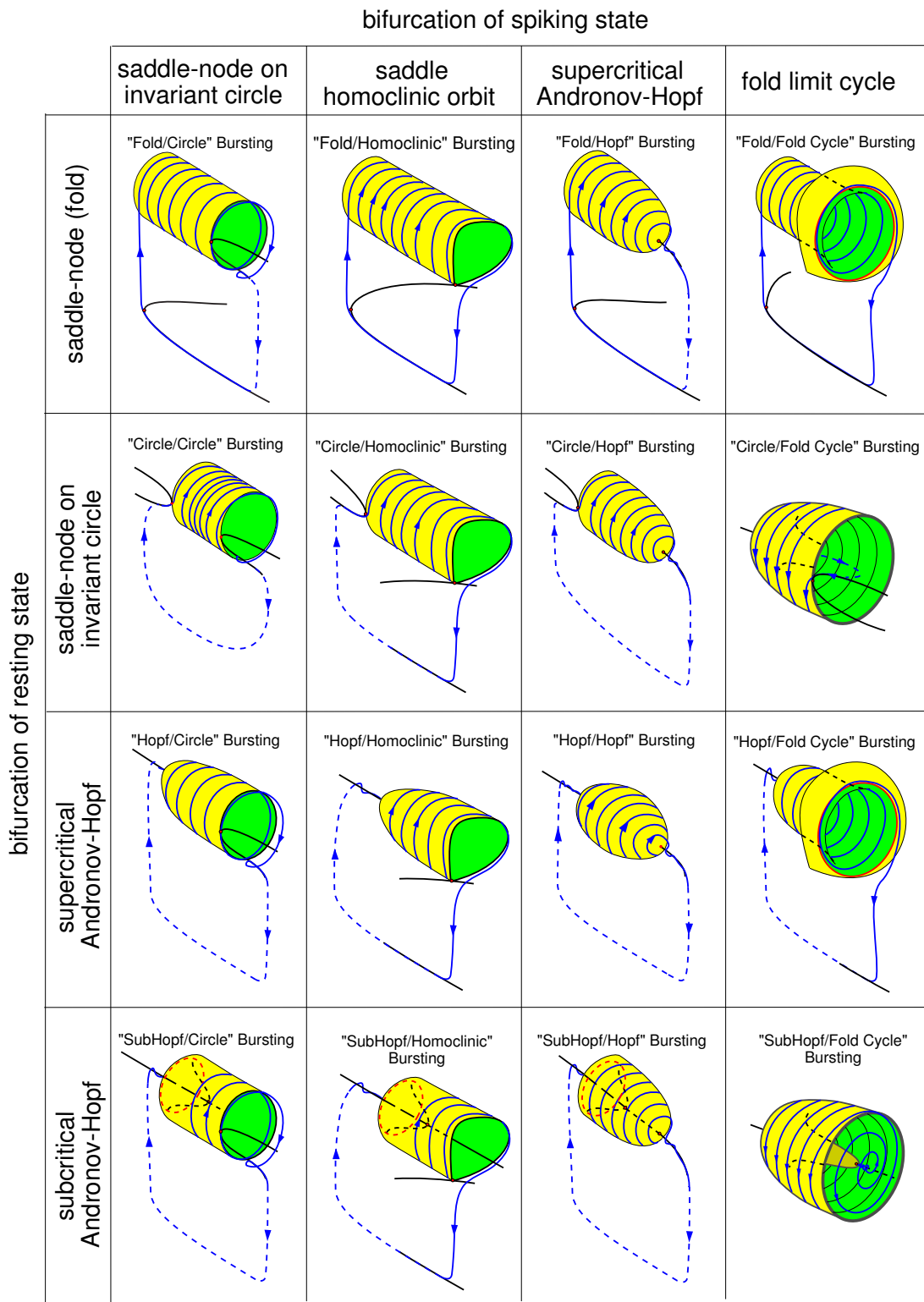
Figure 9.24: Examples of “2+1” point-cycle fast-slow co-dimension-1 bursters of hysteresis-loop type (modified from Izhikevich 2000). Dashed chains of arrows show transitions that might involve other bifurcations not relevant to the bursting type.
