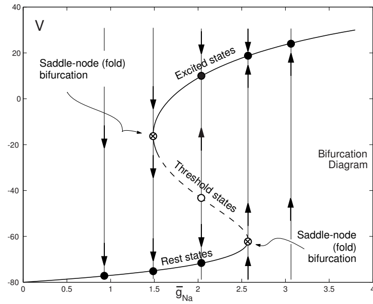
Figure 61: Answer to Ex. 13: Bifurcation diagram of the I_{Na,p} -model (3.5).
