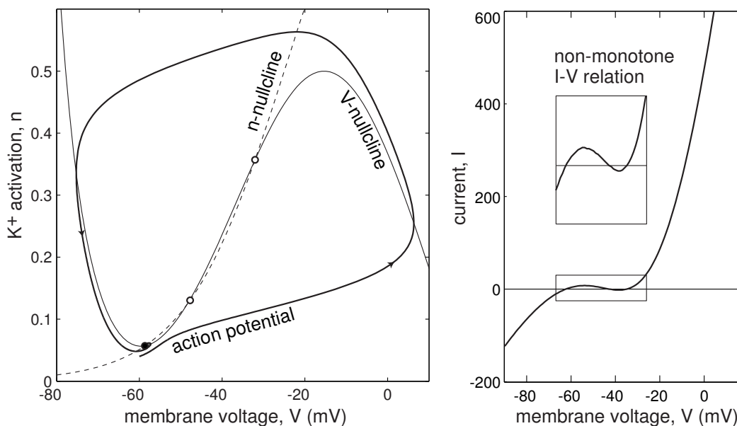
Figure 6.53: Ex. 8: This I_{Na,p} + I_K -model has a non-monotonic I-V relation, yet the resting state becomes unstable via Andronov-Hopf bifurcation before disappearing via saddle-node bifurcation. Parameters as in Fig. 4.1a (Chapter 4) except that E_{leak} = -78 mV and n_{\infty}(V) has k = 12 mV.
