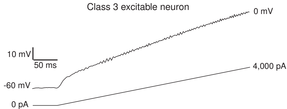
Figure 7.7: Class 3 excitable brainstem mesV neuron does not fire in response to a ramp-current, even though the injected current is stronger than the one in Fig. 7.4.
