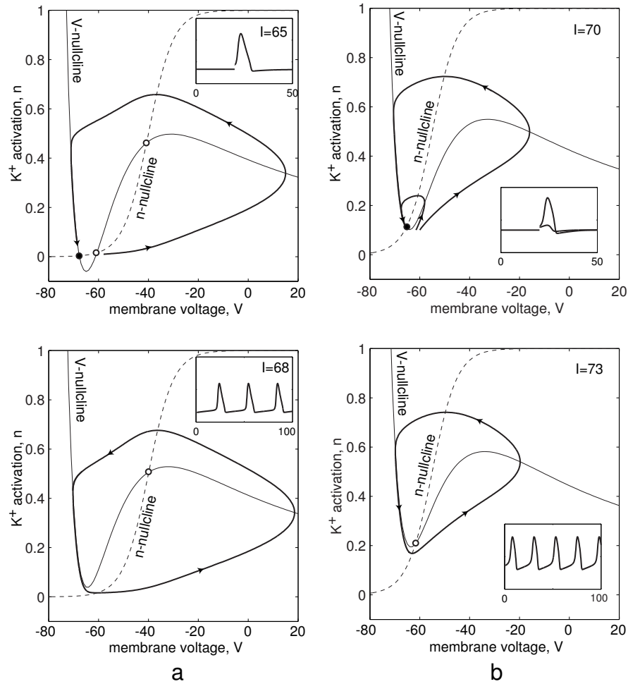
Figure 5.12: Possible intersections of nullclines in the I_K+I_{K_{ir}} -model. Parameters: E_K = -80 mV, g_{K_{ir}} = 20 , g_K = 2 . Instantaneous I_{K_{ir}} with V_{1/2} = -80 mV and k = -12 . Slower I_K with k = 5 , \tau(V) = 5 ms, and V_{1/2} = -40 mV (in a) or V_{1/2} = -55 mV (in b).
