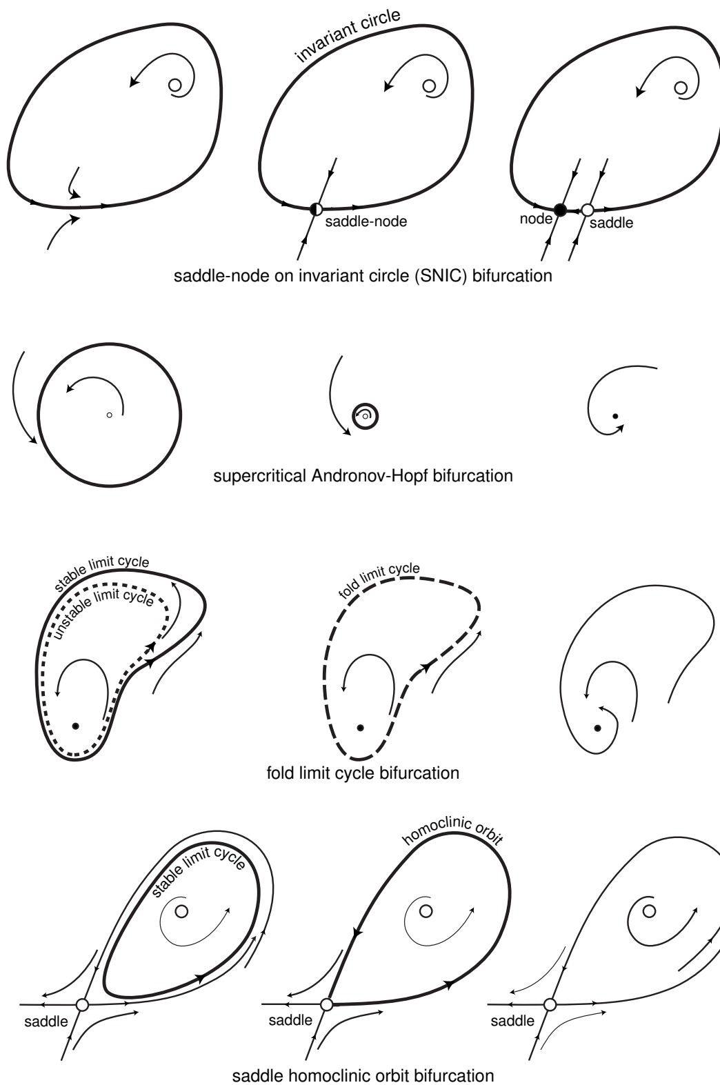
Figure 6.49: Summary of all co-dimension-1 bifurcations of a stable limit cycle (tonic spiking state) on a plane.
