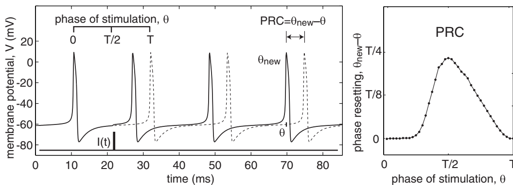
Figure 10.4: Phase response of the I_{Na} + I_K -model with parameters as in Fig. 4.1a and I = 4.7 . Dashed voltage trace is the free-running trajectory.
