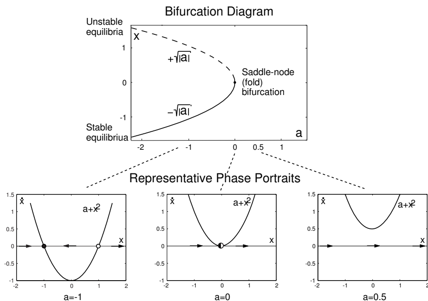
Figure 54: Saddle-node (fold) bifurcation diagram and representative phase portraits of the system \dot{x} = a + x^2 (see Chap. 3, Ex. 6).
