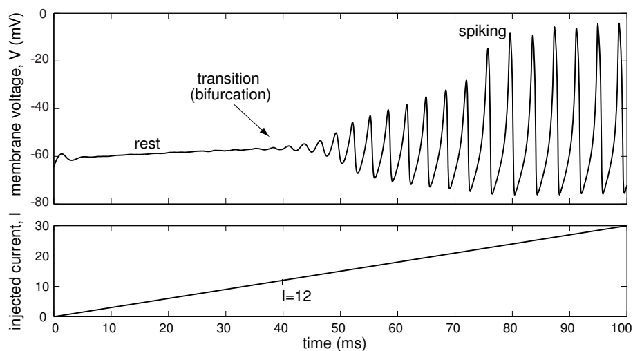
Figure 4.33: Transition from rest state to repetitive spiking in the I_{Na,p} + I_K -model with ramp injected current I ; see also Fig. 4.34 (small-amplitude noise is added to the model to mask the slow passage effect). Notice that the frequency of spiking is relatively constant for a wide range of injected current.
