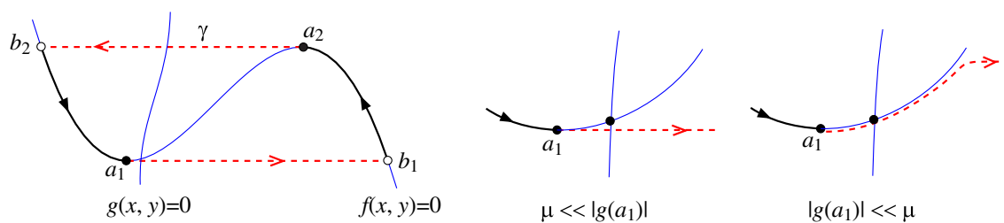
Figure 10.46: Left: Relaxation oscillator in the limit \mu = 0 near the onset of oscillation. Middle and right: A magnification of a neighborhood of the jump point a_1 for various g(a_1) and \mu . Canard (French duck) solutions can appear when g(a_1) \ll \mu .
