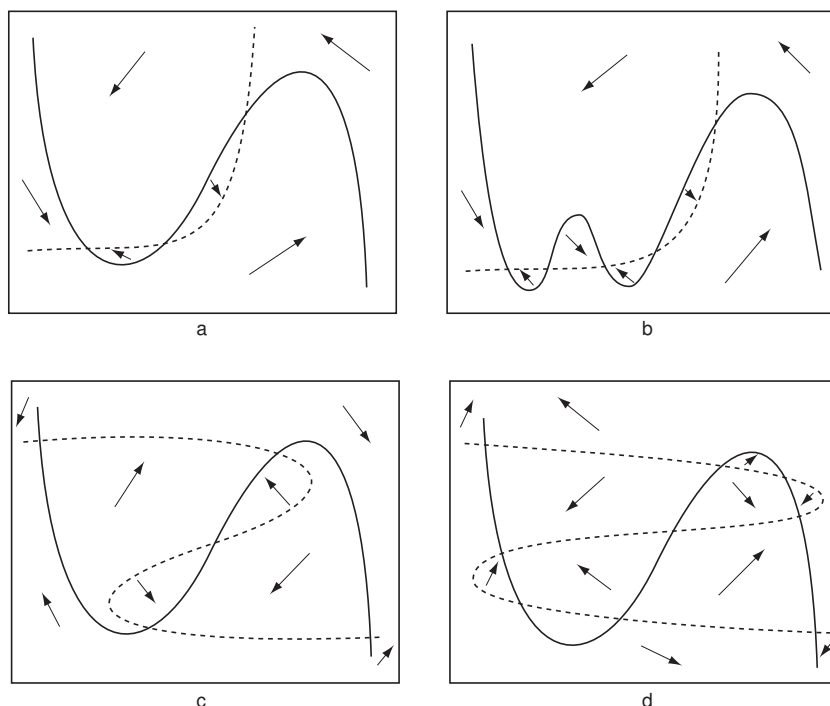
Figure 68: Approximate directions of the vector in each region between the nullclines.
