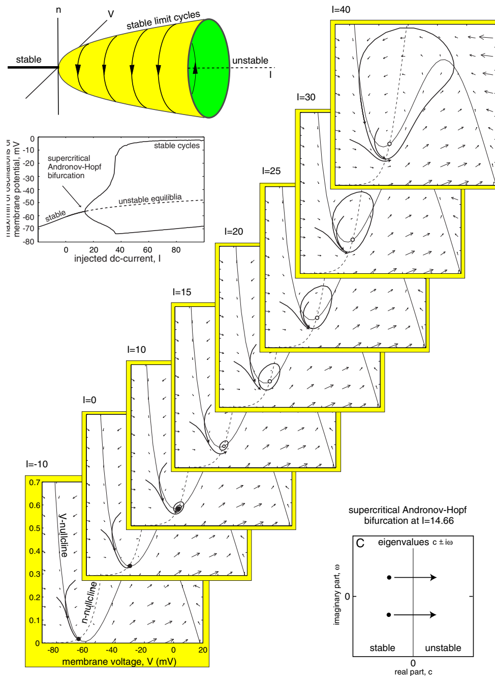
Figure 6.11: Supercritical Andronov-Hopf bifurcation in the I_{Na,p} + I_K -model with low-threshold K^+ current: As a bifurcation parameter I increases, an equilibrium loses stability and gives birth to a stable limit cycle with growing amplitude. Parameters as in Fig. 4.1b.
