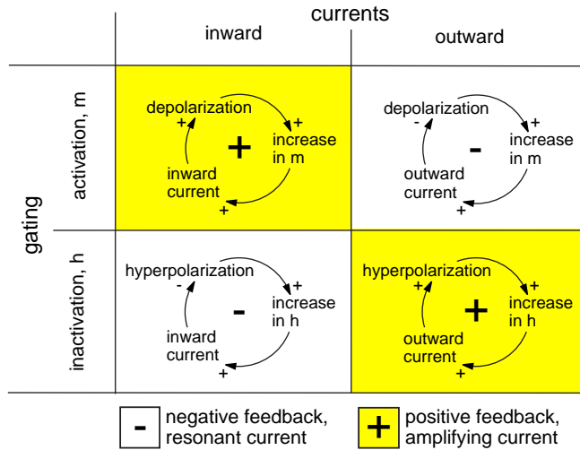
Figure 3.4: Feedback loops between voltage and gating variables in the four models presented above.
