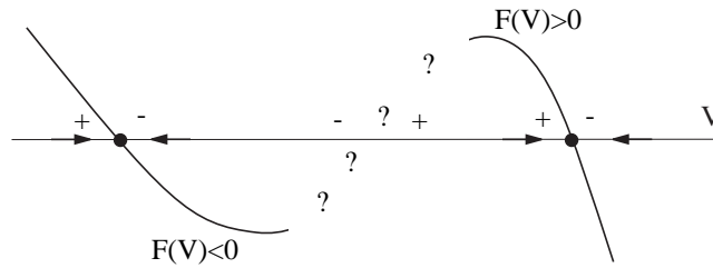
Figure 3.10: Two stable equilibrium points must be separated by at least one unstable equilibrium point because F(V) has to change the sign from “-” to “+”.
