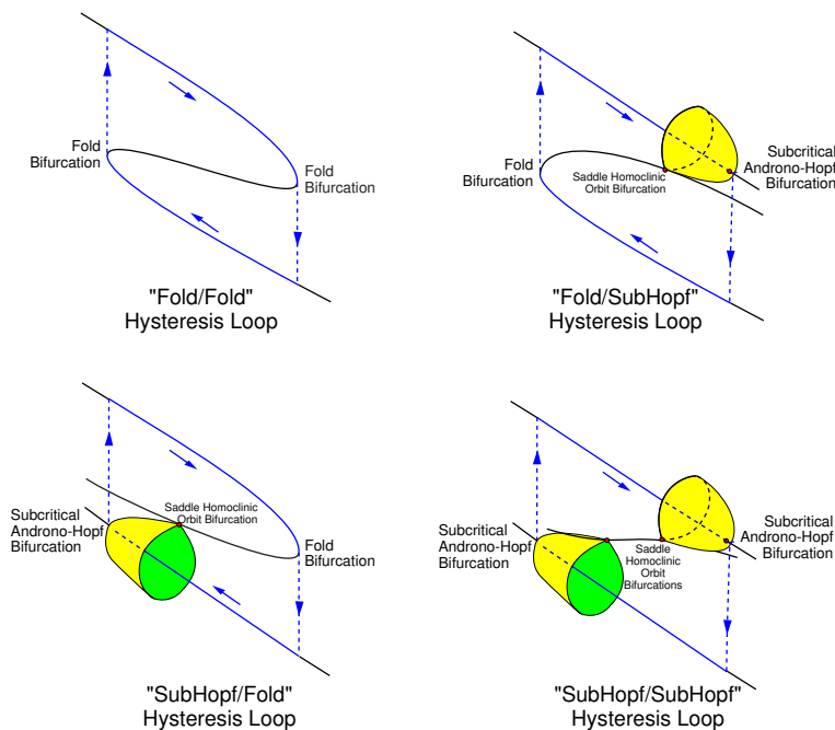
Figure 98: Classification of point-point co-dimension-1 hysteresis loops.
