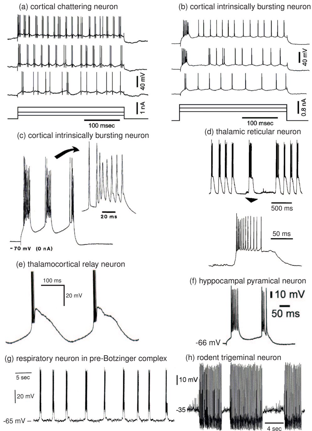
Figure 9.1: Examples of intrinsic bursters. (a) and (b) - cat primary visual cortical neurons (modified from Nowak et al. 2003). (c) cortical neuron in anesthetized cat (modified from Timofeev et al. 2000). (d) thalamic reticular (RE) neuron (modified from Steriade 2003). (e) Cat thalamocortical relay neuron (modified from McCormick and Pape 1990). (f) CA1 pyramidal neuron exhibiting grade II low-threshold bursting pattern (modified from Su et al. 2001). (g) respiratory neuron in the Pre-Botzinger complex (modified from Butera et al. 1999). (h) Trigeminal interneuron from rats brainstem (modified from Del Negro et al. 1998).
