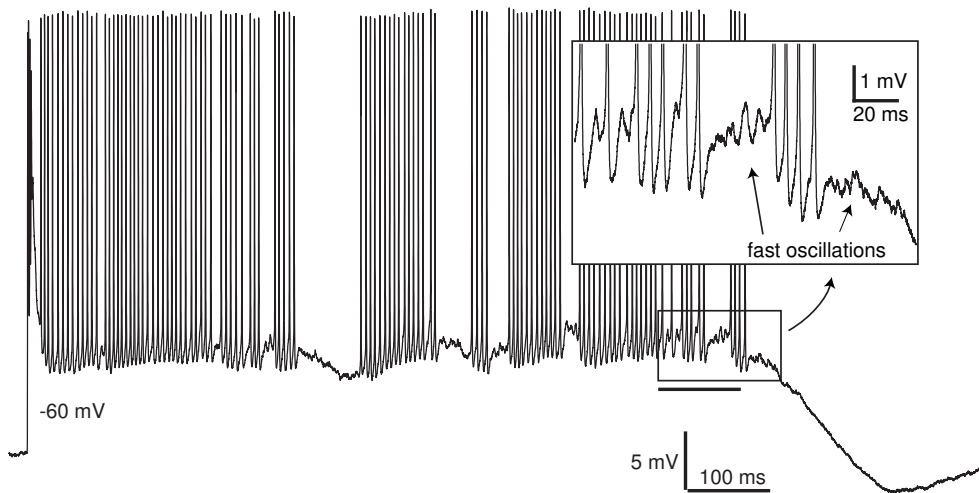
Figure 7.37: Fast subthreshold oscillations during complex spikes of cerebella Purkinje neuron of a guinea-pig (data was provided by Yonatan Loewenstein).
