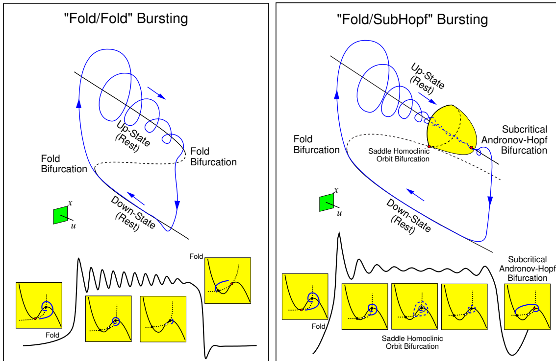
Figure 9.61: Two examples of point-point (not fast-slow) bursters (modified from Izhikevich 2000).
