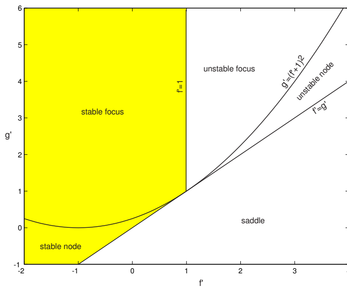
Figure 76: Stability diagram of the Hindmarsh–Rose spiking neuron model; see Ex. 7.
