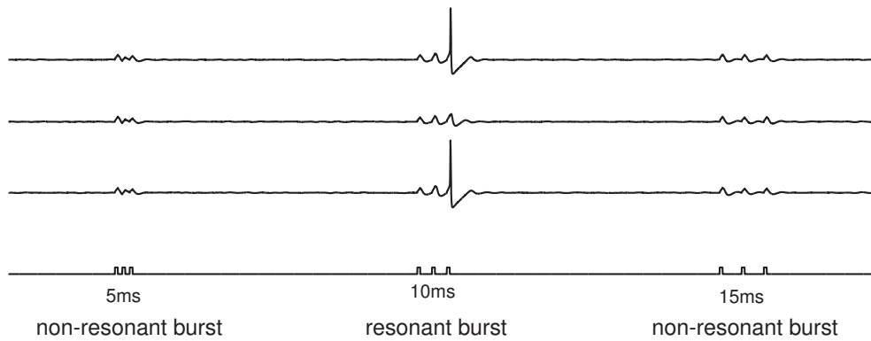
Figure 7.20: Experimental observations of selective response to a resonant (10 ms interspike period) burst in mesencephalic V neurons in brainstem having subthreshold membrane oscillations with natural period around 9 ms; see also Fig. 7.18. Three consecutive voltage traces are shown to demonstrate some variability of the result. Modified from Izhikevich et al. (2003).
