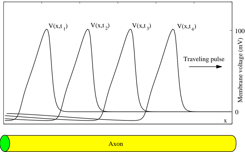
Figure 2.18: Traveling pulse solution of the Hodgkin-Huxley cable equation at four successive moments.
