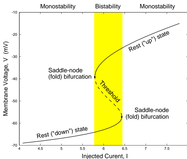
Figure 58: Bifurcation diagram of the I_{Kir} -model (3.11).
