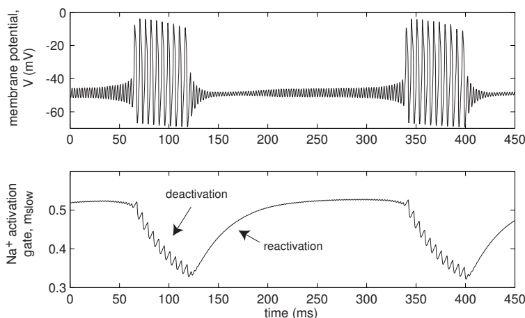
Figure 92: Bursting in the I_{Na,p} + I_K + I_{Na,slow} -model. See Ex. 11.
