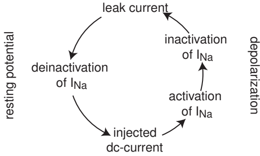
Figure 5.5: Mechanism of generation of sustained oscillations in the I_{Na,t} -model.
