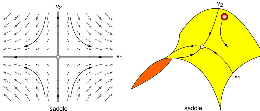
Figure 4.17: Saddle equilibrium occurs when two real eigenvalues have opposite signs, e.g., \lambda_1 = +1 and \lambda_2 = -1 . Most trajectories diverge from the equilibrium along the eigenvector corresponding to the positive eigenvalue (in this case v_1 ).
