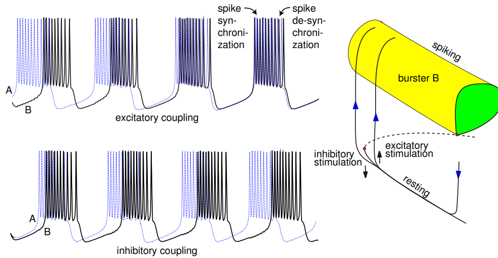
Figure 9.51: Burst synchronization and de-synchronization of two coupled “fold/homoclinic” bursters (modified from Izhikevich 2000).
