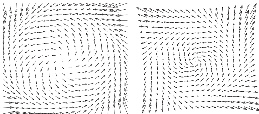
Figure 4.43: Use pencil to draw phase portrait as in Fig. 4.39.
