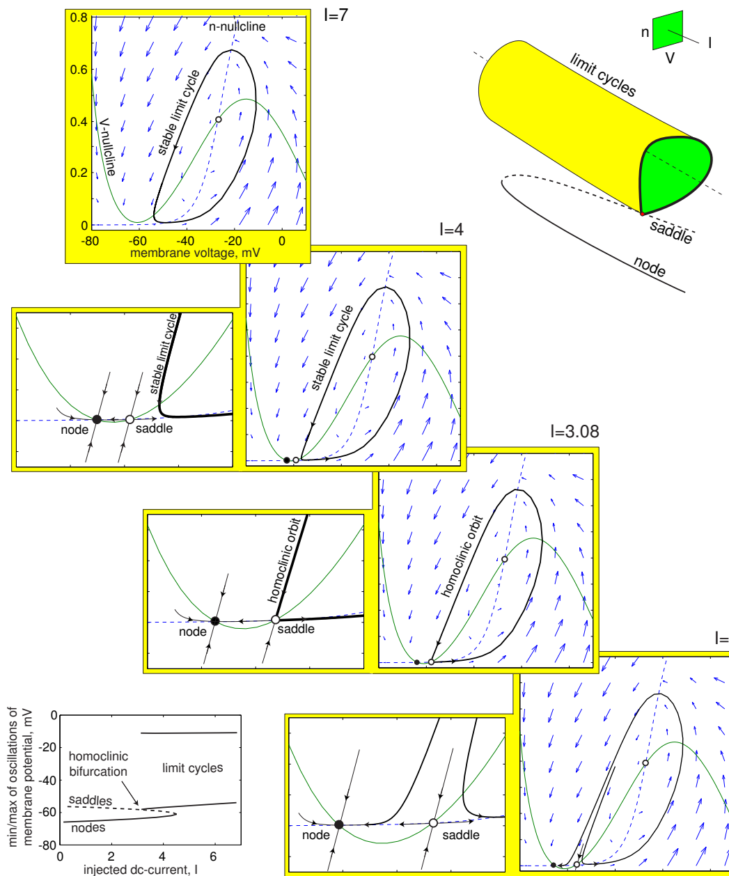
Figure 6.28: Saddle homoclinic orbit bifurcation in the I_{Na,p}+I_K -model with parameters as in Fig. 4.1a and fast K^+ current ( \tau(V) = 0.16 ). As the bifurcation parameter I decreases, the stable limit cycle becomes a homoclinic orbit to a saddle.
