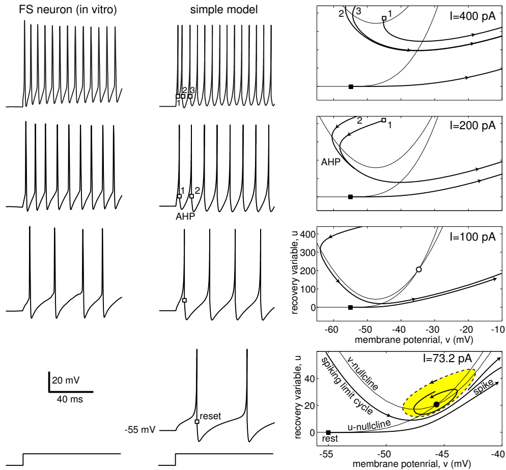
Figure 8.22: Comparison of in vitro recordings of a fast spiking (FS) interneuron of layer 5 rat's visual cortex with simulations of the simple model 20\dot{v} = (v + 55)(v + 40) - u + I , \dot{u} = 0.2\{U(v) - u\} , if v \geq 25 , then v \leftarrow -45 mV. Slow nonlinear nullcline U(v) = 0 when v < v_b and U(v) = 0.025(v - v_b)^3 when v \geq v_b with v_b = -55 mV. Shaded area denotes the attraction domain of the resting state.
