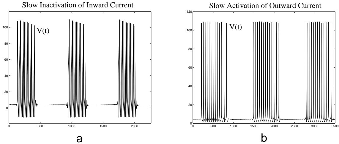
Figure 9.9: Hodgkin-Huxley (1952) model with three gating variables is minimal for bursting (modified from Fig.1.10 in Izhikevich 2001).
