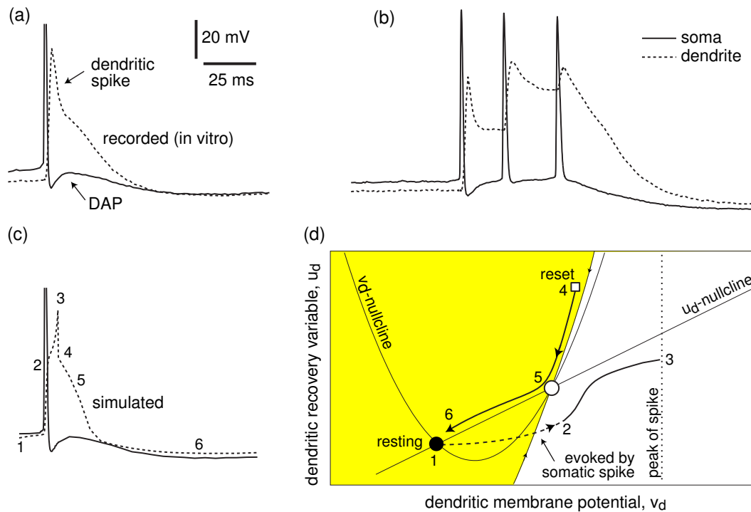
Figure 8.16: Somatic and dendritic spike (a) and burst (b) in an IB neuron. The dendritic spike in (a) is simulated in (c) using the simple model described in Fig. 8.16. Phase portrait (d) describes the geometry of dendritic spike-generation mechanism. (Recordings are from layer 5 of somatosensory cortex of a 4 week old rat at 35C; dendritic electrode is 0.43mm from the soma; data was kindly provided by Greg Stuart and Maarten Kole).
