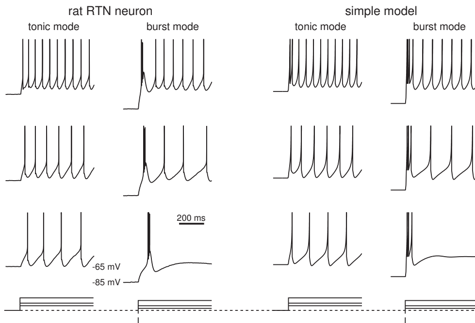
Figure 8.27: Comparison of in vitro recordings of a reticular thalamic nucleus (RTN) neuron of a rat with simulations of the simple model 40\dot{v} = 0.25(v + 65)(v + 45) - u + I , \dot{u} = 0.015\{b(v + 65) - u\} , b = 10 if v \leq -65 and b = 2 otherwise. When v \geq 0 (spike cutoff), then v \leftarrow -55 , u \leftarrow u + 50 . Injected current pulses are 50, 70, 110 pA. In burst mode, the cell was hyperpolarized to -80 mV prior to injecting a depolarizing pulse of current (data provided S.H. Lee and C.L. Cox).
