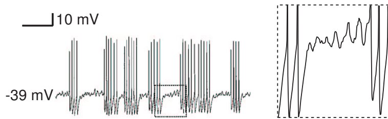
Figure 9.37: Putative “subHopf/fold cycle” bursting in rodent trigeminal neurons (modified from Del Negro et al. 1998).
