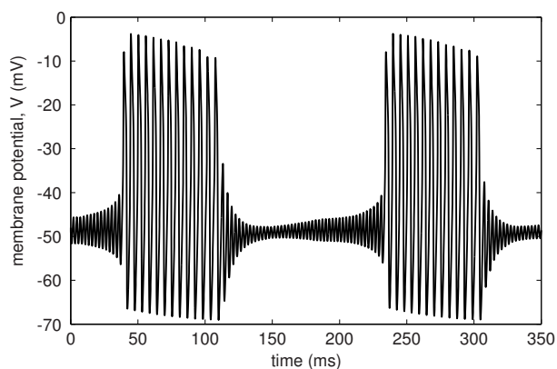
Figure 9.58: Bursting in the I_{Na,p}+I_K+I_{Na,slow} -model; see Ex. 11.
