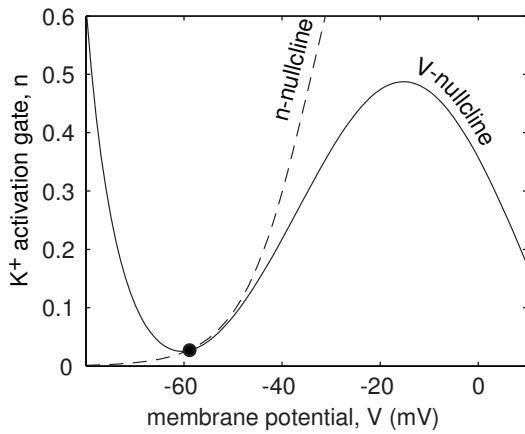
Figure 7.39: Bogdanov-Takens bifurcation in the I_{Na} + I_K -model (4.1, 4.2). Parameters as in Fig. 4.1a, except n_\infty(V) has k = 7 mV and V_{1/2} = -31.64 mV, E_{leak} = -79.42 and I = 5 . Integrator: V_{1/2} = -31 mV and I = 4.3 . Resonator: V_{1/2} = -34 mV and I = 7 .
