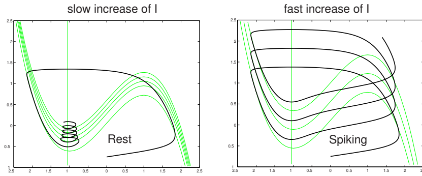
Figure 93: The system has a unique attractor – equilibrium, yet it can exhibit repetitive spiking activity when the N-shaped nullcline is moved up not very slow.
