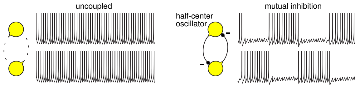
Figure 9.10: Central pattern generation by mutually inhibitory oscillators.
