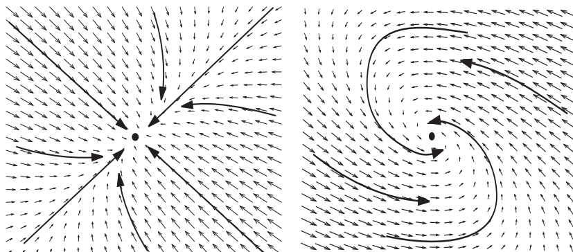
Figure 70: Left: Stable node. Right: Stable focus.
