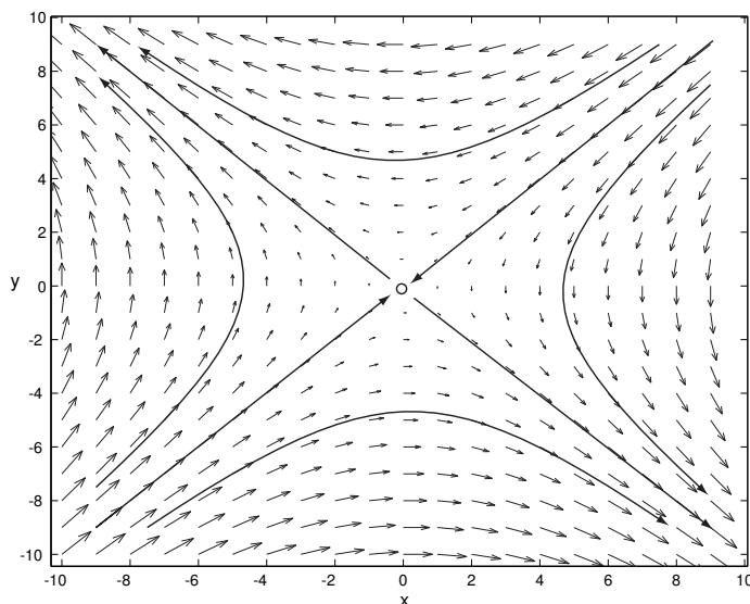
Figure 4.6: Representative trajectories of two-dimensional system (4.3,4.4).
