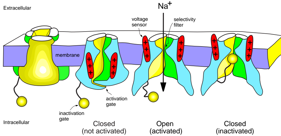
Figure 2.8: Structure of voltage-gated ion channels. Voltage sensors open activation gate and allow selective ions to flow through the channel according to their electrochemical gradients. The inactivation gate blocks the channel (modified from Armstrong and Hille 1998).
