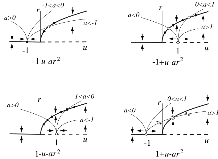
Figure 88: Intersections of nullclines r' = 0 (bold curve) and u' = 0 (thin curve) for various a and \pm 1 \pm u - ar^2 ; see Ex. 8.
