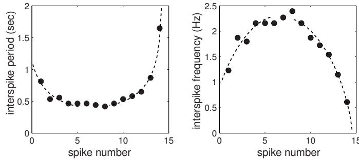
Figure 9.32: The interspike period in the “circle/circle” bursting in Fig. 9.31 resembles a parabola, which motivates the name “parabolic bursting” used in earlier studies.
