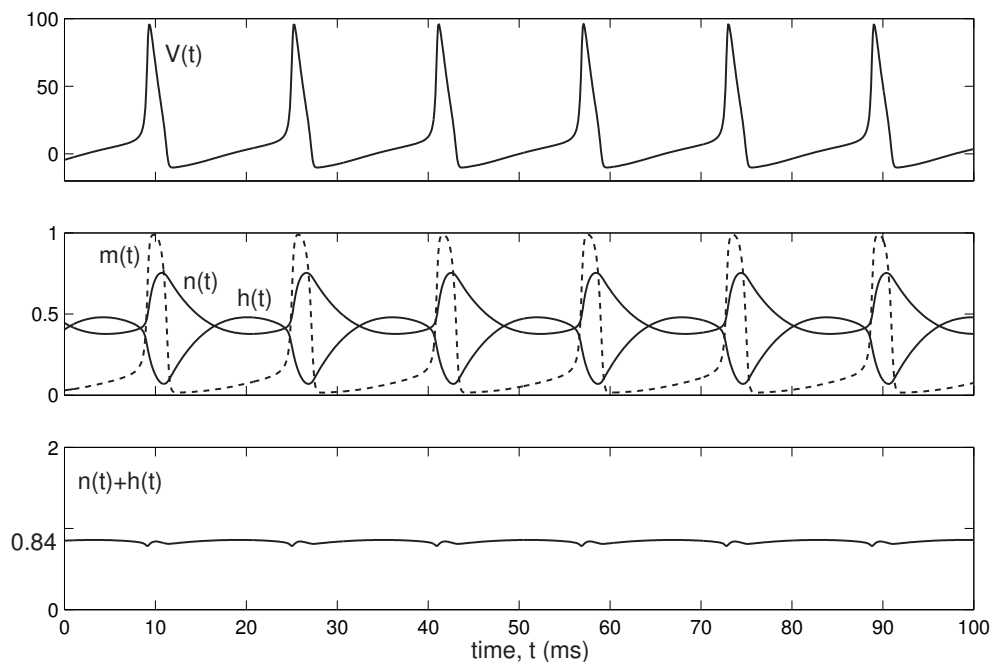
Figure 5.18: The sum n(t) + h(t) \approx 0.84 in the Hodgkin-Huxley model. Parameters as in Chap. 2 and I = 8 .
