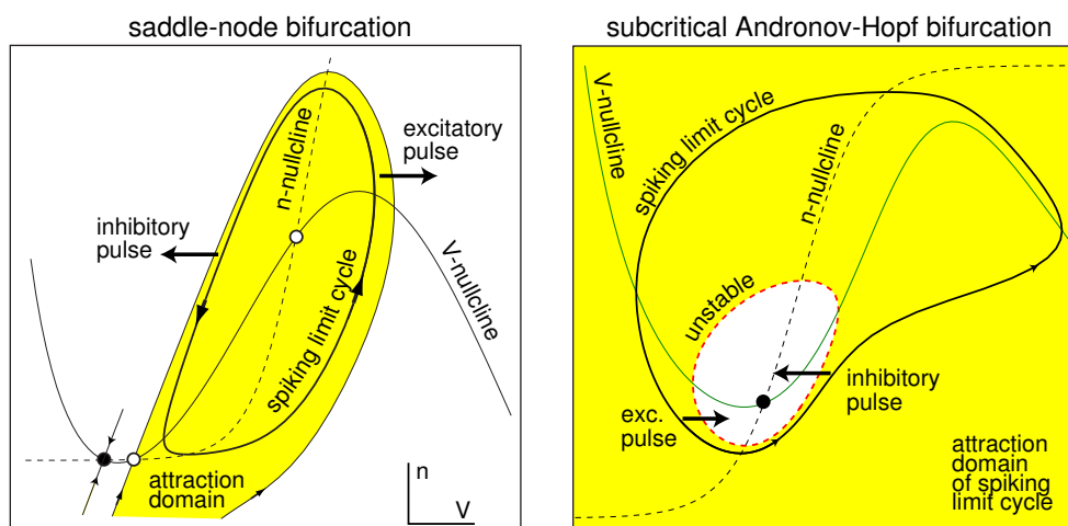
Figure 7.11: Coexistence of stable equilibrium and spiking limit cycle attractor in the I_{Na,p} + I_K -model. Left : The rest state is about to disappear via saddle-node bifurcation. Right : The rest state is about to lose stability via subcritical Andronov-Hopf bifurcation. Right (left) arrows denote the location and the direction of excitatory (inhibitory) pulse that switches spiking behavior to resting.
