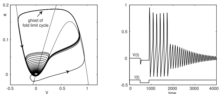
Figure 86: Rebound bursting in the FitzHugh-Nagumo oscillator; see Ex. 4.
