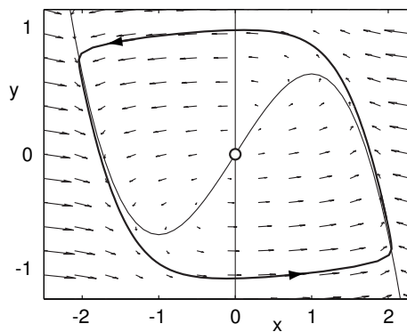
Figure 74: Nullclines and phase portrait of the van der Pol oscillator ( b = 0.1 ).
