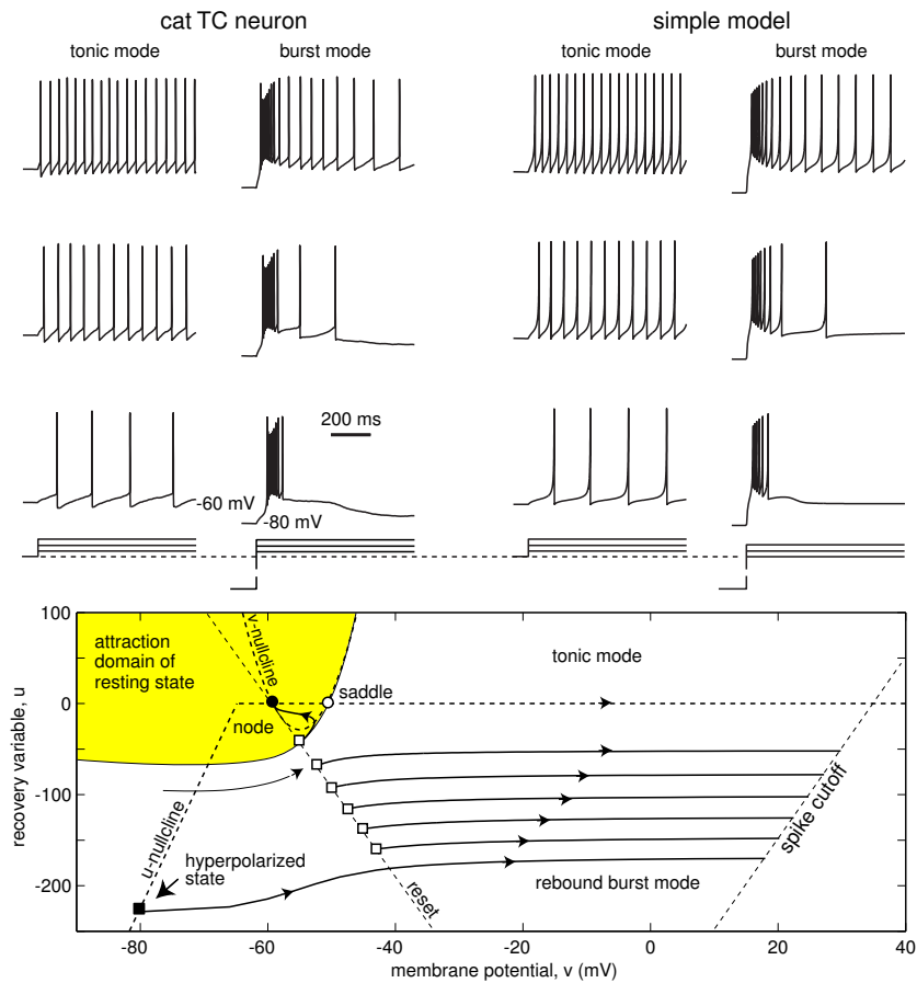
Figure 8.26: Comparison of in vitro recordings of a thalamocortical (TC) cell of cat dorsal lateral geniculate nucleus with simulations of the simple model 200\dot{v} = 1.6(v + 60)(v + 50) - u + I , \dot{u} = 0.01\{b(v + 65) - u\} , b = 15 if v \leq -65 and b = 0 otherwise. When v \geq 35 + 0.1u , then v \leftarrow -60 - 0.1u , u \leftarrow u + 10 . Injected current pulses are in 50 pA increments. In burst mode, the cell was hyperpolarized to -80 mV prior to injecting a depolarizing pulse of current (data provided by C. L. Cox and S. M. Sherman)
