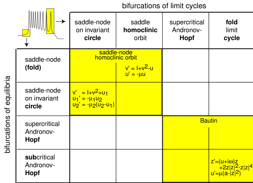
Figure 9.62: Some canonical models of fast-slow bursters; see Ex. 27.
