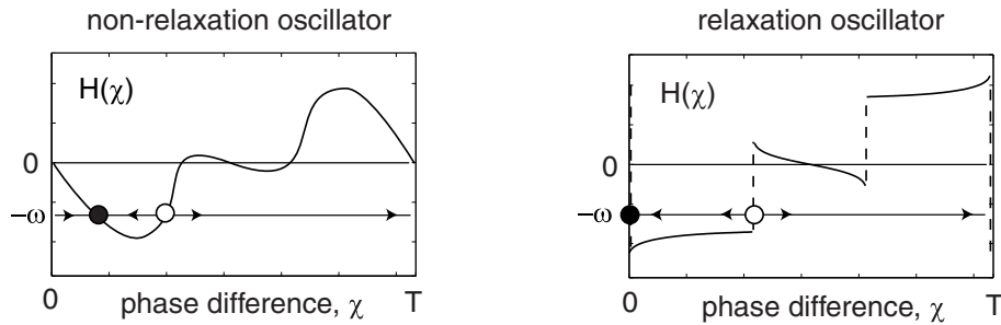
Figure 10.31: Functions H(\chi) for weakly coupled oscillators of non-relaxation (smooth) and relaxation type. Frequency mismatch \omega creates a phase difference in the smooth case, but not in the relaxation case.
