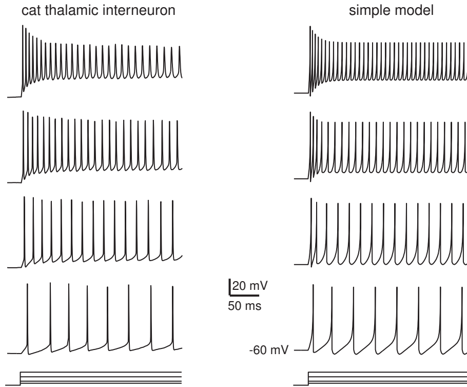
Figure 8.28: Comparison of in vitro recordings of dorsal lateral geniculate nucleus interneuron of a cat with simulations of the simple model 20\dot{v} = 0.5(v + 60)(v + 50) - u + I , \dot{u} = 0.05\{7(v + 60) - u\} . When v \geq 20 - 0.08u (spike cutoff), then v \leftarrow -65 + 0.08u , u \leftarrow u + 50 . Injected current pulses are 50, 100, 200, 300 pA (data provided by C. L. Cox and S. M. Sherman)
