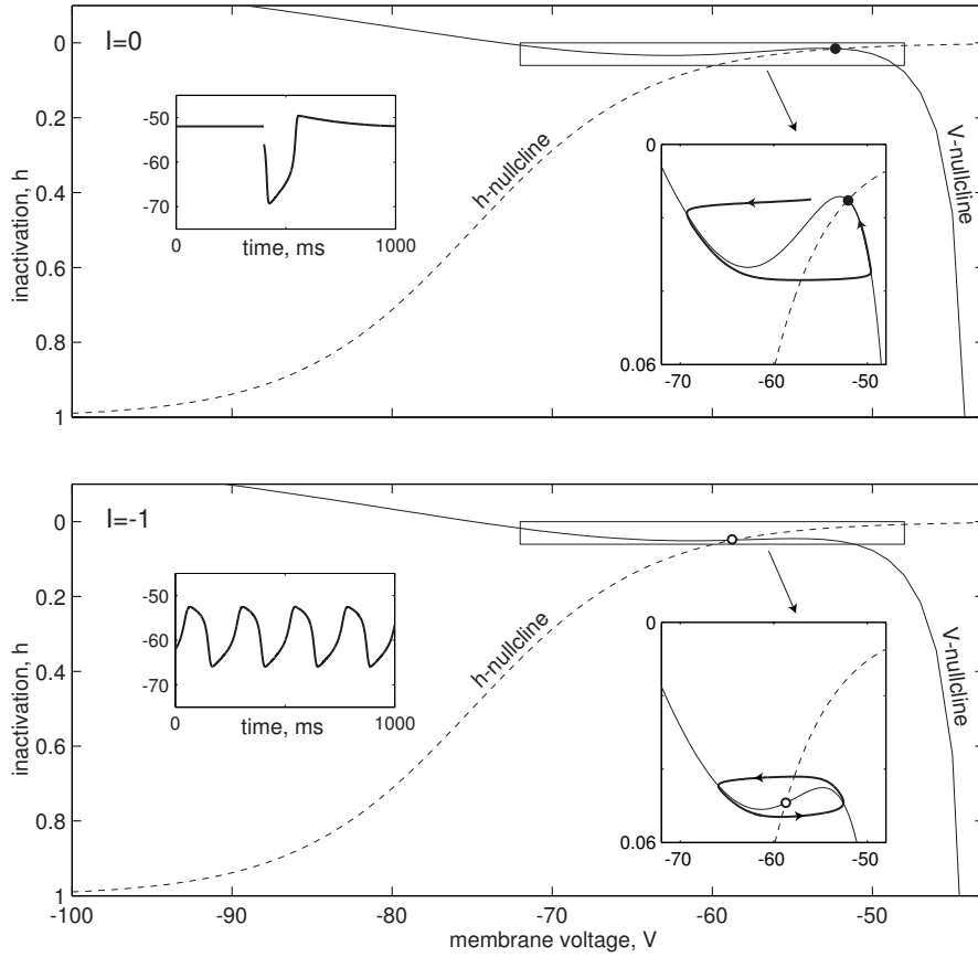
Figure 5.8: Rest and sustained subthreshold oscillations in the I_{Na,p}+I_h -model. Parameters for currents as in thalamocortical neurons, E_{Na} = 20 mV, E_h = -43 mV, E_L = -80 mV, g_L = 1.3 , g_{Na} = 0.9 , and g_h = 3 .
