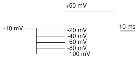
Figure 2.24: Multiple voltage steps are often needed to determine time constants of inactivation; see Ex. 7.
