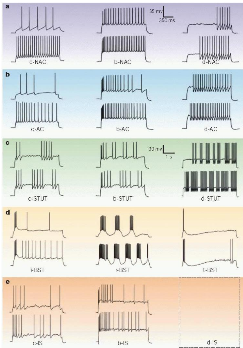
Figure 8.24: An alternative classification of neocortical inhibitory interneurons (modified from Markram et al. 2004). Five major classes: non-accommodating (NAC), accommodating (AC), stuttering (STUT), bursting (BST), and irregular spiking (IS). Most classes contain subclasses: delay (d), classic (c), and burst (b). For bursting interneurons, the three types are repetitive (r), initial (i), and transient (t). Subclass d-IS is not provided in the original picture by Markram et al. (2004).
