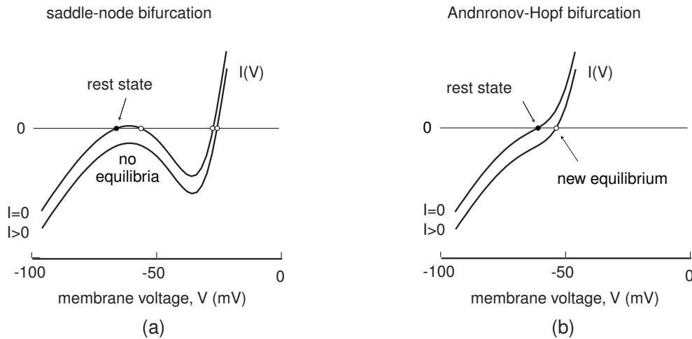
Figure 6.3: Steady-state I-V curves of the I_{Na,p} + I_K -model with high-threshold (left) or low-threshold (right) K^+ current (parameters as in Fig. 4.1).
