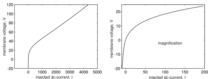
Figure 59: Dependence of the position of equilibrium in the Hodgkin-Huxley model on the injected dc-current; see Ex. 10.
