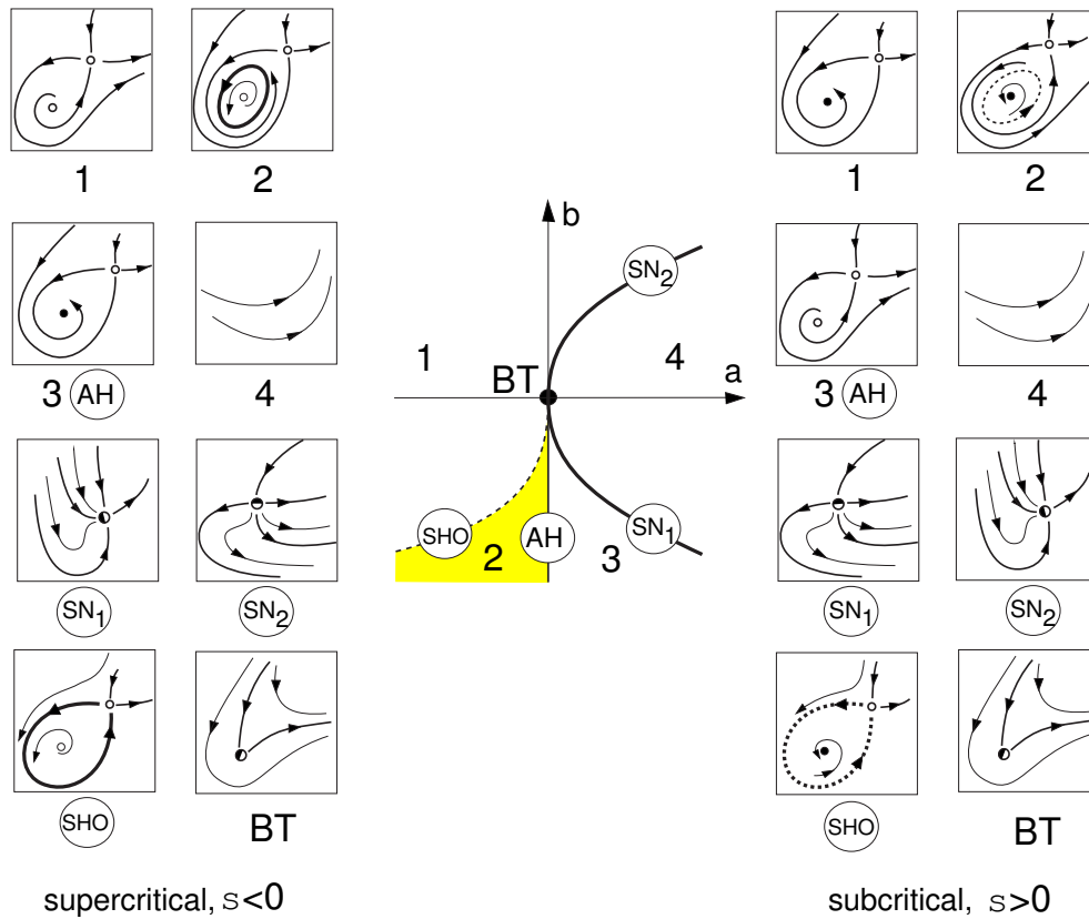
Figure 6.38: Bogdanov-Takens (BT) bifurcation diagram of the topological normal form (6.7). Abbreviations: AH - Andronov-Hopf bifurcation, SN - saddle-node bifurcation, SHO - saddle homoclinic orbit bifurcation.
