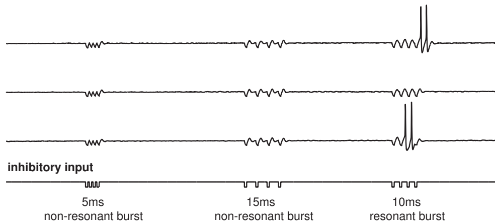
Figure 7.21: Experimental observations of selective response to inhibitory resonant burst in mesencephalic V neurons in brainstem having oscillatory potentials with the natural period around 9 ms. Modified from Izhikevich et al. (2003).
