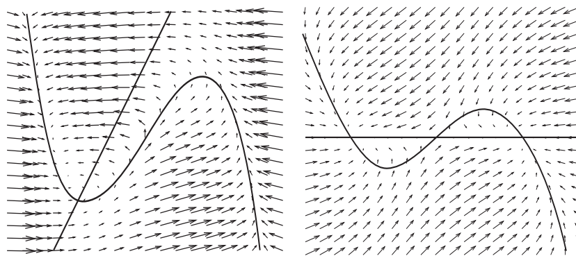
Figure 65: Nullclines of the vector field; see also Fig. 71.
