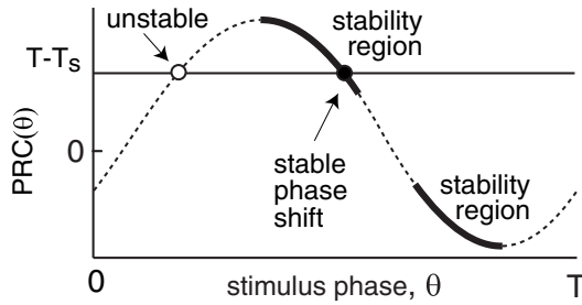
Figure 10.13: Fixed points of the Poincare phase map (10.1.5).
