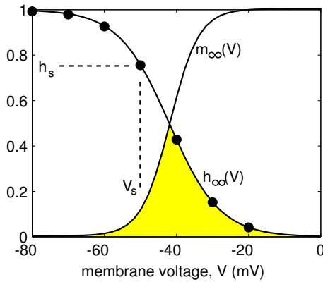
Figure 2.11: Steady-state activation function m_\infty(V) from Fig. 2.10, inactivation function h_\infty(V) , and values h_s from Fig. 2.12. Their overlap (shaded region) produces a noticeable persistent “window” current.
