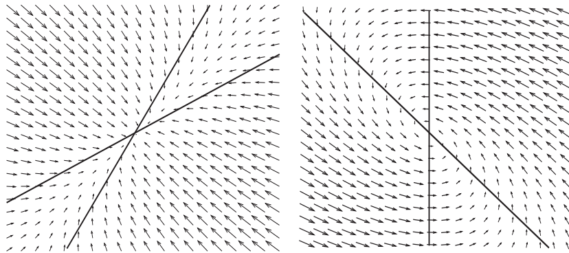
Figure 64: Nullclines of the vector field; see also Fig. 70.
