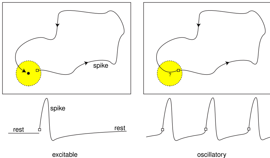
Figure 7.1: Left : An abstract definition of excitability. There is a spike trajectory that starts near a stable equilibrium and returns to it. Right : Excitable systems are near bifurcations. A modification of the vector field in the small shaded region can result in a periodic trajectory.
