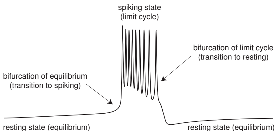
Figure 9.21: Two important bifurcations associated with fast-slow bursting.
